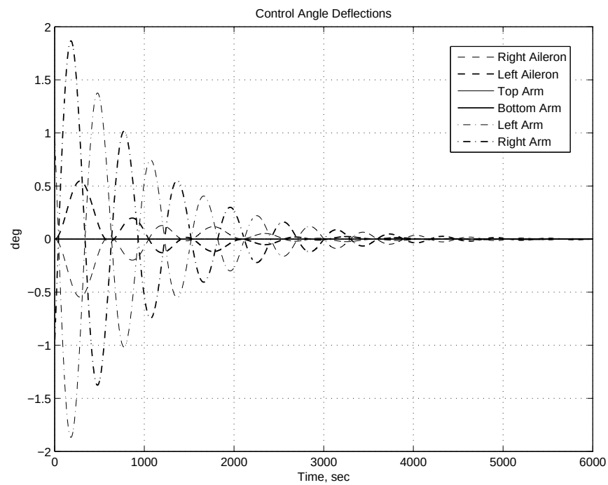
Figure E.28: Control angle deflections at 300km with yaw offset 10^\circ .
