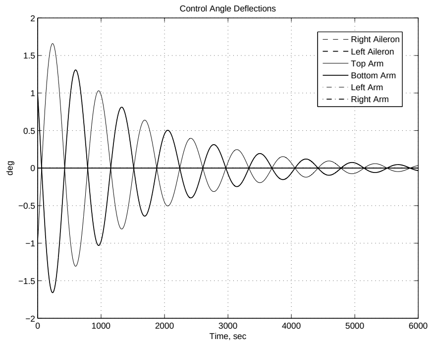
Figure E.24: Control angle deflections 300 km with pitch offset 10^\circ .
