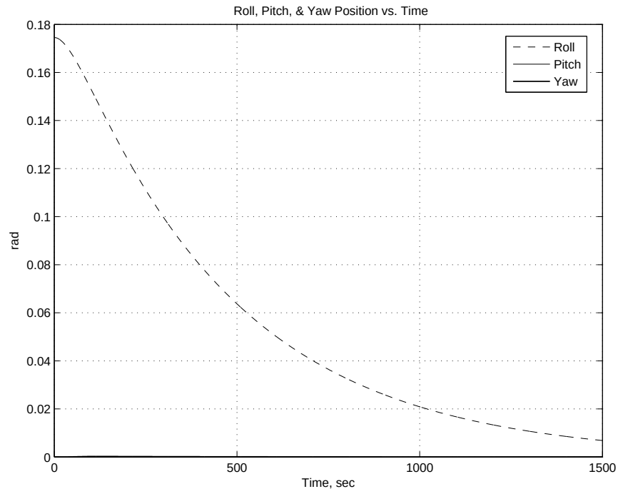
Figure E.1: Angular displacement at 200km with roll offset 10^\circ .
