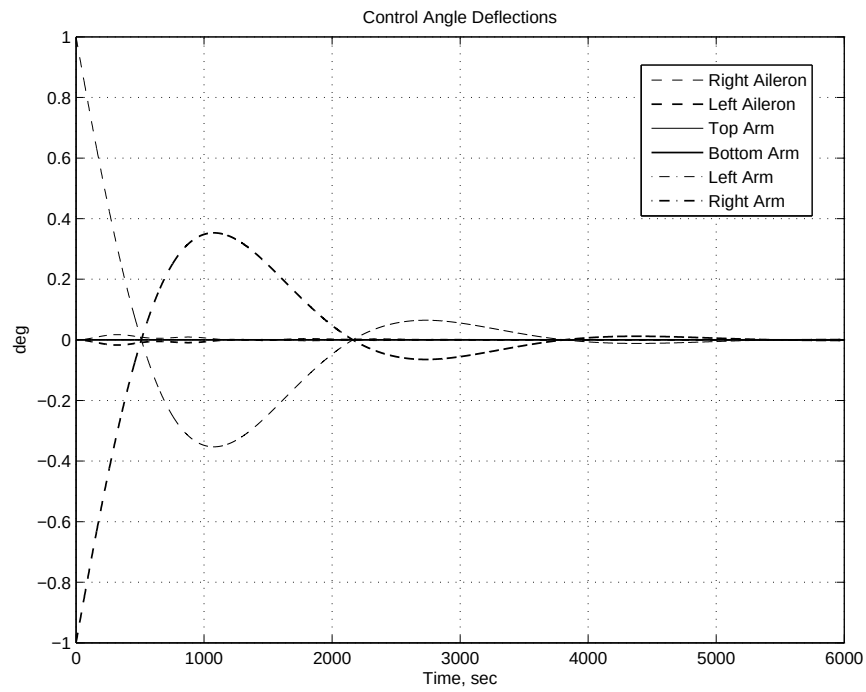
Figure E.20: Control angle deflections 300 km with roll offset 10^\circ .
