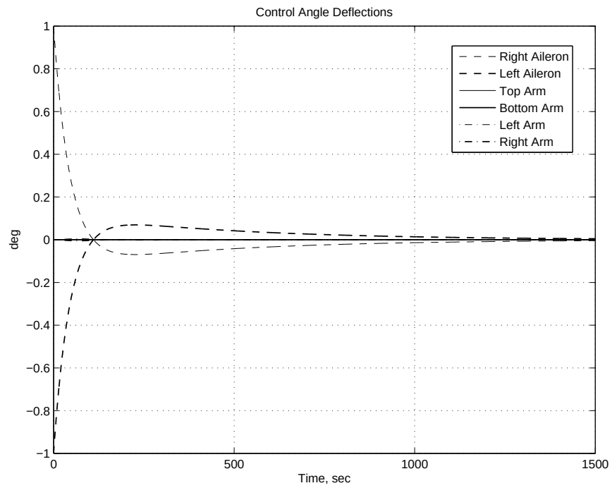
Figure E.4: Control angle deflections 200 km with roll offset 10^\circ .
