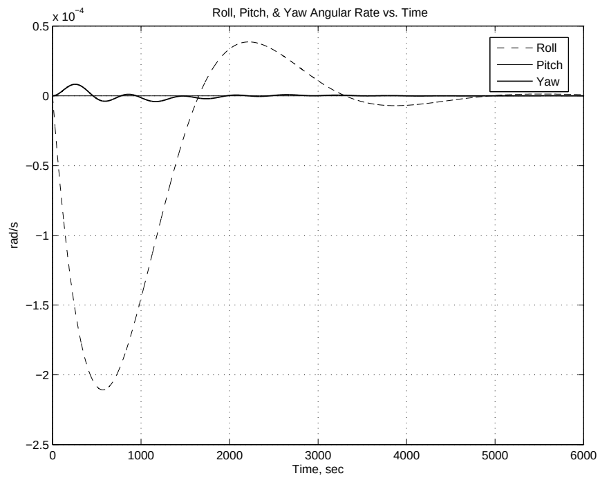
Figure E.18: Angular rate at 300km with roll offset 10^\circ .
