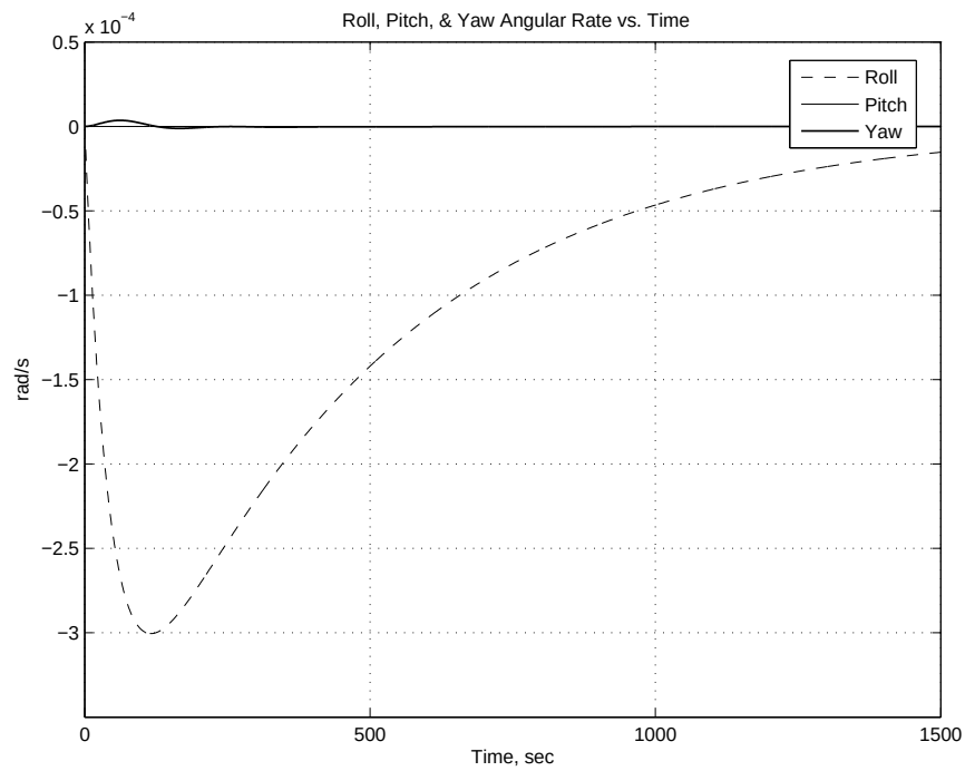
Figure E.2: Angular rate at 200km with roll offset 10^\circ .
