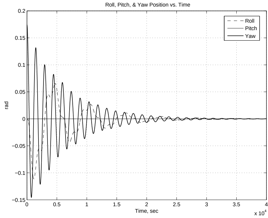
Figure E.41: Angular displacement at 400km with yaw offset 10^\circ .
