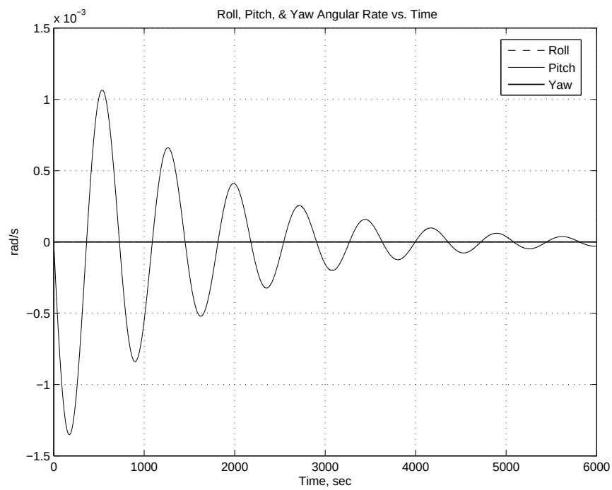
Figure E.22: Angular rate at 300km with pitch offset 10^\circ .
