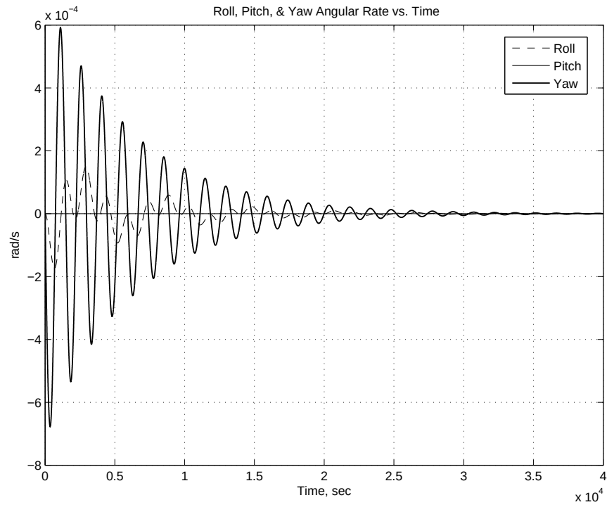
Figure E.42: Angular rate at 400km with yaw offset 10^\circ .
