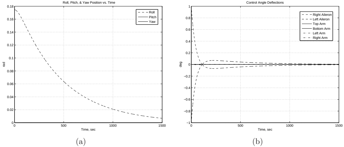
Figure 5.1: (a) Angular displacement with roll offset 10^\circ . (b) Control angles with roll 10^\circ .
