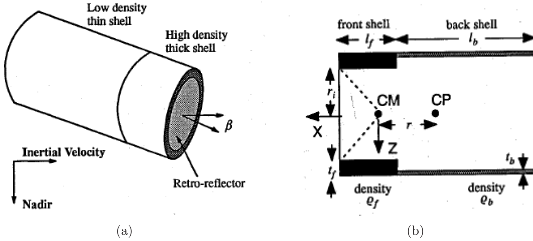
Figure 2.3: (a) Shuttle Hitchhiker schematic (b) Cross section view
