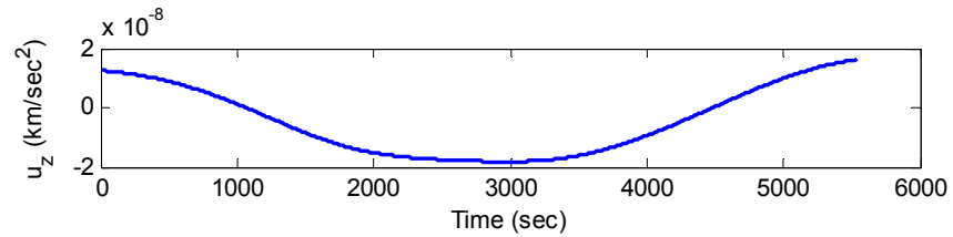
Figure 29. Case Study #4, 10-km Formation Radius
