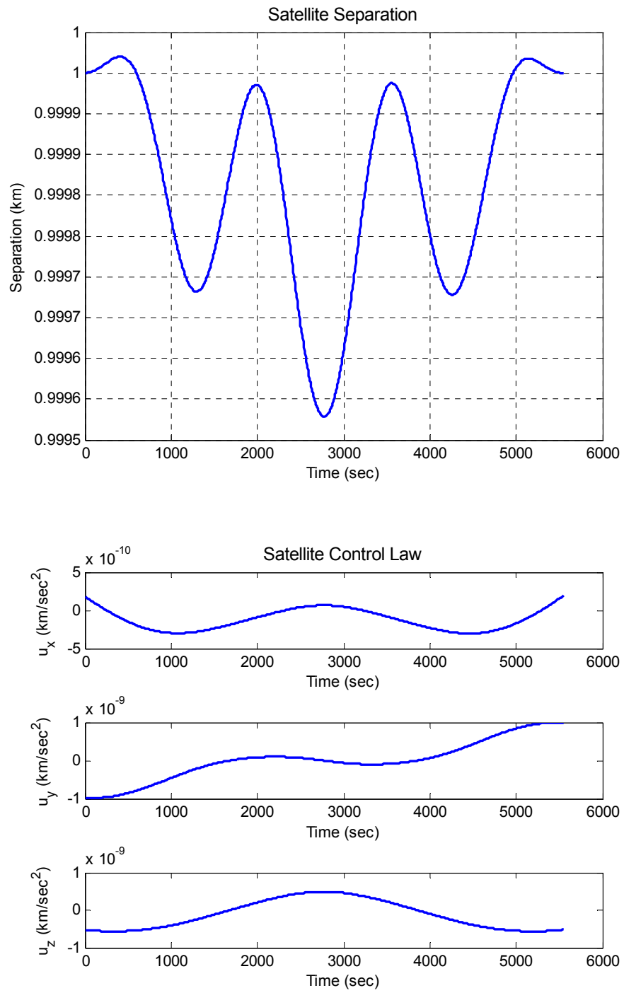
Figure 16. Case Study #1, 90-deg Inclination
