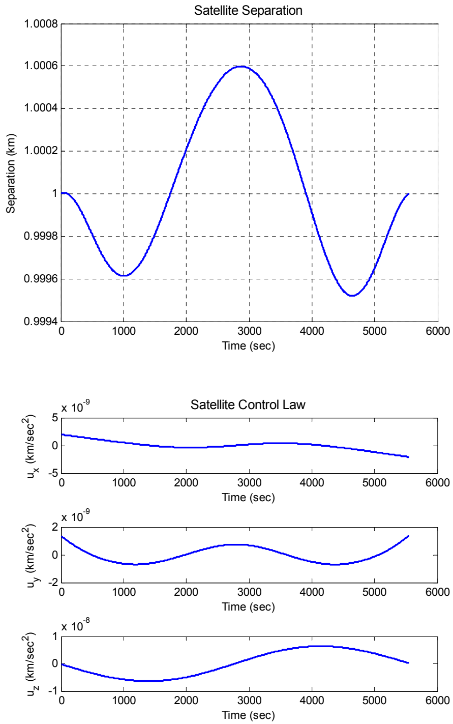
Figure 18. Case Study #2, 0-deg Inclination
