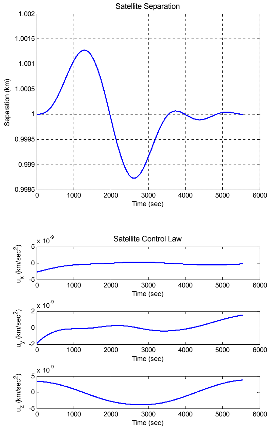
Figure 13. Case Study #1, 30-deg Inclination
