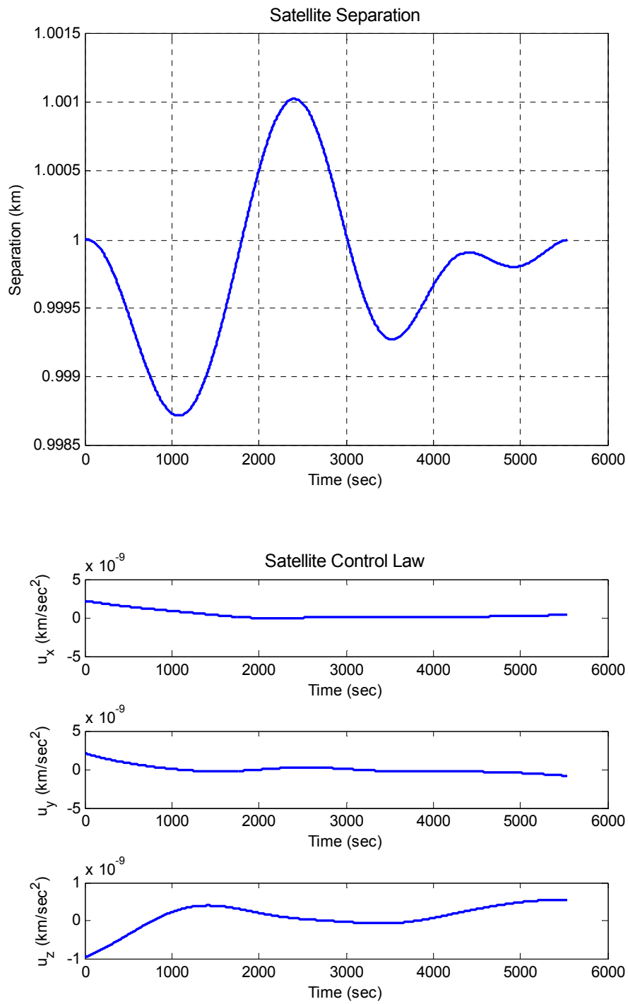
Figure 20. Case Study #2, 45-deg Inclination
