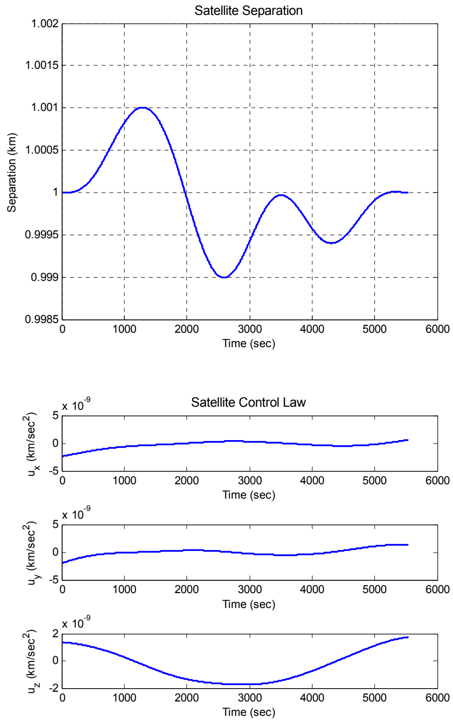
Figure 14. Case Study #1, 45-deg Inclination
