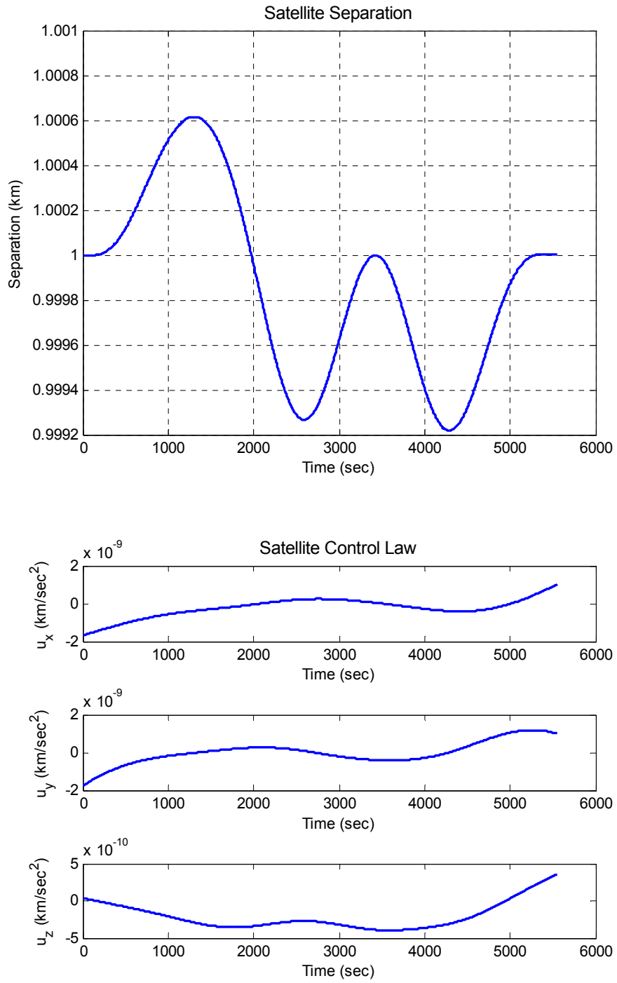
Figure 15. Case Study #1, 60-deg Inclination
