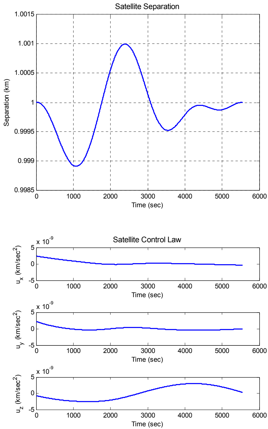
Figure 19. Case Study #2, 30-deg Inclination
