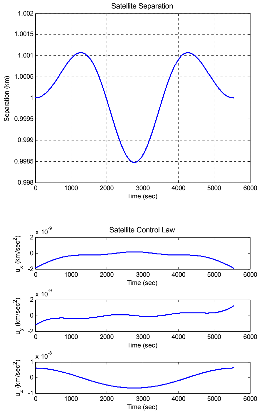
Figure 12. Case Study #1, 0-deg Inclination
