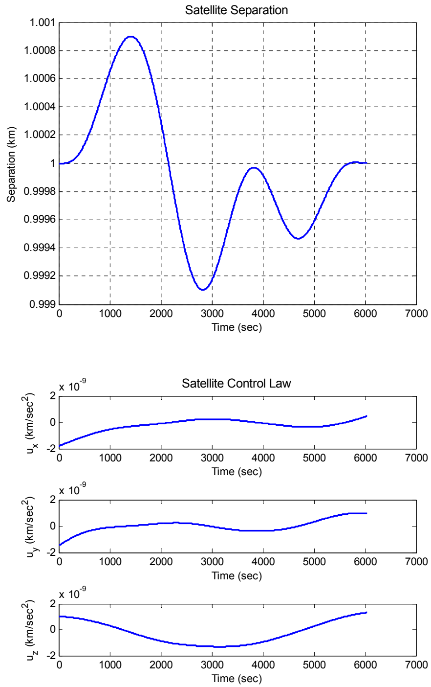
Figure 25. Case Study #3, 45-deg Inclination
