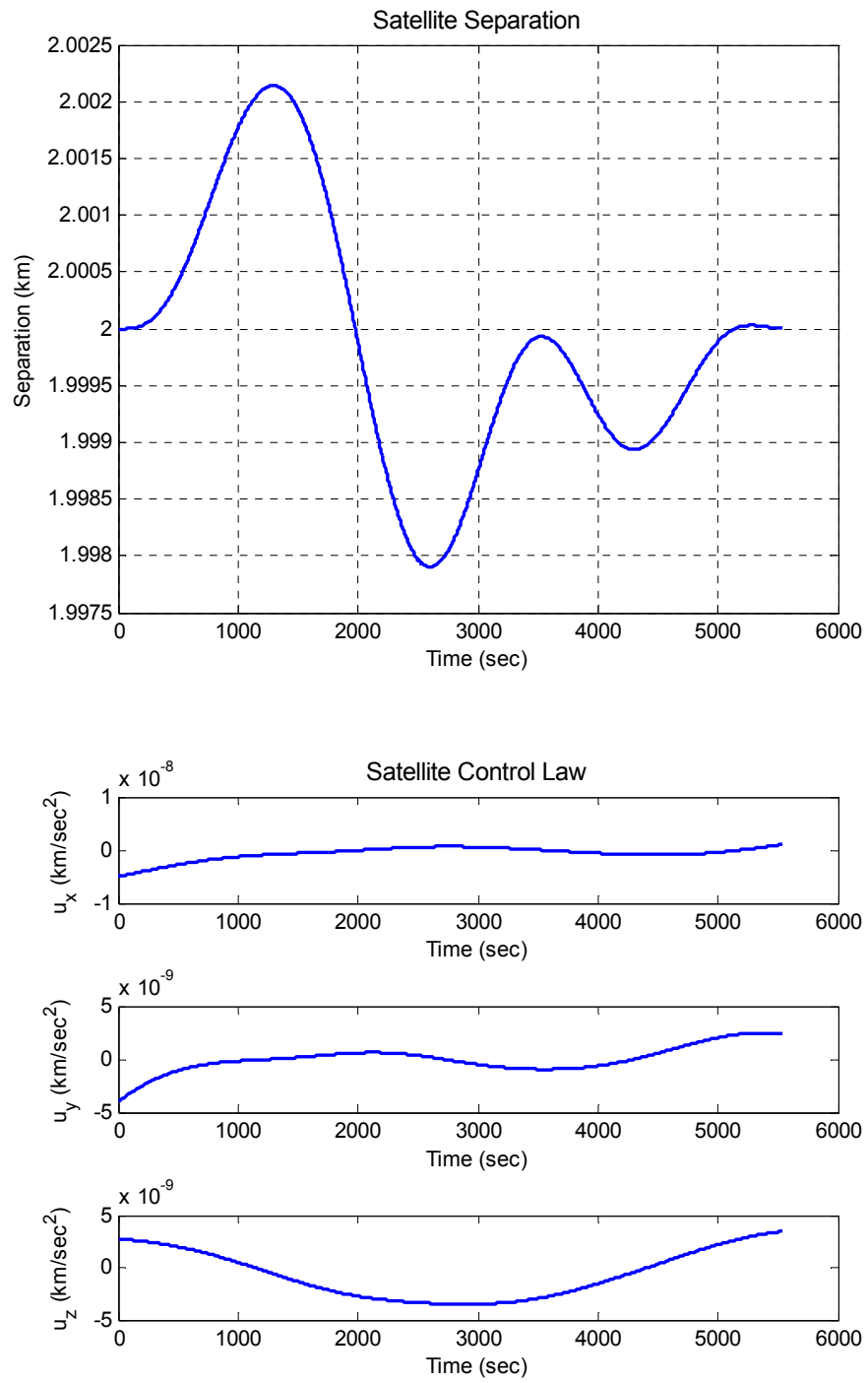
Figure 28. Case Study #4, 2-km Formation Radius
