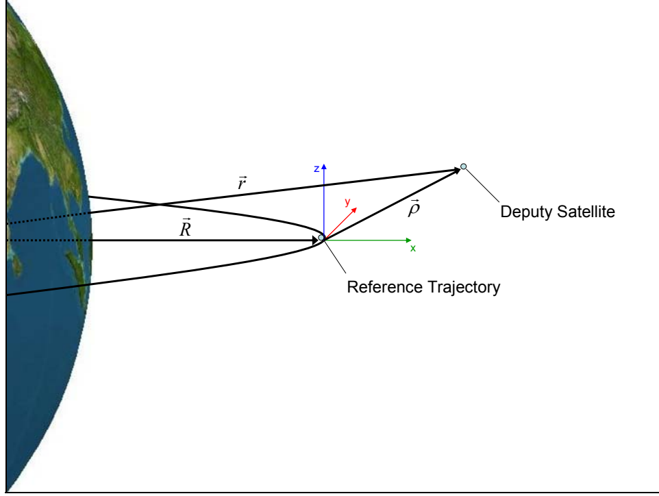
Figure 3. Formation Geometry
