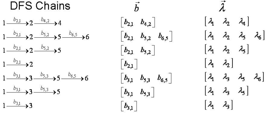
Figure 3 Depth First Search Chain Identification
