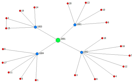
Figure A.1: nodes = 20; range = 0
