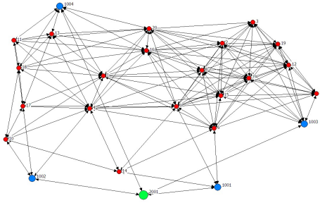
Figure A.5: nodes = 20; range = 10
