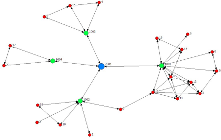
Figure A.3: nodes = 20; range = 3
