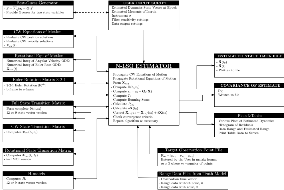
Figure 3.5 Estimator Architecture
