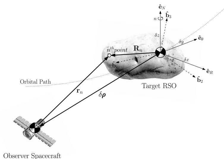
Figure 3.1 Observation Geometry of Observer-Target System
