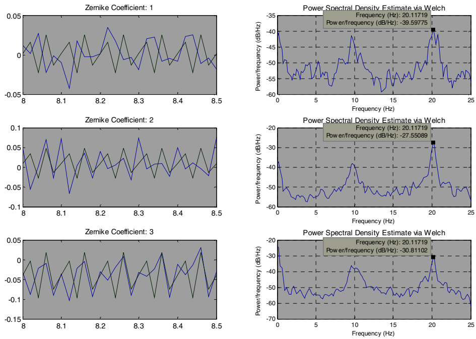
Figure 3.18 Frequency Response 20 Hz (Time Domain/Frequency Domain)
