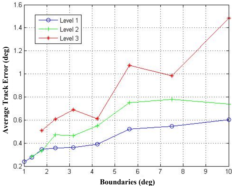
Figure 36 – Mean of Individual Pilot’s Average Tracking Errors
