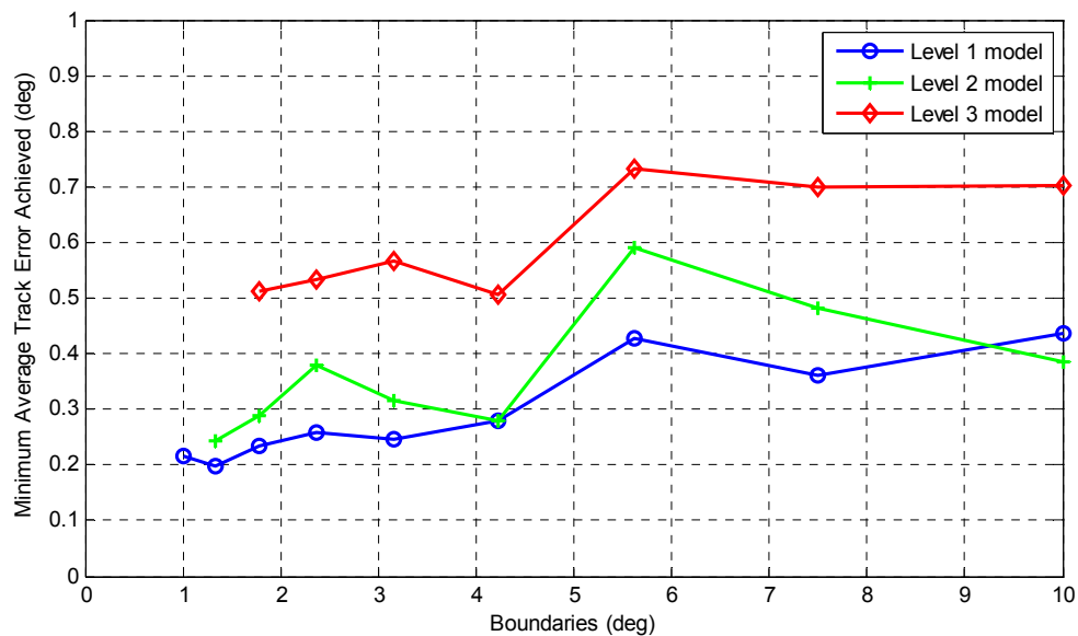
Figure 35 – Minimum Average Track Error - All Pilots, All Test Runs
