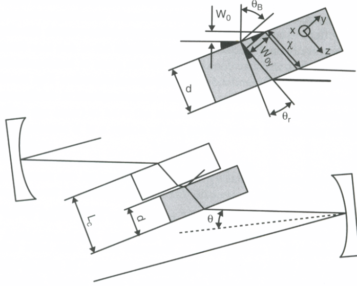
Figure 3.13: Analysis of differing path lengths in the x and y directions to allow correction. [14, p.330]
