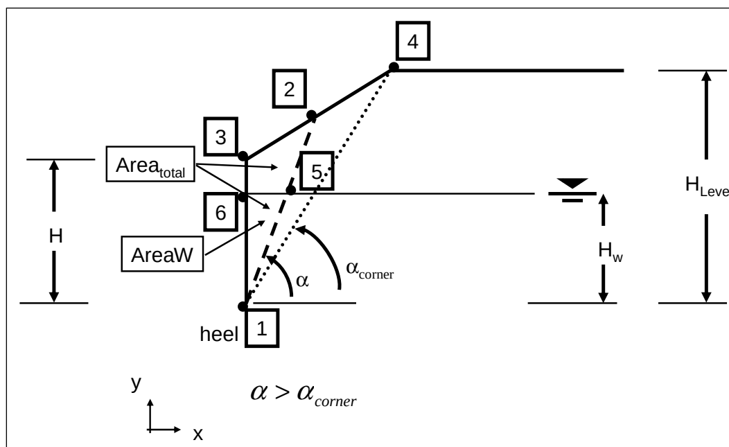
Figure A.5. Soil wedge defined by a bilinear ground surface with \alpha greater than \alpha_{\text{corner}} and no crack.
