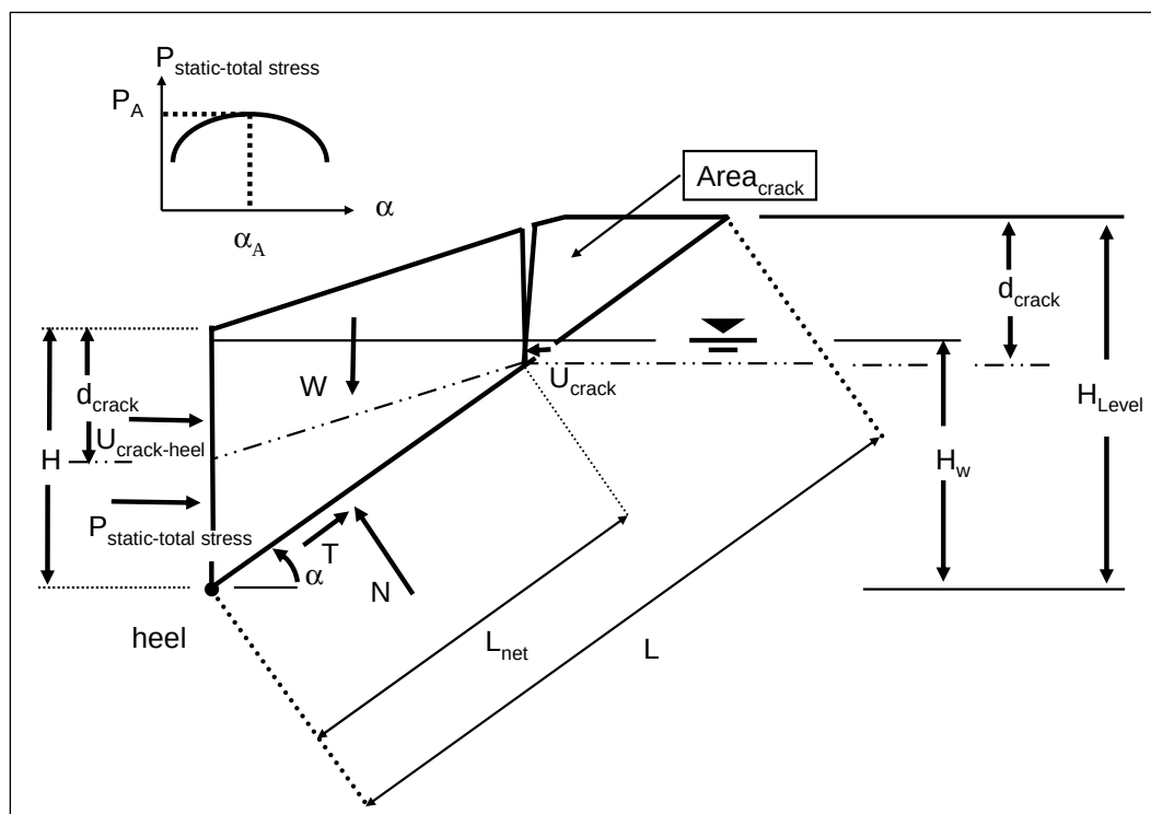
Figure A.4. Static active sweep-search wedge analysis, total stress analysis with a hydrostatic water table (zone of cracking of depth d_{crack} ).
