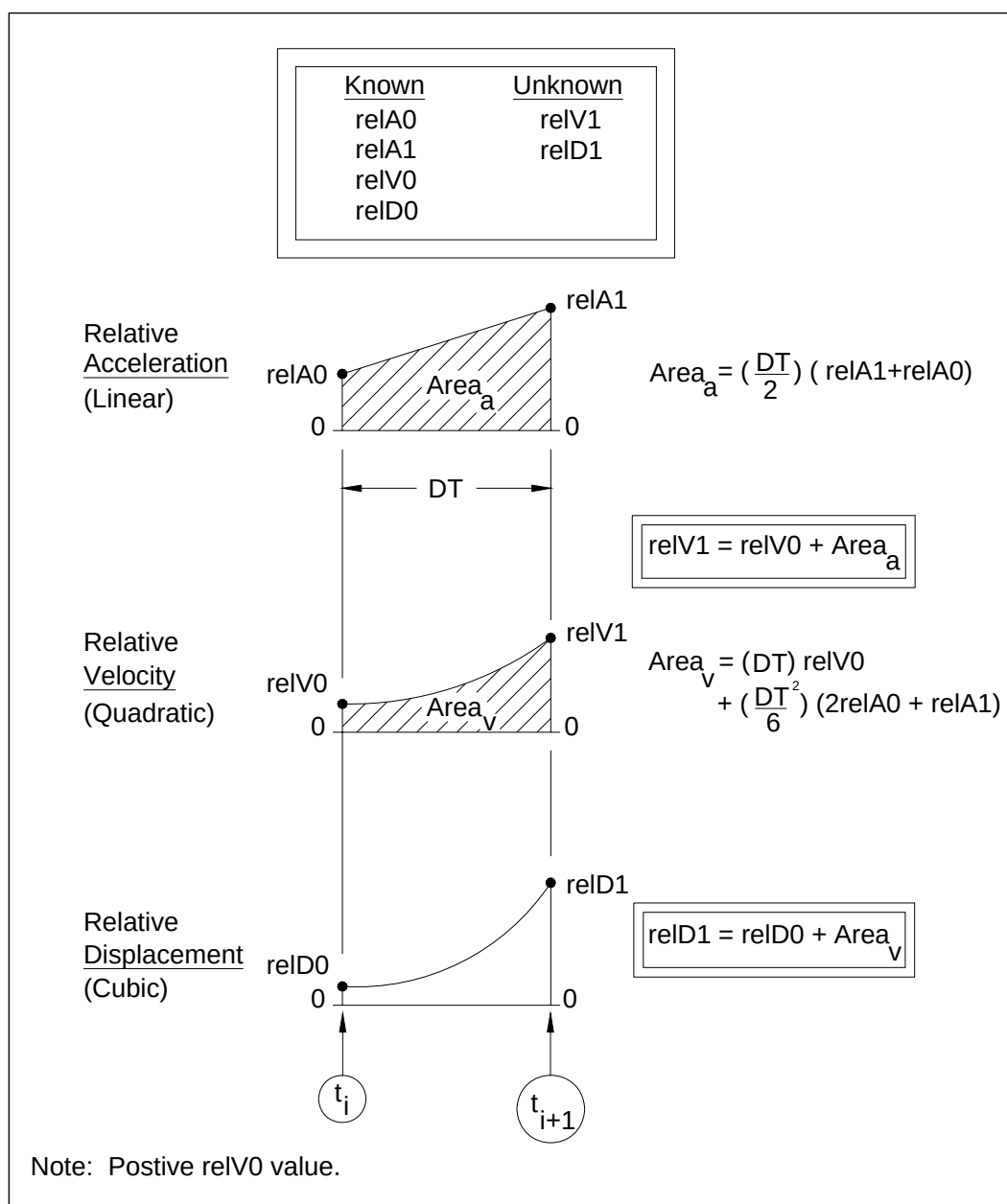
Figure 2.4. Relative velocity and displacements at the end of time increment DT based on linearly varying relative acceleration.
