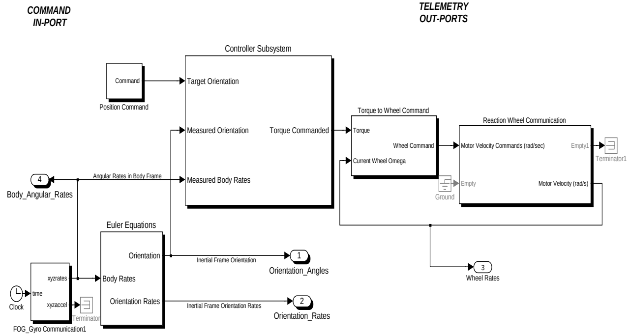
Figure D.1 SimSAT Main Diagram
