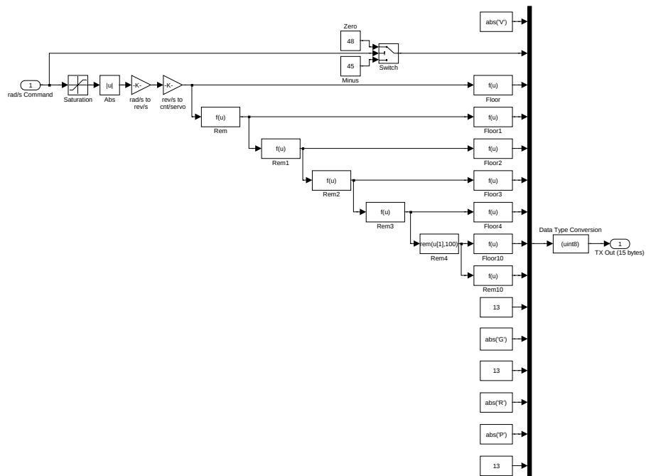
Figure D.11 Reaction Wheel Velocity Encoder
