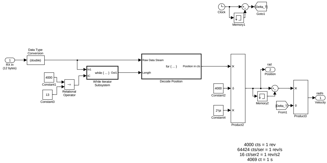
Figure D.7 Reaction Wheel Motor Velocity Decoder
