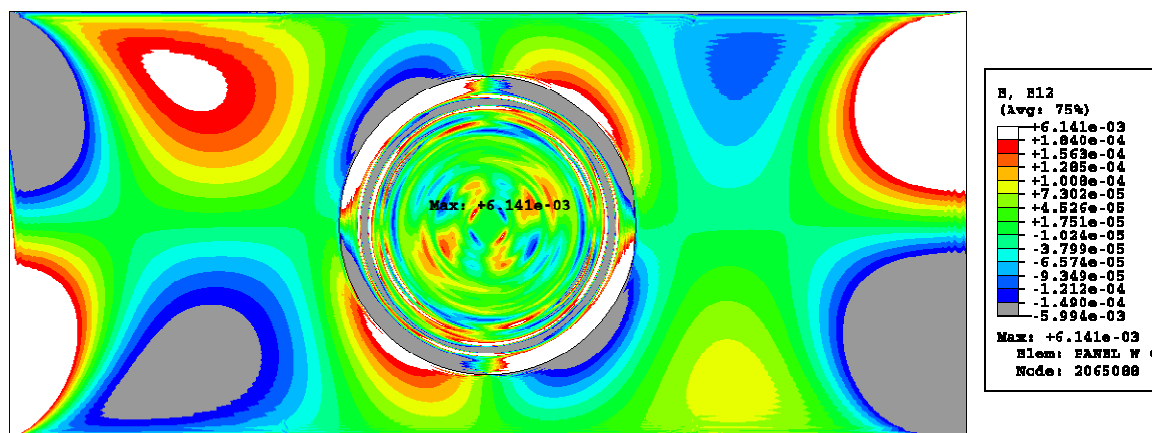
Figure 5.11. \epsilon_{xy} : Finite Element Model
