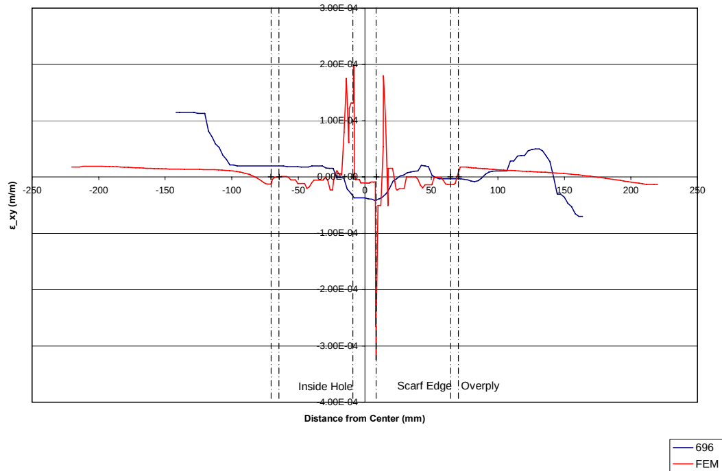
Figure 5.22 \epsilon_{xy} : Data Plot, y=4 , Experimental vs. Finite Element Model
