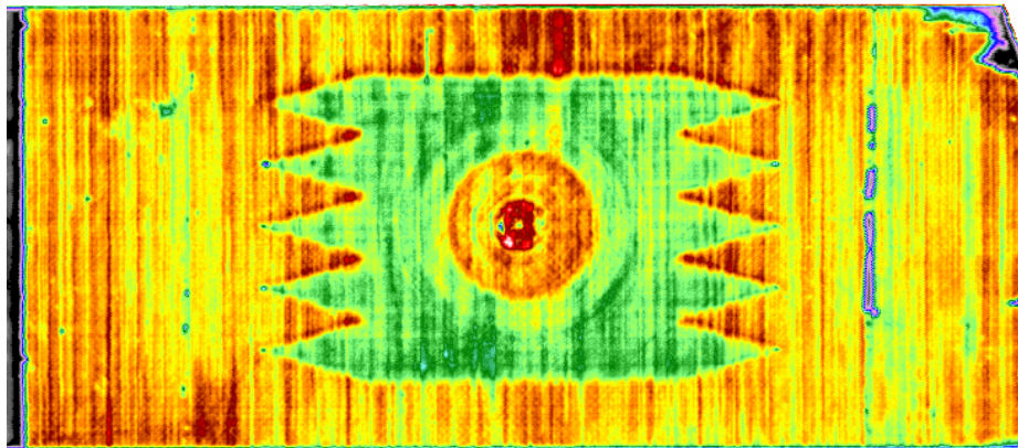
Figure 3.7. Post-Test Ultrasonic Inspection (C-Scan) of Repaired Panel
