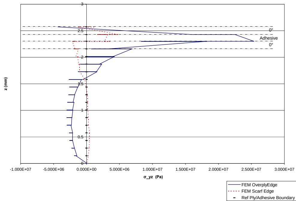
Figure 5.34 \sigma_{yz} Overply and Scarf Edge (Figure 5.33)
