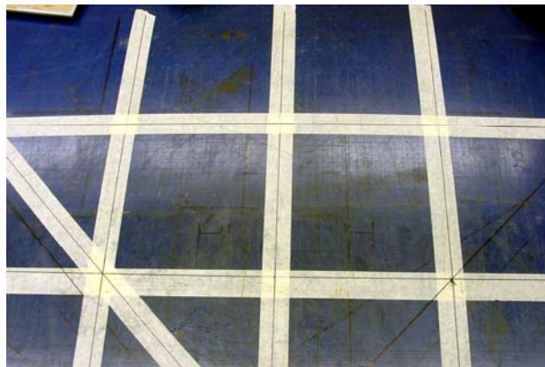
Figure 2.1. Composite Layup Table. Layup Lines Used to for Fiber Orientation
