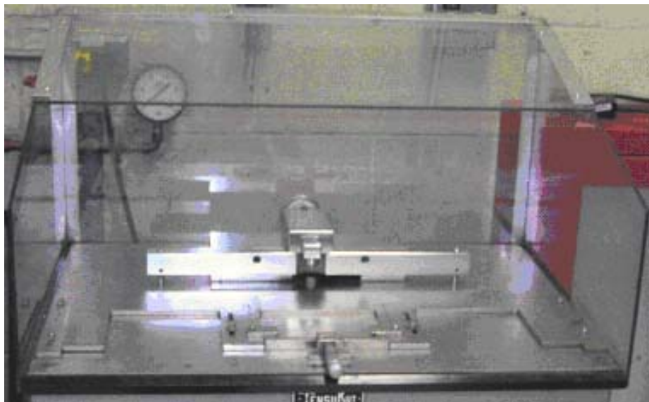
Figure 2.10. Tensile Cut Machine used for Trimming Panel to Final Width
