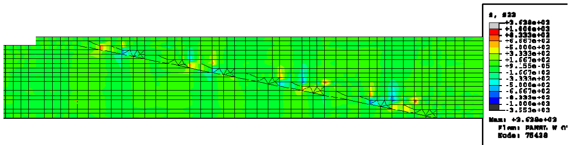
Figure 5.33 \sigma_{yz} Repair Cross-Section, y=4
