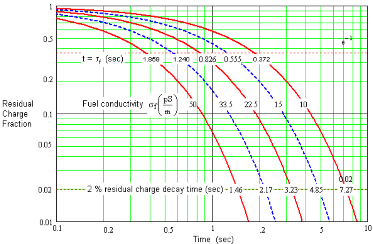
Figure 15. Relative Charge Decay Versus Time for Hydrocarbon Fuels
