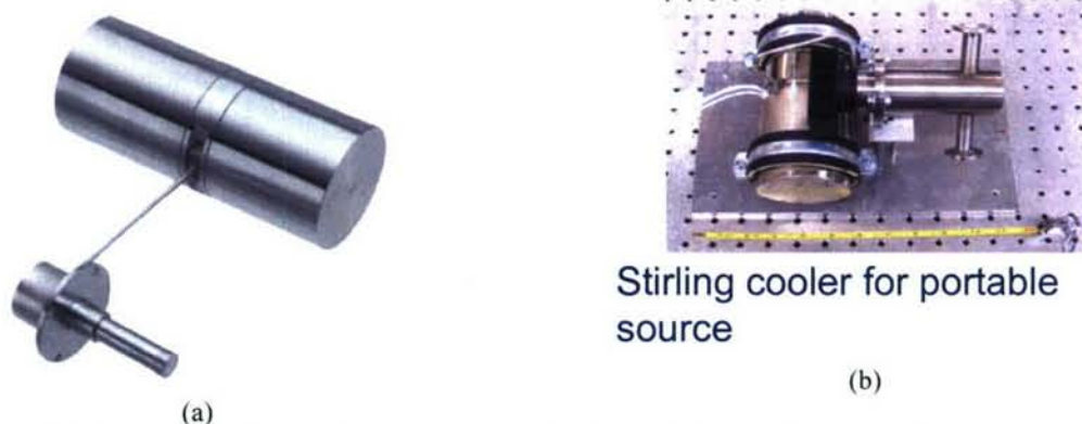
Figure 15. A picture of the AIM (AEG INFRAROT-MODULE GmbH) SL200 Cryogenic Linear Drive Stirling Cooler that we are using to develop a portable THz source. The cold finger is the lower-left small cylinder that will be mounted inside an evacuated chamber to avoid frost. The THz beam emits from a transparent TPX window. Overall size is about 10 cm on a side. Right panels show the cooler on an optical bench at the University of Delaware.
