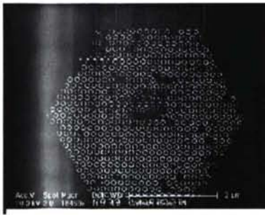
Figure 6. First InGaP photonic crystal laser emitting in the red (680nm) wavelength range.
