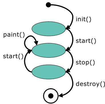
Figure 6.1: Applet callbacks
