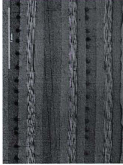
70µm HGF spacing within a 16 ply [-45^\circ/90^\circ/+45^\circ/0^\circ]_{2s} CFRP (T300/914)
