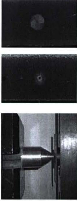
Indentation (1400N) ↓
