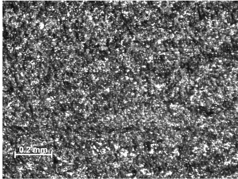
Figure 23 – Micrograph of sample 02-04 (diamond saw machined), demonstrating the substantial difference between the machined surfaces of diamond saw and water jet machined samples of PMR-15 neat resin aged for 100 h in air at 288°C.
