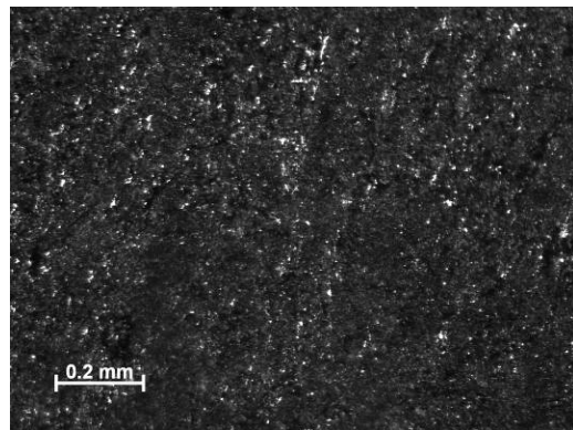
Figure 94 –Sample 12-07, PMR-15 neat resin aged in argon for 50 h, T = 288^{\circ}\text{C} , Creep stress = 10 MPa. Machined with water jet.
