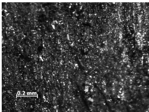
Figure 125 –Sample 12-07, PMR-15 neat resin aged in argon for 1000 h, T = 288^{\circ}\text{C} , Creep stress = 10 MPa. Machined with water jet showing slight microcracking.
