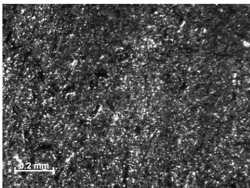
Figure 89 – Sample 12-06, PMR-15 neat resin aged in air for 1000 h, T = 288^{\circ} . Before testing, Machined with water jet.
