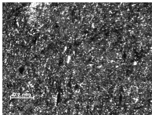
Figure 90 –Sample 12-06, PMR-15 neat resin aged in air for 1000 h, T = 288^{\circ}\text{C} , Creep stress = 10 MPa. Machined with water jet showing slight microcracking..
