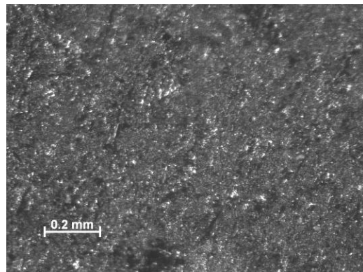
Figure 80 –Sample 12-19, PMR-15 neat resin aged in air for 250 h, T = 288^{\circ}\text{C} , Creep stress = 10 MPa. Machined with water jet.
