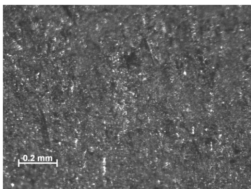
Figure 101 –Sample 13-03, PMR-15 neat resin aged in argon for 100 h, T = 288^{\circ} . Before testing, Machined with water jet.
