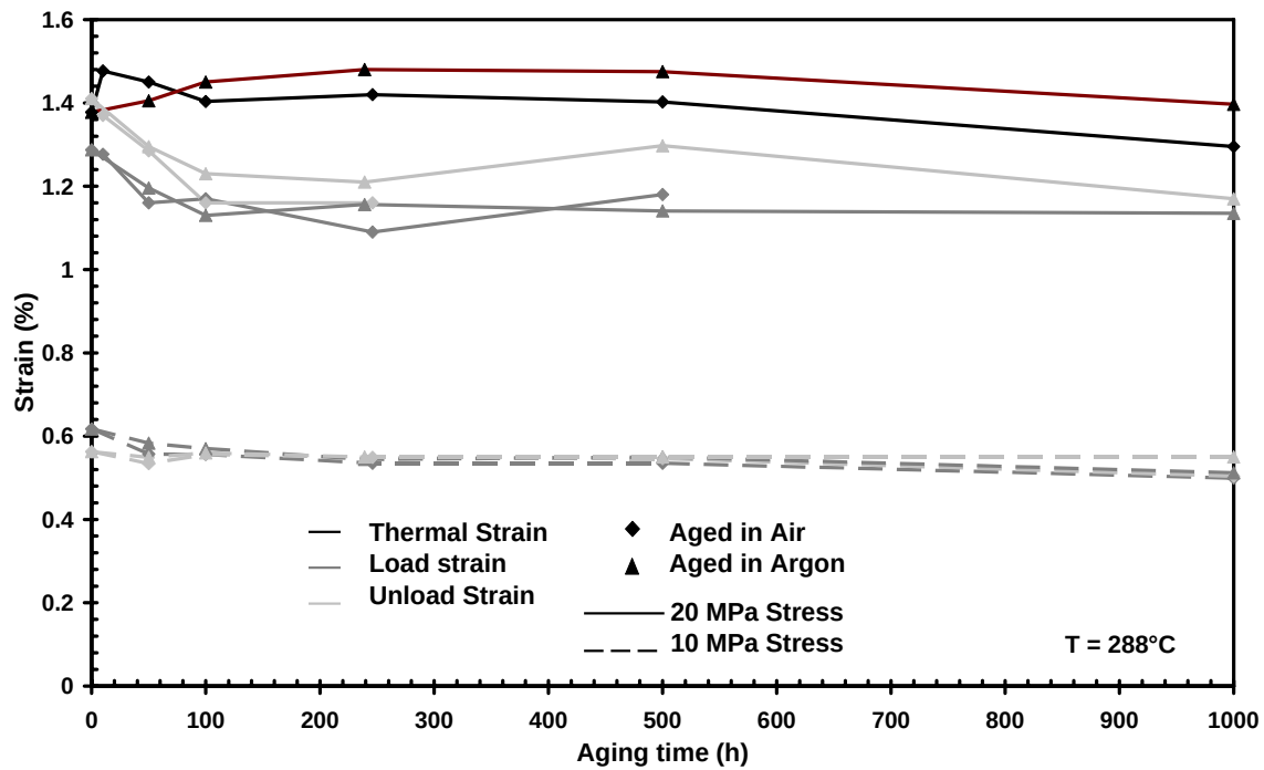
Figure 33 – Average thermal, loading and unloading strains versus aging time for PMR-15 neat resin specimens subjected to prior aging in air or in argon and creep at 10 or 20 MPa at 288°C.
