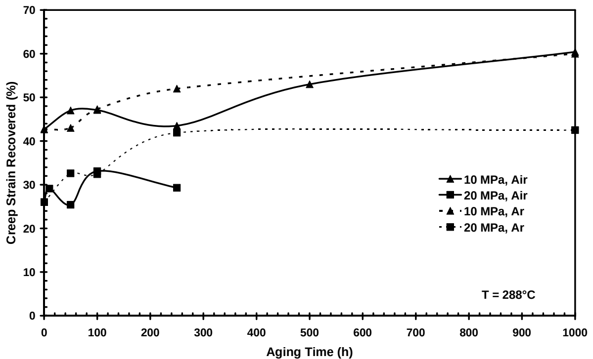
Figure 45 – Creep strain recovered in 50 h as a function of prior aging time at 288°C for PMR-15 neat resin. Recovered creep strain increases with increasing prior aging time in either environment.
