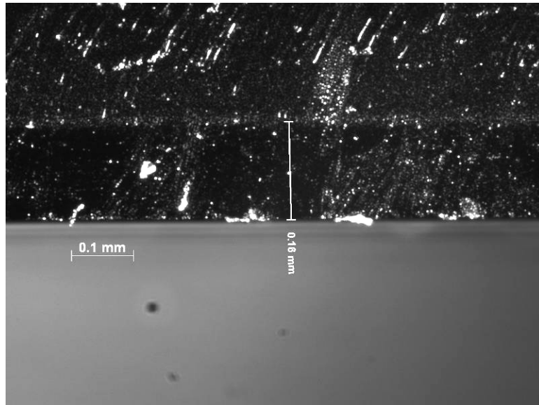
Figure 19 –Photograph showing the visible oxidation layer on the fracture surface of a PMR-15 neat resin sample aged for 1000 h at 288°C in air and tested in creep.
