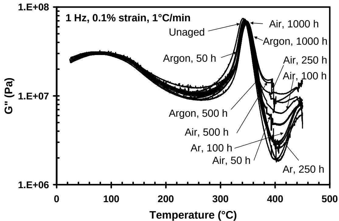
Figure 48 – Loss Modulus versus temperature as determined by DMA for samples aged in air and in argon at 288°C. The temperature at the peak of the curve increased moderately with increasing prior aging time.
