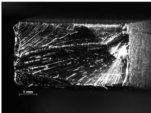
Figure 69 –Sample 12-18, PMR-15 neat resin aged in air for 100 h, T = 288^{\circ}\text{C} , Creep stress = 20 MPa. Machined with water jet, showing slight microcracking.
