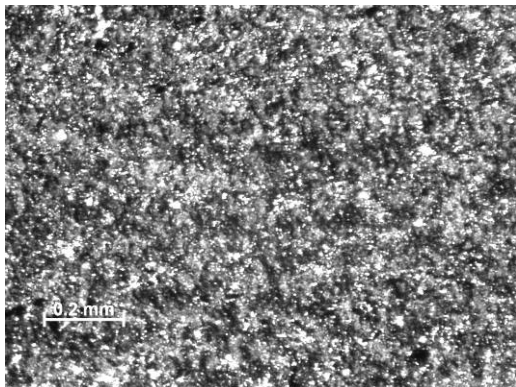
Figure 71 –Sample 11-16, PMR-15 neat resin aged in air for 100 h, T = 288^{\circ} . Before testing, Machined with diamond saw.
