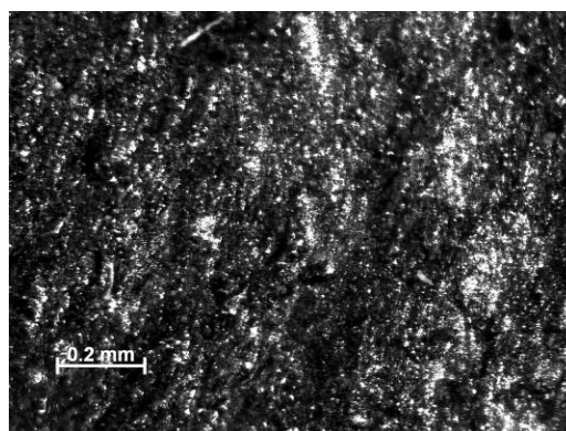
Figure 98 –Sample 12-14, PMR-15 neat resin aged in argon for 100 h, T = 288^{\circ}\text{C} , Creep stress = 10 MPa. Machined with water jet.
