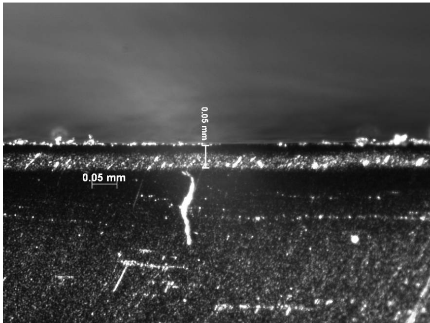
Figure 128 – Oxidation layer observed on fracture surface of sample aged in air at 288°C for 100 h. Showing formation of an oxidation layer 0.05 mm thick.
