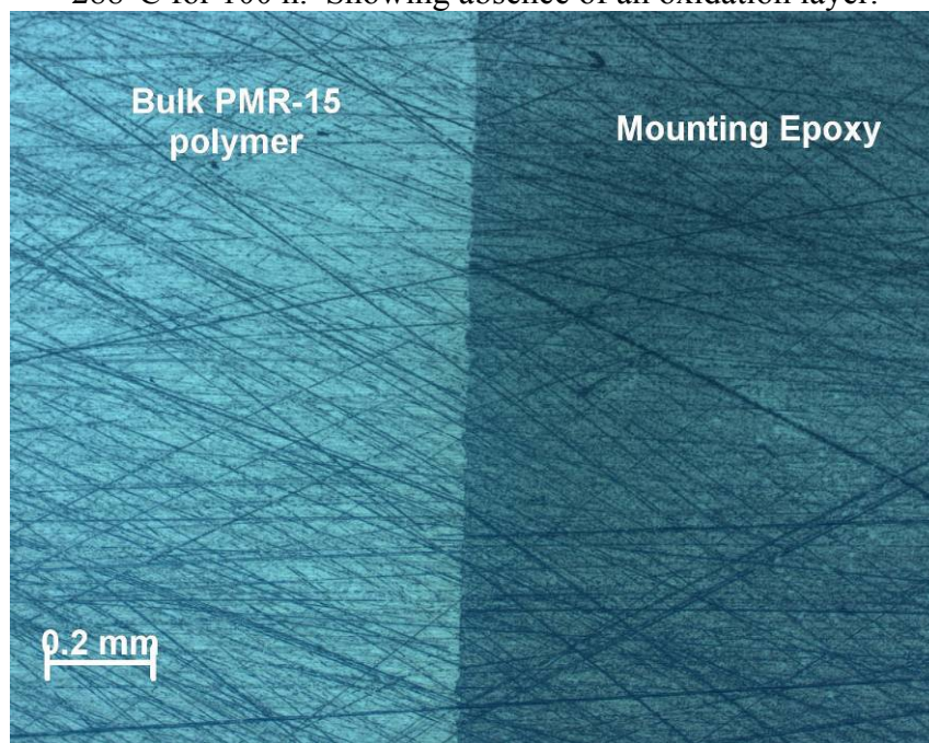
Figure 138 – Oxidation layer observed polished section of sample aged in argon at 288°C for 100 h. Showing absence of an oxidation layer.
