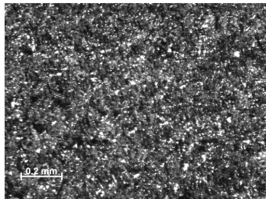
Figure 78 –Sample 02-05, PMR-15 neat resin aged in air for 250 h, T = 288^{\circ}\text{C} , Creep stress = 10 MPa. Machined with diamond saw.
