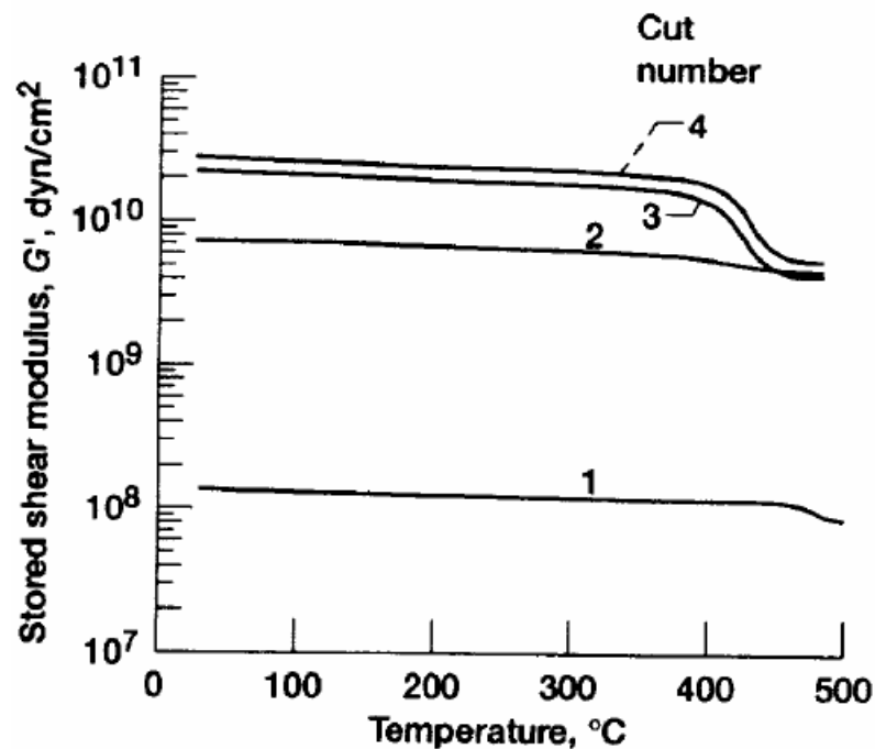
Figure 7 – Stored shear modulus of T650-35/PMR-15 composite as a function of temperature for various depth cuts. Samples aged in air at 360°C for 2090 h. Sample #1 is the surface sample. Figure from Ref. [3].
