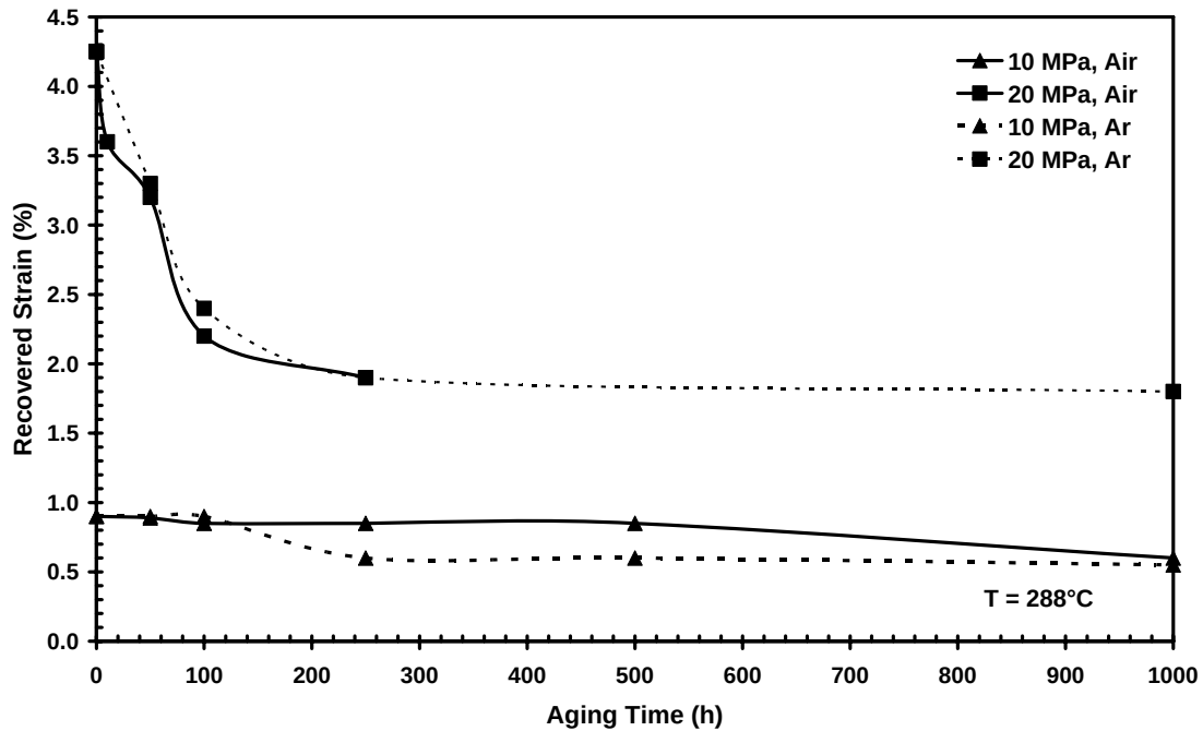
Figure 42 – Strain recovered after 50 h at zero stress as a function of aging time for PMR-15 neat resin. Recovered strain decreases with increasing prior aging time.
