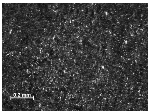
Figure 115 –Sample 12-20, PMR-15 neat resin aged in argon for 500 h, T = 288^{\circ} . Before testing, Machined with water jet.
