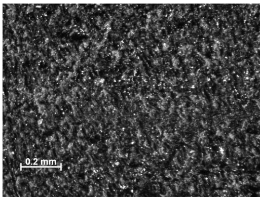
Figure 51 – Sample 02-01, as-processed PMR-15 neat resin, Creep stress = 20 MPa. Machined with diamond saw.
