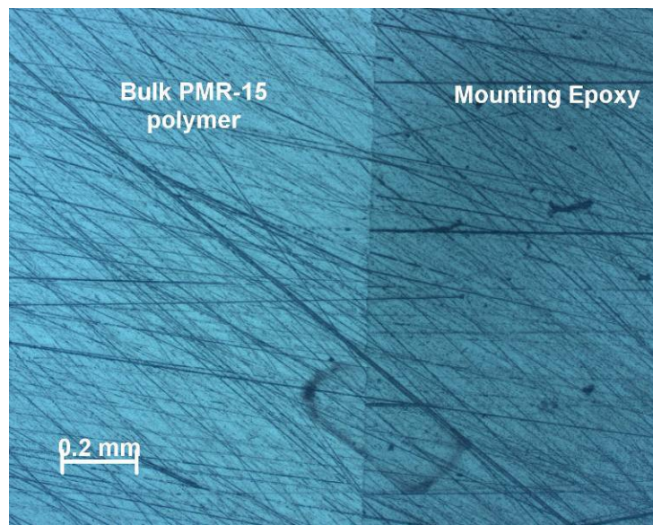
Figure 17 –Optical micrograph showing the absence of an oxidation layer on the outer surface of PMR-15 neat resin sample aged for 1000 h at 288°C in argon.
