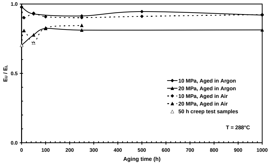
Figure 31 – Ratio of elastic modulus measured upon unloading to the elastic modulus measured upon loading as a function of aging time for various aging environments for PMR-15 neat resin specimens tested in creep at 10 and 20 MPa.
