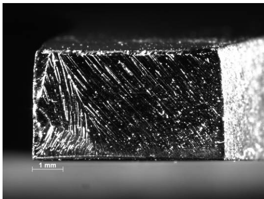
Figure 75 –Sample 13-09, PMR-15 neat resin aged in air for 250 h, T = 288^{\circ}\text{C} , Creep stress = 20 MPa. Machined with water jet showing microcracking.
