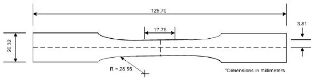
Figure 13 –Dog bone tensile specimens with nominal dimensions shown. Figure from Ref. [22:47].
