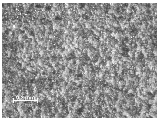
Figure 95 –Sample 11-03, PMR-15 neat resin aged in argon for 100 h, T = 288^{\circ} . Before testing, Machined with diamond saw.
