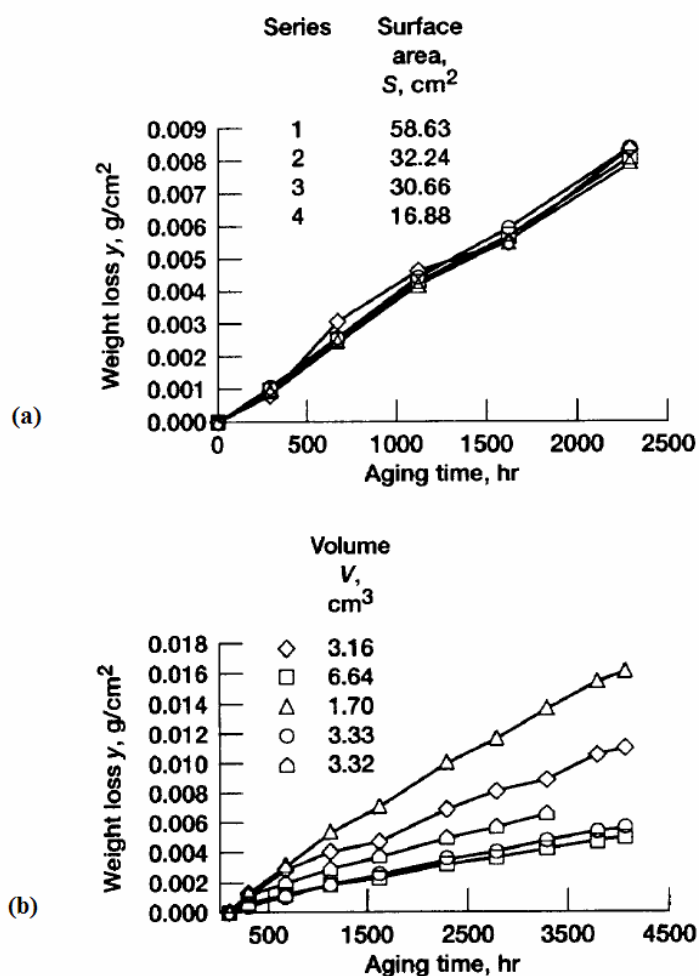
Figure 4 - PMR-15 neat resin aged in air at 288°C. Weight loss normalized by surface area as a function of aging time for (a) various sample surface areas and (b) various sample volumes. Figure from Ref. [3].
