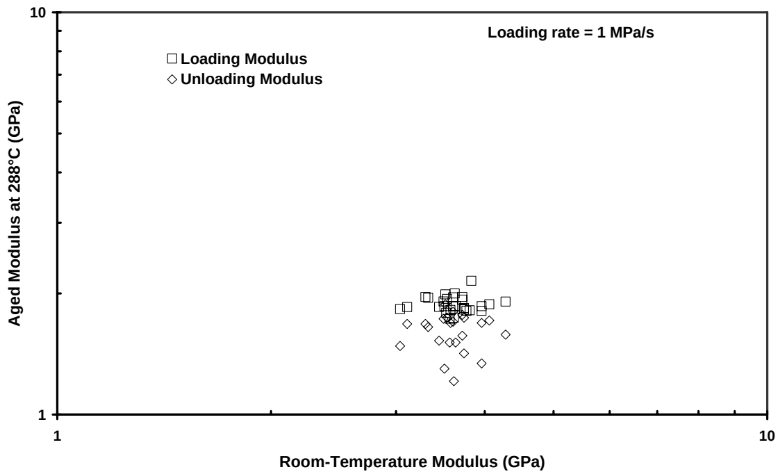
Figure 25 –Elastic modulus of aged samples measured at 288°C versus initial room temperature elastic modulus for PMR-15 neat resin.
