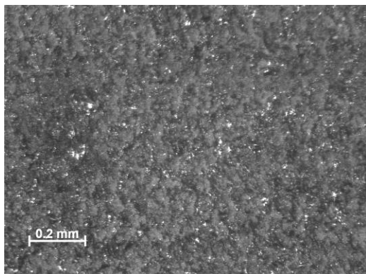
Figure 103 –Sample 11-18, PMR-15 neat resin aged in argon for 250 h, T = 288^{\circ} . Before testing, Machined with diamond saw.
