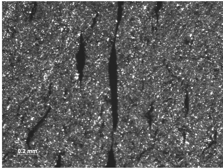
Figure 22 –Sample 12-18 (water jet machined), showing the presence of significant surface micro cracking on the machined surface of the gauge section. PMR-15 neat resin aged for 100 h in air at 288°C.
