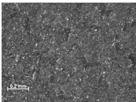
Figure 97 –Sample 12-14, PMR-15 neat resin aged in argon for 100 h, T = 288^{\circ} . Before testing, Machined with water jet.
