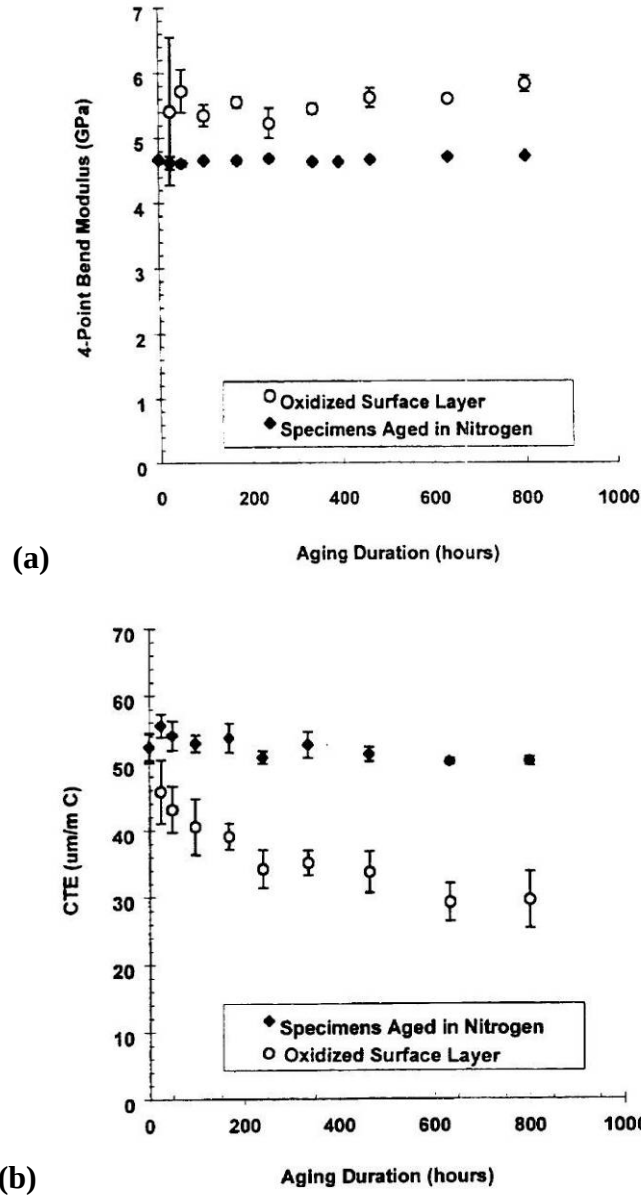
Figure 9 – (a), 4 point bend modulus and (b) CTE for both oxidized and unoxidized material as a function of aging time at 316°C for PMR-15 neat resin. Figures from Ref. [14].
