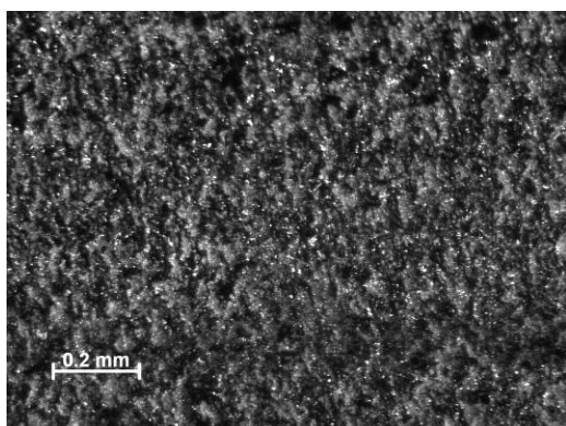
Figure 111 –Sample 11-09, PMR-15 neat resin aged in argon for 500 h, T = 288^{\circ} . Before testing, Machined with diamond saw.
