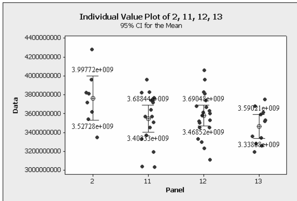
Figure 21 – Initial room temperature elastic modulus data as a function of origin panel number, with 95% confidence intervals for each panel. Figure produced using MiniTab program.
