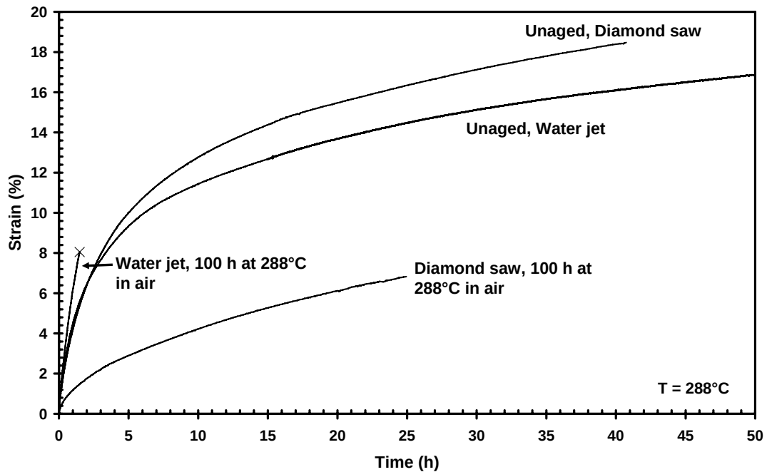
Figure 24 – Creep curves obtained for diamond saw and water jet machined samples. Results for the as-processed (unaged) material and material aged for 100 h in air at 288°C are shown.
