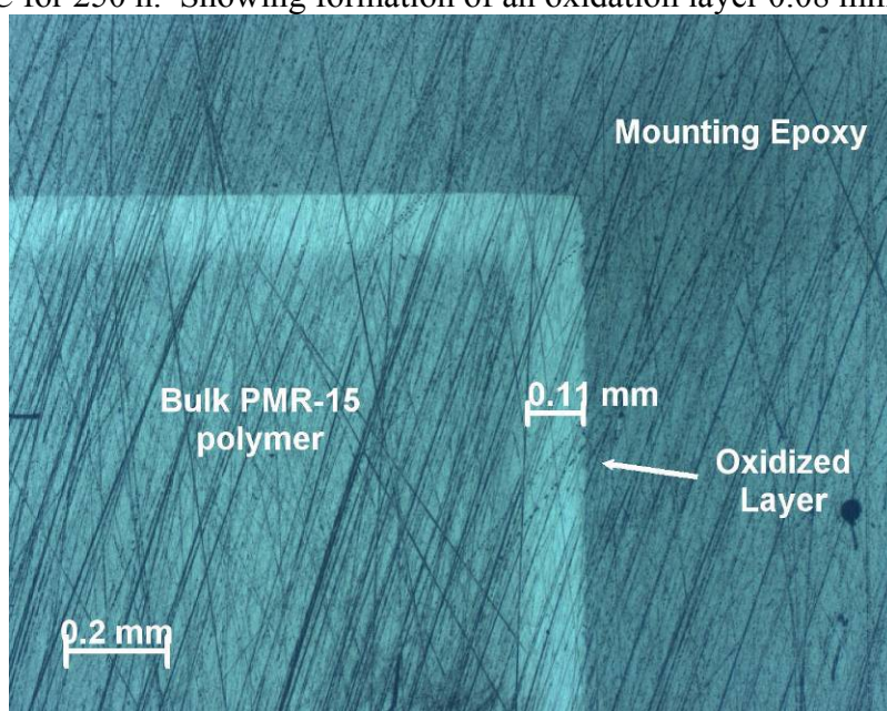
Figure 135 – Oxidation layer observed on polished section of sample aged in air at 288°C for 500 h. Showing formation of an oxidation layer 0.11 mm thick.
