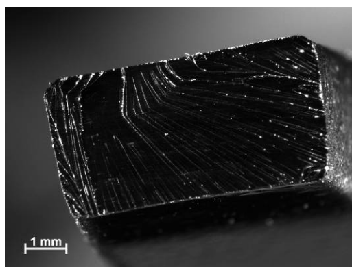
Figure 124 –Sample 12-03, PMR-15 neat resin aged in argon for 1000 h, T = 288^{\circ}\text{C} , Creep stress = 20 MPa. Machined with water jet showing fracture line and surface.
