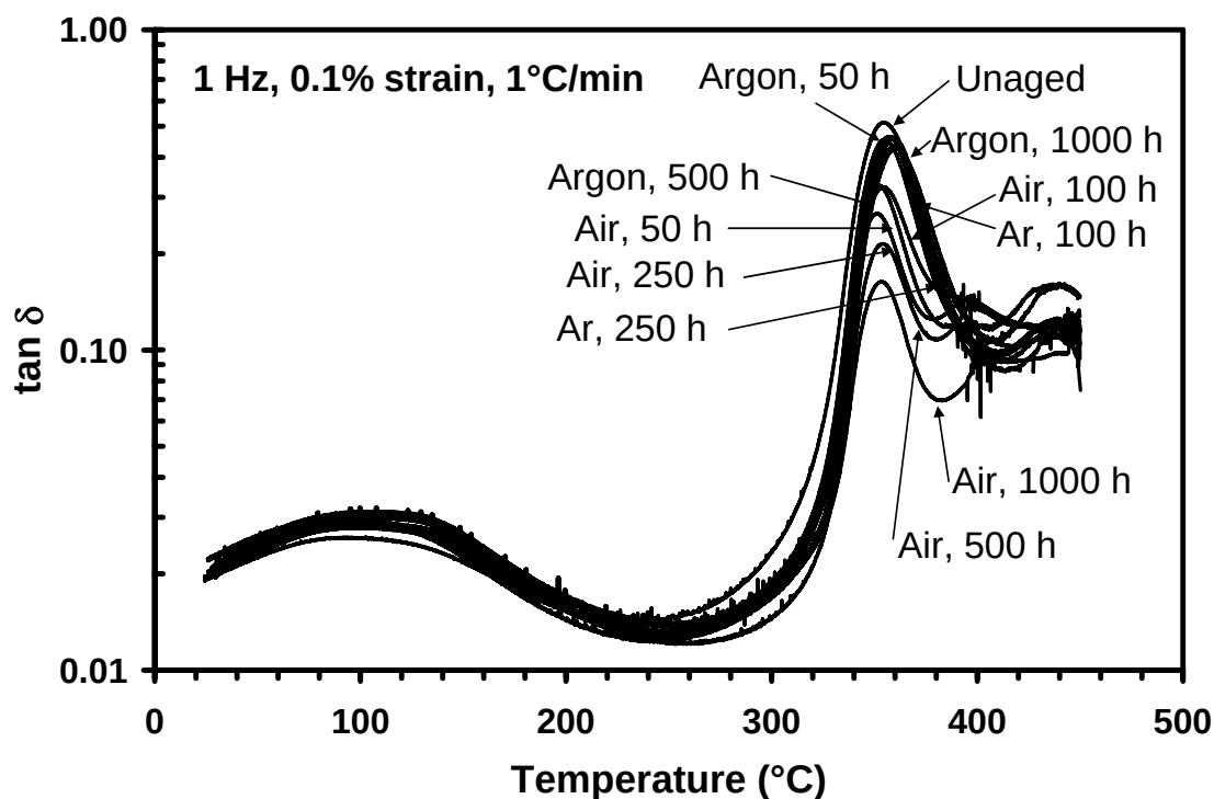
Figure 49 – \tan \delta versus temperature as determined by DMA for samples aged in air or in argon at 288 ^{\circ}\text{C} . The peak value of the ratio decreases with increasing prior aging time.
