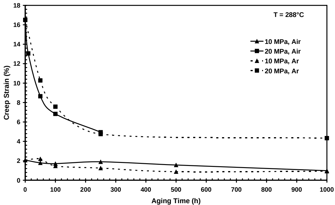
Figure 37 – Creep strain accumulated in 25 h as a function of aging time for PMR-15 neat resin. Creep strain accumulation decreases with increasing prior aging time.
