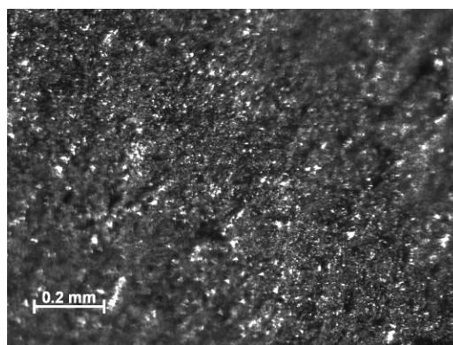
Figure 106 –Sample 12-12, PMR-15 neat resin aged in argon for 250 h, T = 288^{\circ}\text{C} , Creep stress = 20 MPa. Machined with water jet.
