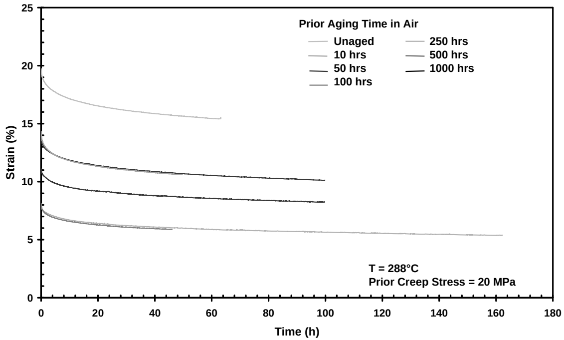
Figure 38 – Recovery curves for PMR-15 neat resin aged in air at 288°C. Prior creep stress = 20 MPa, test temperature = 288°C.
