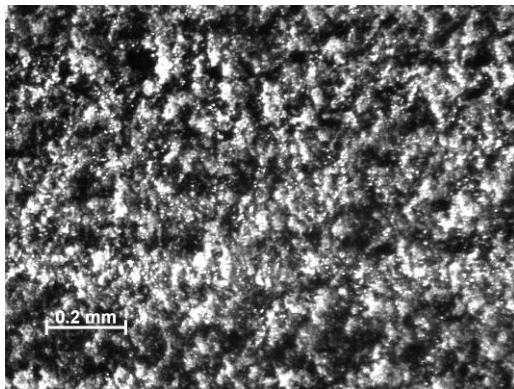
Figure 55 – Sample 02-08, as-processed PMR-15 neat resin. Before testing, Machined with diamond saw.
