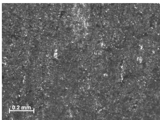
Figure 105 –Sample 12-12, PMR-15 neat resin aged in argon for 250 h, T = 288^{\circ} . Before testing, Machined with water jet.
