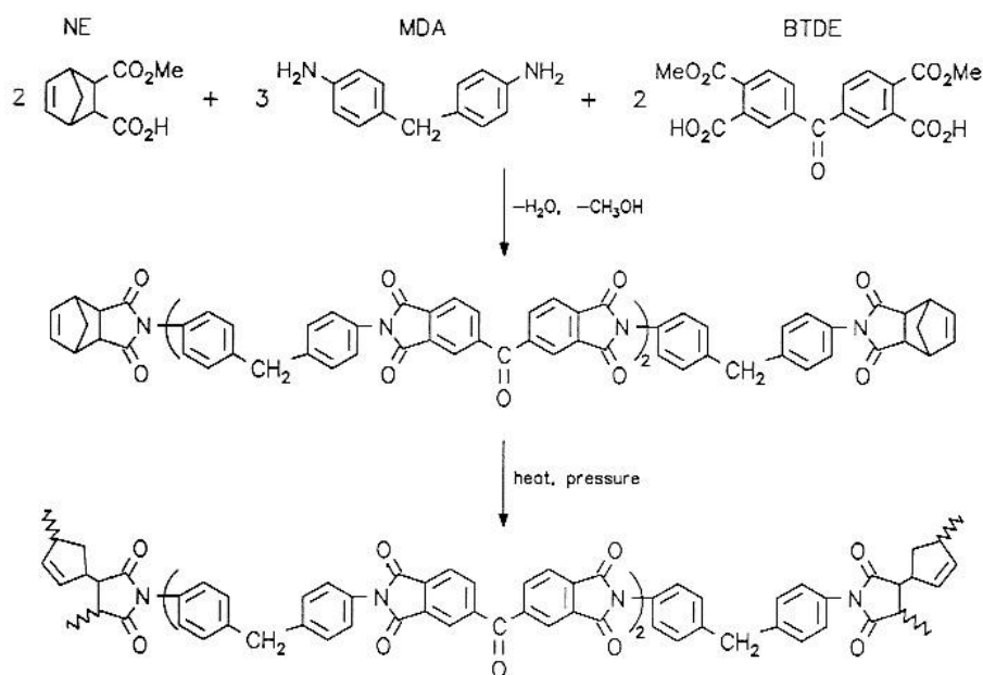
Figure 1 - Classical chemistry of PMR-15. Figure from Ref. [5].
