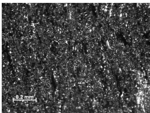
Figure 117 –Sample 12-06, PMR-15 neat resin aged in argon for 500 h, T = 288^{\circ} . Before testing, Machined with water jet.
