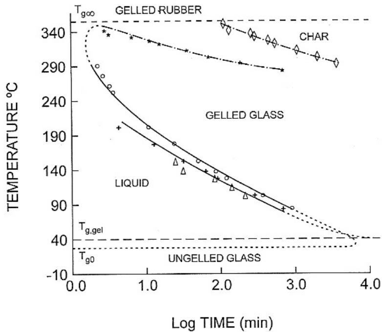
Figure 12 – TTT diagram for an epoxy thermosetting polymer system showing possible degradation after long periods of exposure at temperatures below T_{g,\infty} . Figure from Ref. [20:142].
