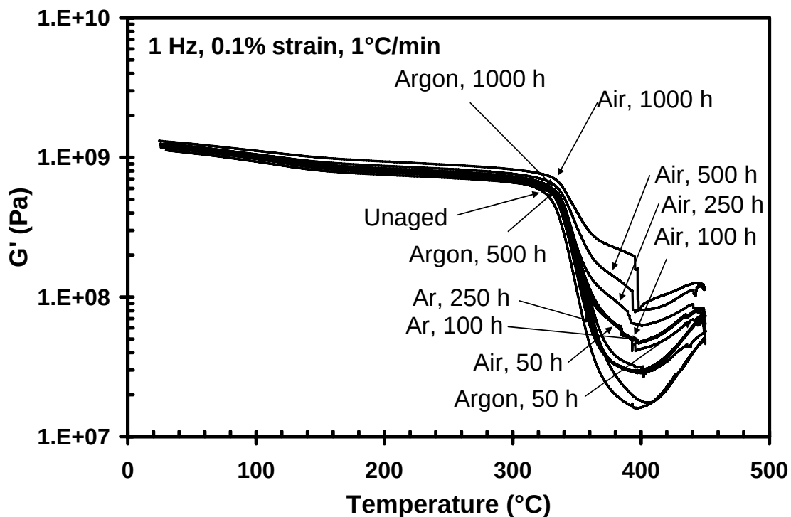
Figure 47 – Storage Modulus versus temperature as determined by DMA for samples aged in air or argon at 288°C. The transition temperature increased with increased prior aging time.
