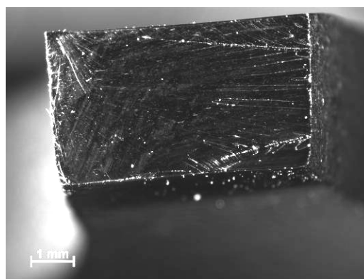
Figure 118 –Sample 13-06, PMR-15 neat resin aged in argon for 500 h, T = 288^{\circ}\text{C} , Creep stress = 20 MPa. Machined with water jet showing microcracking around the fracture line and surface.
