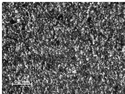
Figure 88 –Sample 02-07, PMR-15 neat resin aged in air for 1000 h, T = 288^{\circ}\text{C} , Creep stress = 10 MPa. Machined with diamond saw.
