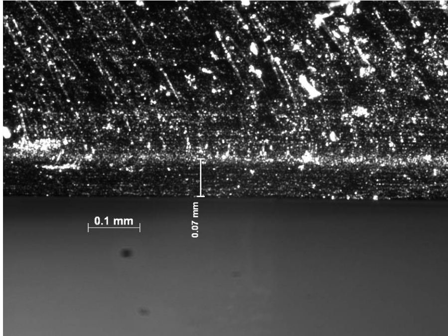
Figure 129 – Oxidation layer observed on fracture surface of sample aged in air at 288°C for 250 h. Showing formation of an oxidation layer 0.07 mm thick.
