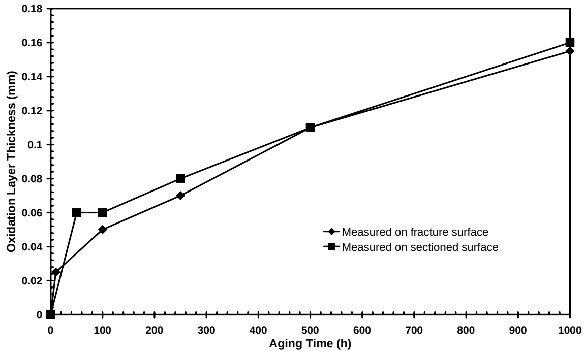
Figure 20 –Oxidation layer thickness measured on both cross sectional cut and fracture surfaces as a function of aging time in air at 288°C for PMR-15 neat resin.
