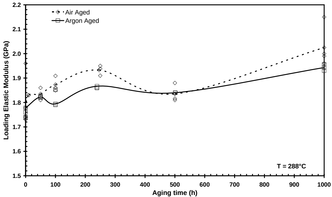
Figure 27 – Elastic modulus upon loading versus aging time in air and in argon at 288°C for PMR-15 neat resin.
