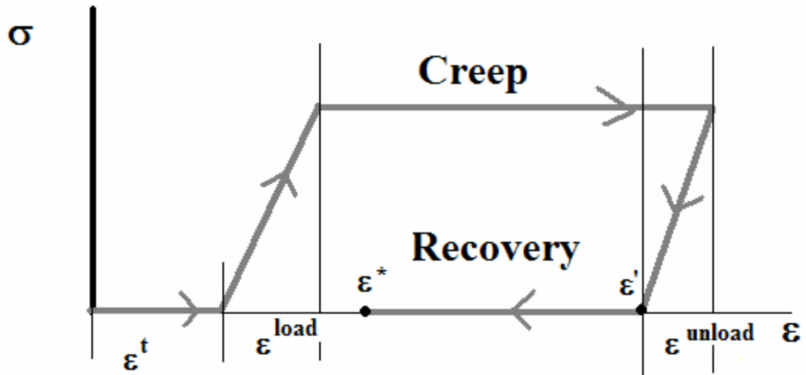
Figure 39 – Schematic stress-strain curve for a constant stress creep period followed by recovery period at zero stress.
