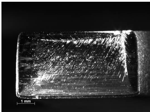
Figure 85 –Sample 12-01, PMR-15 neat resin aged in air for 1000 h, T = 288^{\circ}\text{C} , Creep stress = 20 MPa. Machined with water jet showing slight microcracking around fracture line.
