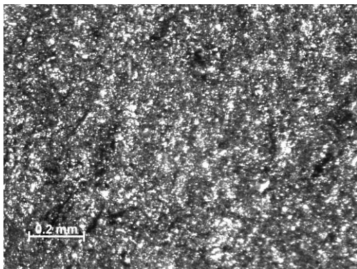
Figure 73 –Sample 12-16, PMR-15 neat resin aged in air for 100 h, T = 288^{\circ} . Before testing, Machined with water jet.
