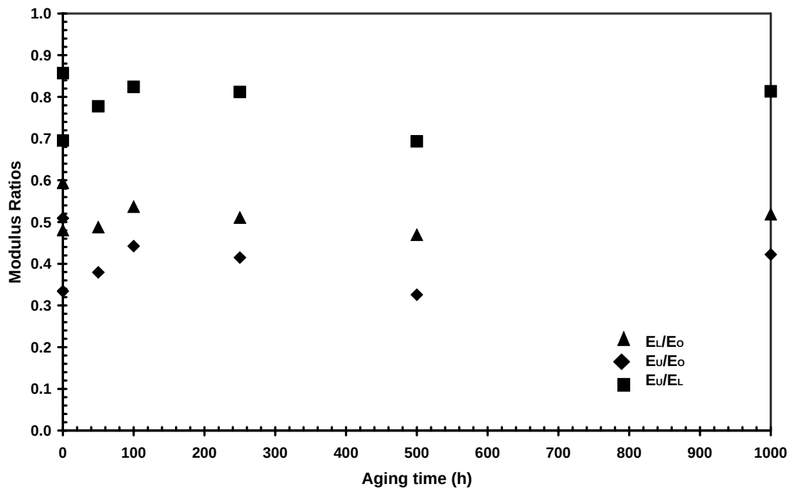
Figure 29 – Elastic modulus ratios versus aging time in argon for PMR-15 neat resin specimens aged at 288°C and tested in creep at 20 MPa at 288°C.
