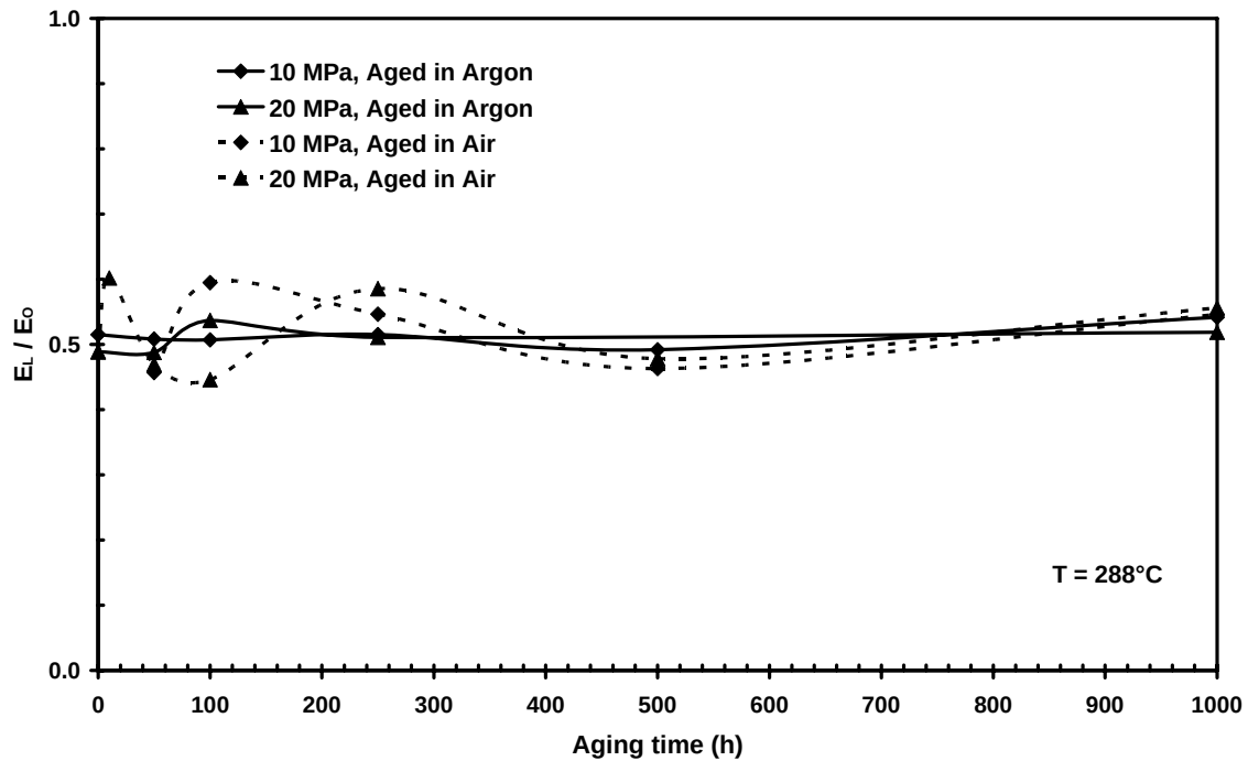
Figure 30 – Ratio of elastic modulus measured upon loading to the initial room-temperature elastic modulus as a function of aging time for various aging environments for PMR-15 neat resin specimens tested in creep at 10 and 20 MPa.
