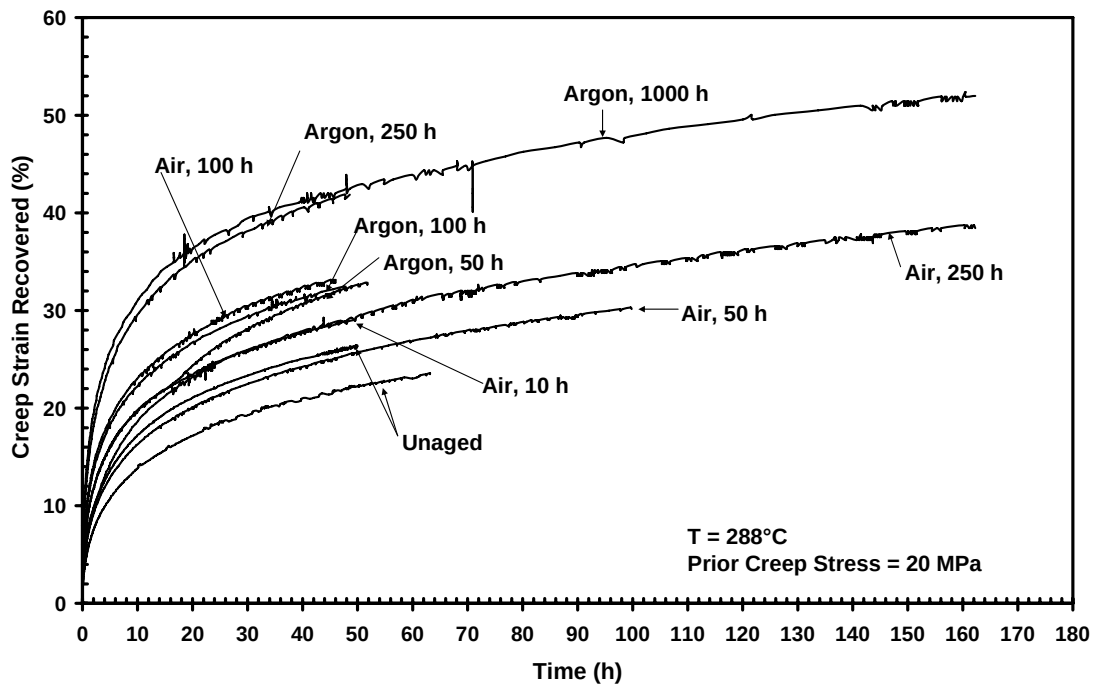
Figure 43 – Creep recovery curves for PMR-15 neat resin aged at 288°C. Prior creep stress = 20 MPa. Recovered creep strain increases with increasing prior aging time.
