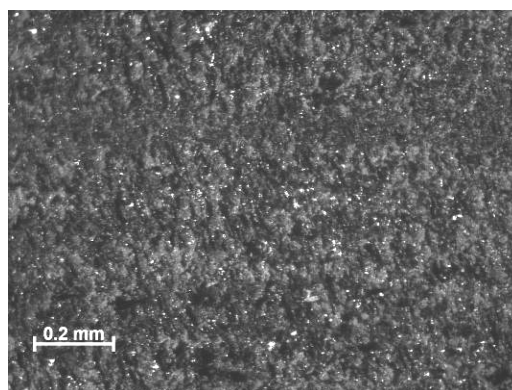
Figure 96 –Sample 11-03, PMR-15 neat resin aged in argon for 100 h, T = 288^{\circ}\text{C} , Creep stress = 10 MPa. Machined with diamond saw.
