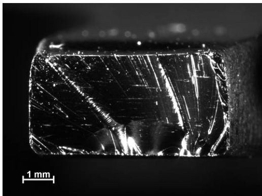
Figure 61 –Sample 12-17, PMR-15 neat resin aged in air for 10 h, T = 288^{\circ}\text{C} , Creep stress = 20 MPa. Machined with water jet showing slight microcracking.
