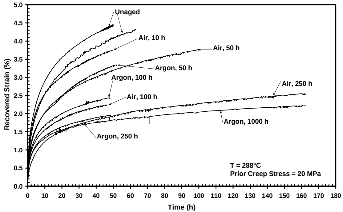
Figure 40 – Recovered strain versus time curves for PMR-15 neat resin aged at 288°C. Creep stress = 20 MPa, test temperature = 288°C. Recovered strain decreases with increasing prior aging time in air or argon.
