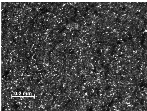
Figure 63 –Sample 12-05, PMR-15 neat resin aged in air for 10 h, T = 288^{\circ}\text{C} , Creep stress = 10 MPa. =Machined with water jet showing slight microcracking.
