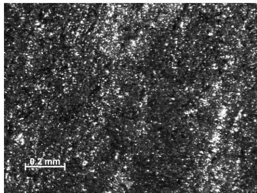
Figure 68 –Sample 12-02, PMR-15 neat resin aged in air for 50 h, T = 288^{\circ}\text{C} , creep stress = 10 MPa. Machined with water jet.
