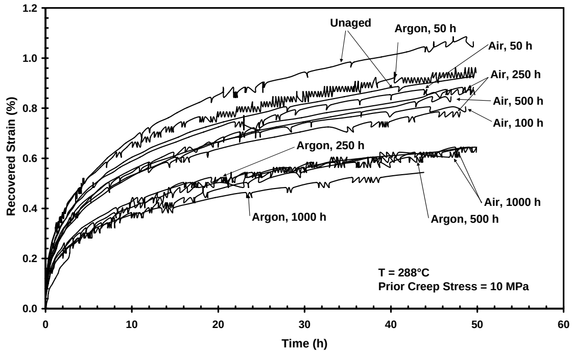
Figure 41 – Recovered strain versus time curves for PMR-15 neat resin aged at 288°C. Creep stress = 10 MPa, test temperature = 288°C. Recovered strain decreases with increasing prior aging time in air or argon.
