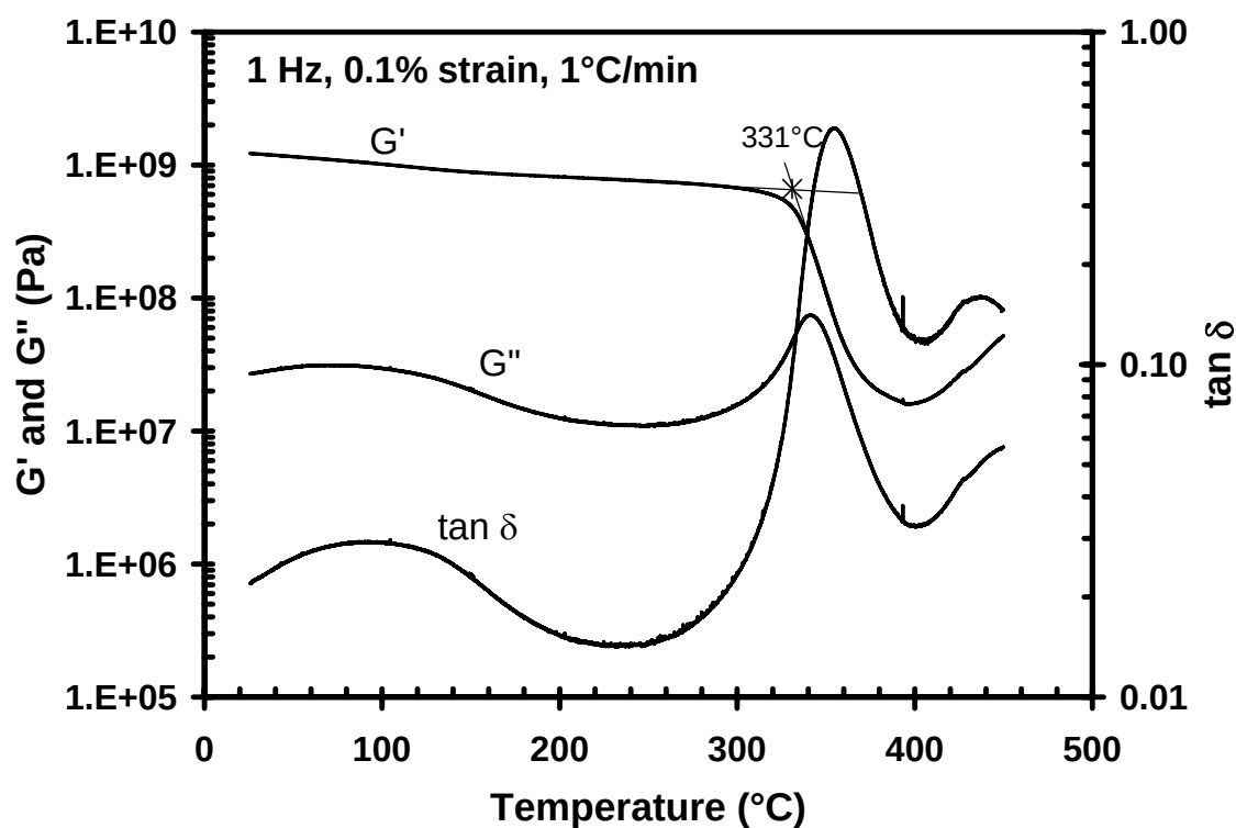
Figure 46 – Results of the DMA tests showing storage modulus, loss modulus and \tan \delta as a function of temperature for an as-processed PMR-15 neat resin. T_g is determined by the intersection of the two slopes of the storage modulus at the transition.
