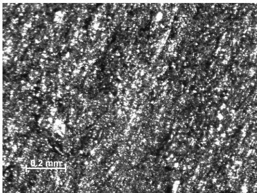
Figure 79 –sample 12-19, PMR-15 neat resin aged in air for 250 h, T = 288^{\circ} . Before testing, Machined with water jet.
