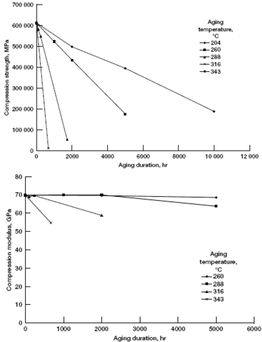
Figure 8— Compression strength and modulus of T650-35/PMR-15 composites as functions of aging time in air at various temperatures. Figure from Ref. [12].
