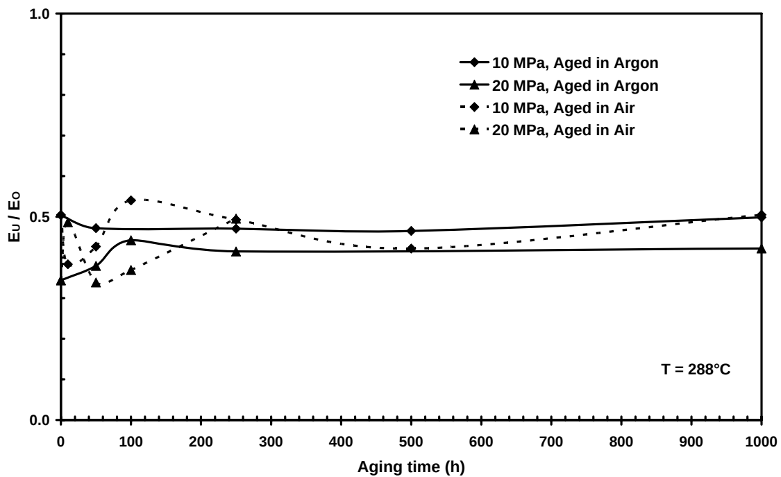
Figure 32 – Ratio of elastic modulus measured upon unloading to the initial room-temperature elastic modulus as a function of aging time for various aging environments for PMR-15 neat resin specimens tested in creep at 10 and 20 MPa.
