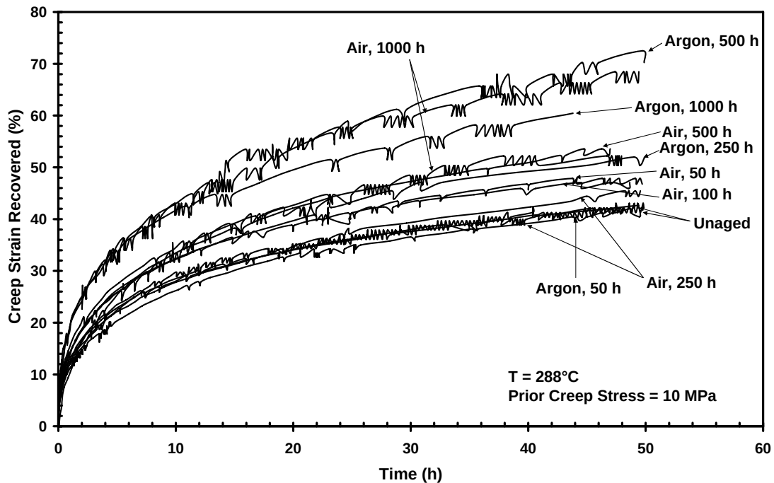
Figure 44 – Creep recovery curves for PMR-15 neat resin aged at 288°C. Prior creep stress = 10 MPa. Recovered creep strain increases with increasing prior aging time.
