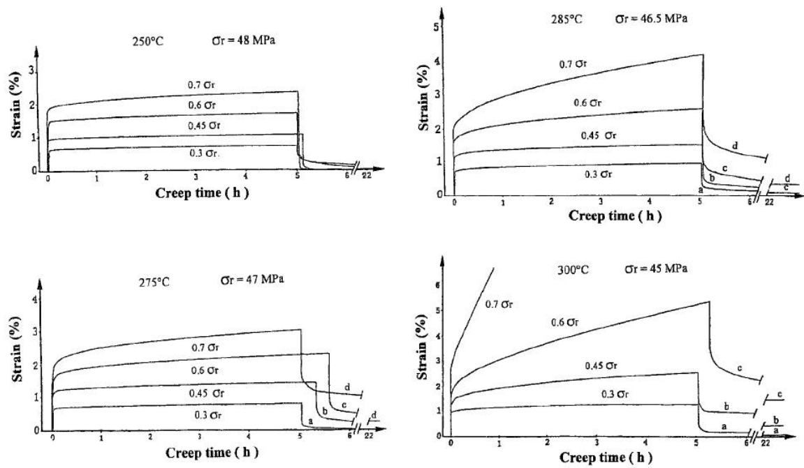
Figure 10 –Creep and recovery curves at multiple temperatures and stress levels for PMR-15 neat resin. Figures from Ref. [16].
