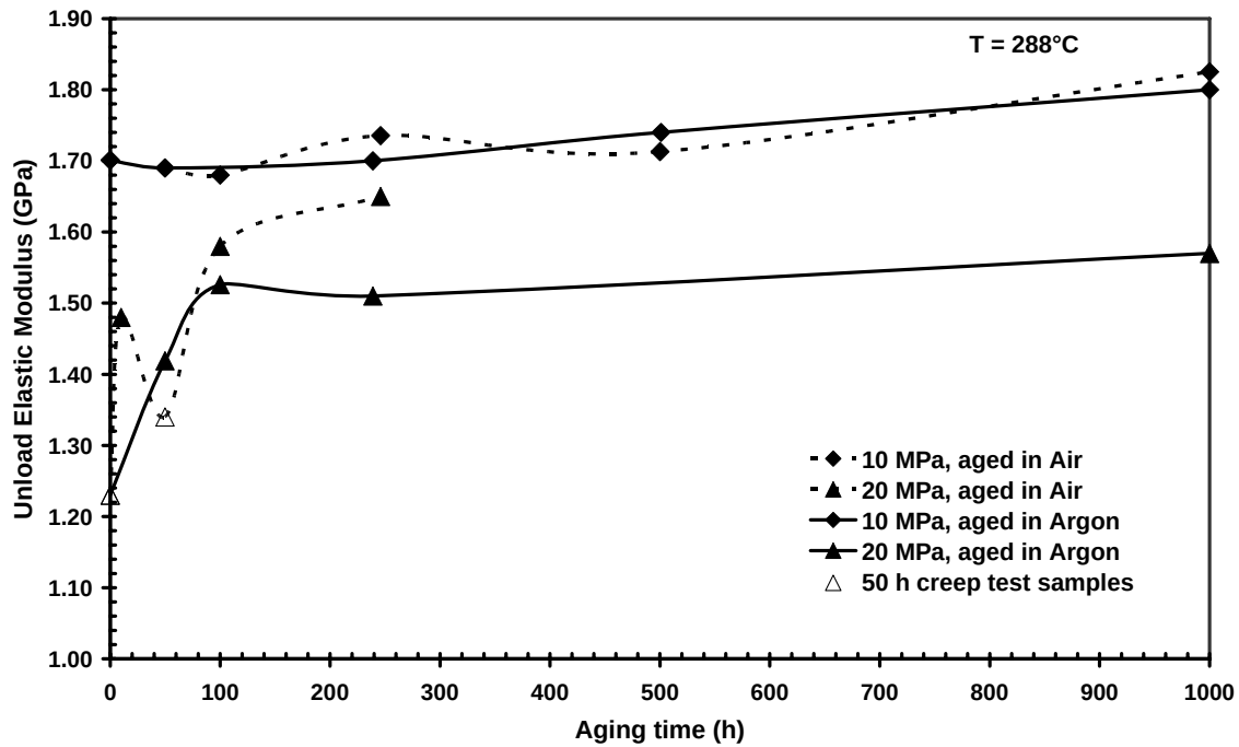
Figure 28 –Elastic modulus obtained upon unloading versus aging time in argon and in air at various creep stress levels. PMR-15 neat resin specimens tested at 288°C.
