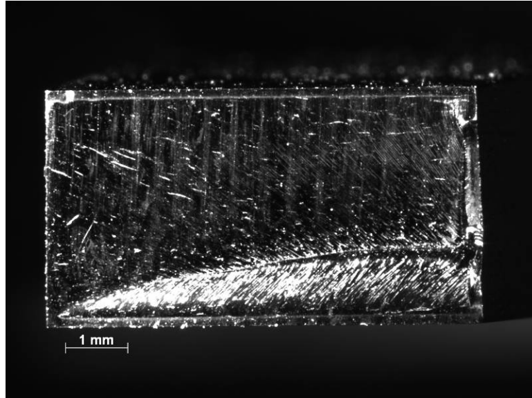
Figure 18 –Photograph showing the visible oxidation layer on the fracture surface of a PMR-15 neat resin sample aged for 1000 h at 288°C in air and tested in creep.
