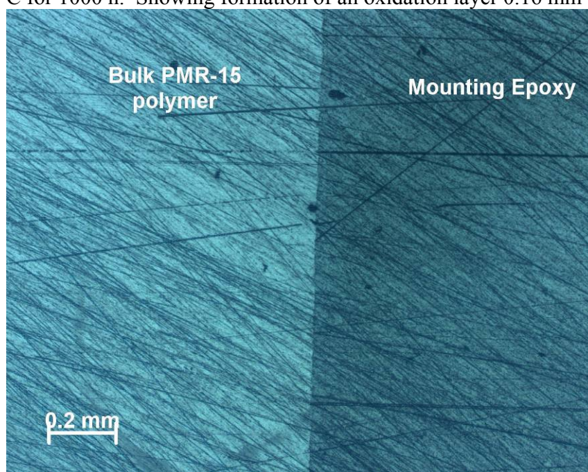
Figure 137 – Oxidation layer observed polished section of sample aged in argon at 288°C for 50 h. Showing absence of an oxidation layer.
