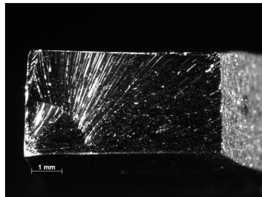
Figure 60 –Sample 10-01, PMR-15 neat resin aged in air for 10 h, T = 288°C, Creep stress = 20 MPa. Machined with water jet showing slight microcracking.
