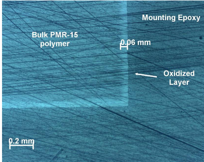
Figure 132 –Oxidation layer observed on polished section of sample aged in air at 288°C for 50 h. Showing formation of an oxidation layer 0.06 mm thick.
