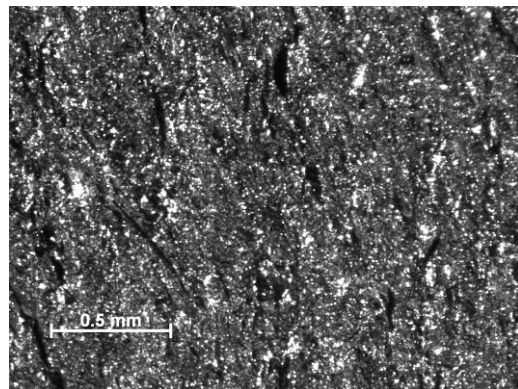
Figure 66 – Sample 13-12, PMR-15 neat resin aged in air for 50 h, T = 288^{\circ}\text{C} , Creep stress = 20 MPa. Machined with water jet showing slight microcracking.
