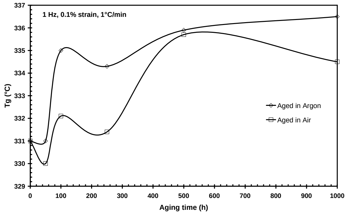
Figure 50 – Glass transition temperature versus prior aging time for specimens aged at 288°C in air or argon as determined by the transition of the storage modulus. T_g increased moderately with increasing prior aging time in air or argon at 288°C
