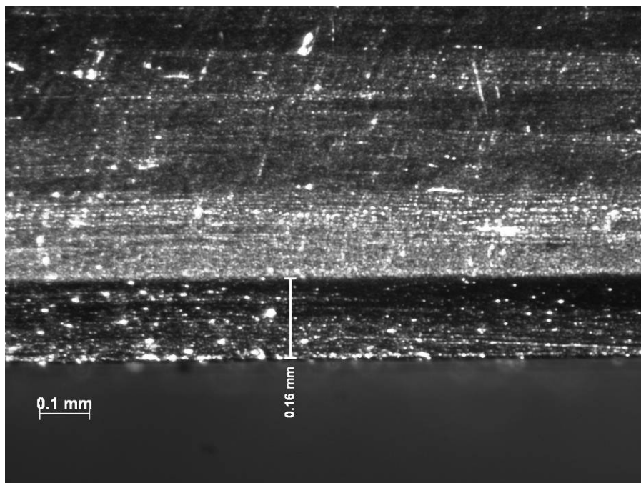
Figure 131 – Oxidation layer observed on fracture surface of sample aged in air at 288°C for 1000 h. Showing formation of an oxidation layer 0.16 mm thick.
