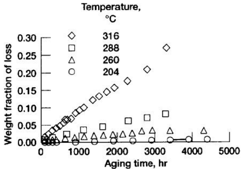
Figure 3 - Weight fraction loss as a function of aging time in air for PMR-15 neat resin. Figure from Ref. [3].
