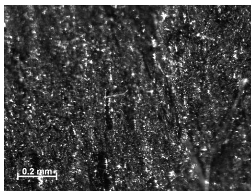
Figure 110 –Sample 13-04, PMR-15 neat resin aged in argon for 250 h, T = 288^{\circ}\text{C} , Creep stress = 20 MPa. Machined with water jet showing slight microcracking.
