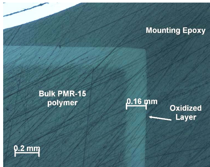
Figure 16 –Optical micrograph showing the oxidation layer on outer surface of PMR-15 neat resin sample aged for 1000 h at 288°C in air.
