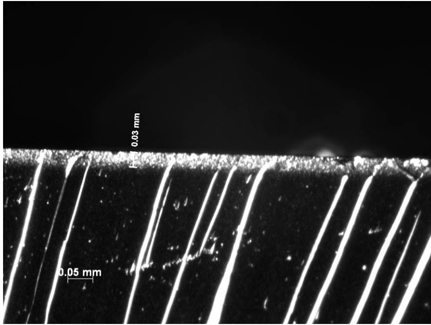
Figure 127 –Oxidation layer observed on fracture surface of sample aged in air at 288°C for 10 h. Showing formation of an oxidation layer 0.03 mm thick.
