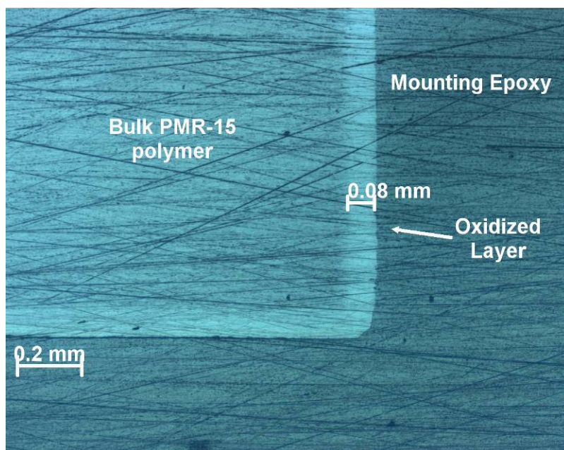
Figure 134 – Oxidation layer observed on polished section of sample aged in air at 288°C for 250 h. Showing formation of an oxidation layer 0.08 mm thick.
