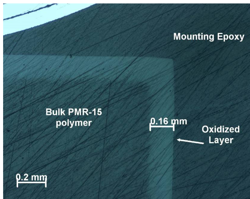
Figure 136 – Oxidation layer observed on polished section of sample aged in air at 288°C for 1000 h. Showing formation of an oxidation layer 0.16 mm thick.
