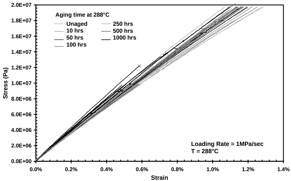
Figure 26 – Tensile stress-strain curves during loading obtained in all tests at 288°C showing qualitatively similar stress-strain behavior. An X indicates a sample fracture.
