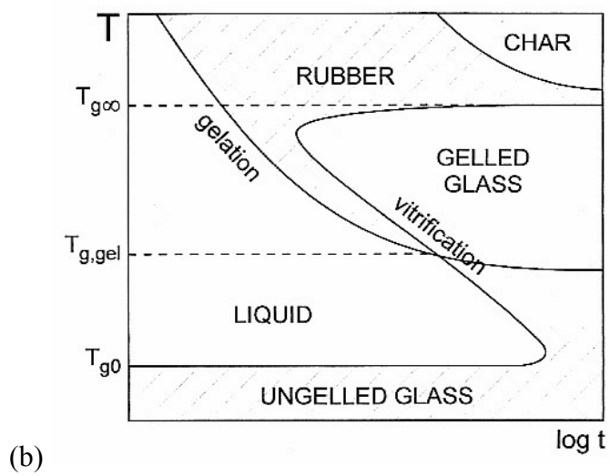
Figure 11 – (a) CTT diagram for generic thermoset polymer, (b) TTT diagram for generic thermoset polymer. Figures from Ref. [20:139-143].
