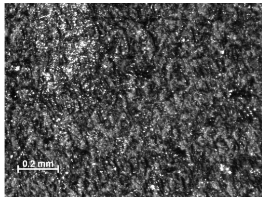
Figure 64 – Sample 11-05, PMR-15 neat resin aged in air for 10 h, T = 288^{\circ}\text{C} , Creep stress = 20 MPa. Machined with diamond saw.
