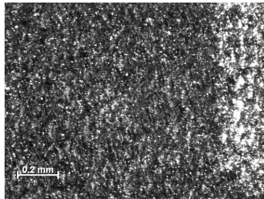
Figure 56 –Sample 02-08, as-processed PMR-15 neat resin, Creep stress = 15 MPa. Machined with diamond saw.
