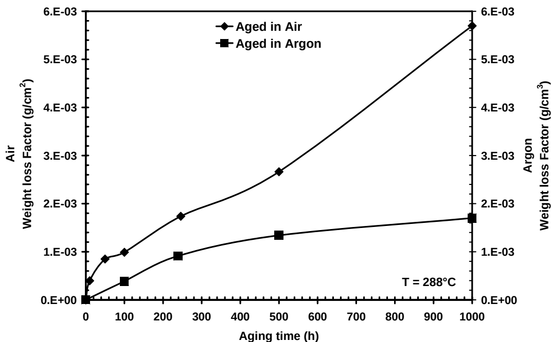
Figure 14 –Weight loss factor as a function of aging time for PMR-15 neat resin at 288°C in air and in argon.
