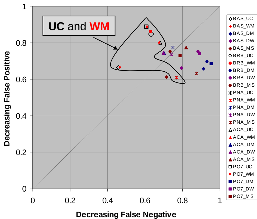
Figure B-7. Comparisons of 250 ppt Threshold-Based MOE Values for 25 Sets of Urban HPAC Predictions of JU03 Night Releases in the CBD – Five Modes (UC, WM, DM, DW, and MS) × Five MET Input Options (BAS, BRB, PNA, ACA, and PO7).
