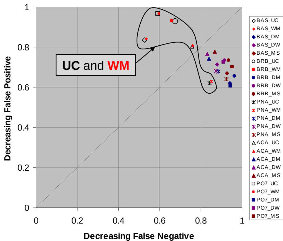
Figure B-3. Comparisons of 25 ppt Threshold-Based MOE Values for 25 Sets of Urban HPAC Predictions of JU03 Night Releases in the CBD – Five Modes (UC, WM, DM, DW, and MS) × Five MET Input Options (BAS, BRB, PNA, ACA, and PO7).
