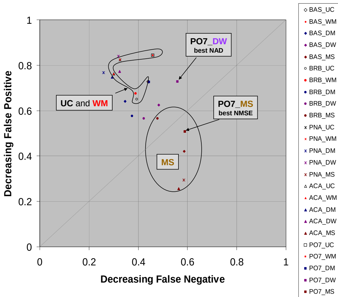
Figure B-9. Comparisons of Concentration-Based MOE Values for 25 Sets of Urban HPAC Predictions of JU03 Day Releases in the CBD – Five Modes (UC, WM, DM, DW, and MS) × Five MET Input Options (BAS, BRB, PNA, ACA, and PO7).
