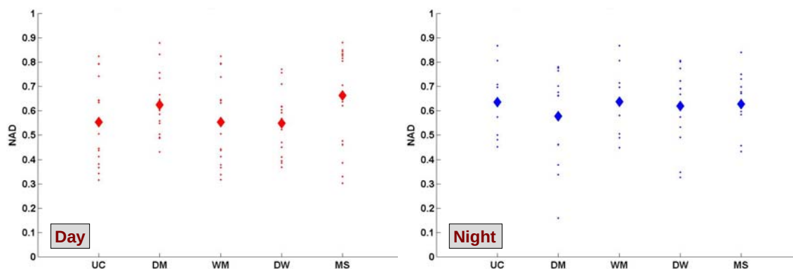
Figure 3-25. Comparisons of NAD Values for Urban HPAC Predictions of the 17 Daytime (left) and 12 Nighttime (right) Releases of JU03. These NAD values are for predictions of 30-minute average concentrations within the CBD using the PNA MET input option.
