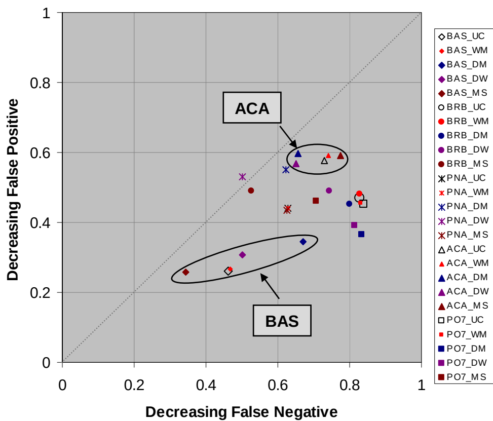
Figure B-8. Comparisons of 250 ppt Threshold-Based MOE Values for 25 Sets of Urban HPAC Predictions of JU03 Night Releases on the Arcs – Five Modes (UC, WM, DM, DW, and MS) × Five MET Input Options (BAS, BRB, PNA, ACA, and PO7).
