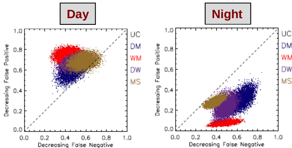
Figure 3-2. Comparisons of Concentration-Based MOE Values for Urban HPAC Predictions of the 17 Daytime (left) and 12 Nighttime (right) Releases of JU03. These MOE values are for predictions of 30-minute average concentrations on the arcs using the BAS MET input option.
