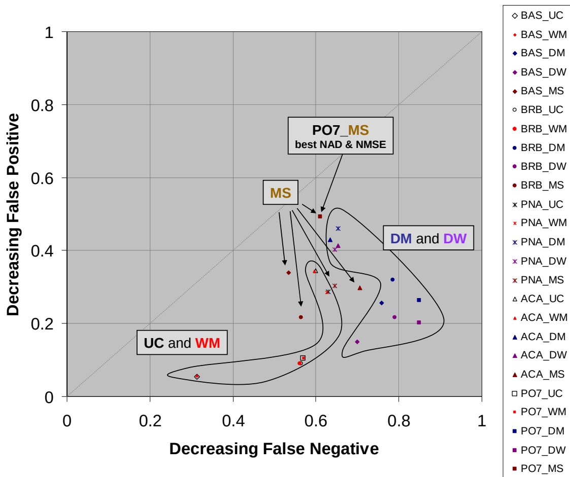
Figure B-11. Comparisons Concentration-Based MOE Values for 25 Sets of Urban HPAC Predictions of JU03 Night Releases in the CBD – Five Modes (UC, WM, DM, DW, and MS) × Five MET Input Options (BAS, BRB, PNA, ACA, and PO7).
