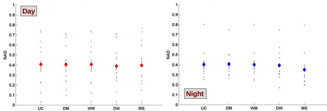
Figure 3-36. Comparisons of NAD Values for Urban HPAC Predictions of the 17 Daytime (left) and 12 Nighttime (right) Releases of JU03. These NAD values are for predictions of 30-minute average concentrations on the arcs using the ACA MET input option.
