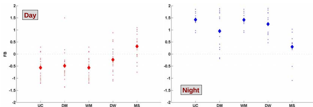
Figure 3-3. Comparisons of FB Values for Urban HPAC Predictions of the 17 Daytime (left) and 12 Nighttime (right) Releases of JU03. These FB values are for predictions of 30-minute average concentrations within the CBD using the BAS MET input option.
