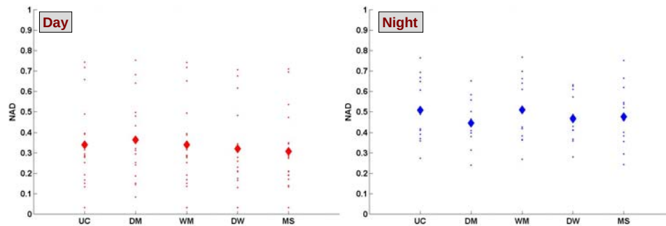
Figure 3-26. Comparisons of NAD Values for Urban HPAC Predictions of the 17 Daytime (left) and 12 Nighttime (right) Releases of JU03. These NAD values are for predictions of 30-minute average concentrations on the arcs using the PNA MET input option.
