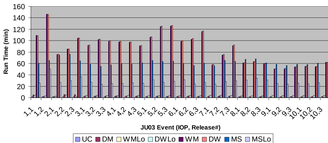
Figure 2-9. Run Times for Urban HPAC Predictions of 29 JU03 Releases Using Various Configurations and the PO7 Meteorological Input Option
