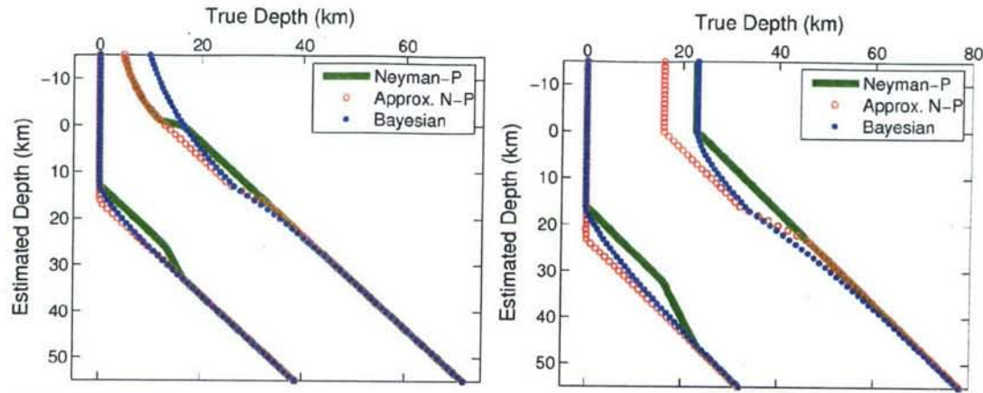
Figure 1. Confidence intervals on event depth in a fictitious problem involving a direct estimate of depth, which is either Gaussian (left panel) or Laplace (right) distributed, with a standard error of 10 km in each case. Three types of confidence limits (at \beta = 90\% ) are shown, each as a function of the depth estimate itself (vertical axis): exact N-P (green line), approximate N-P (red dots), and Bayesian (blue dots). The corresponding confidence interval is the range of true depth between these limits.
