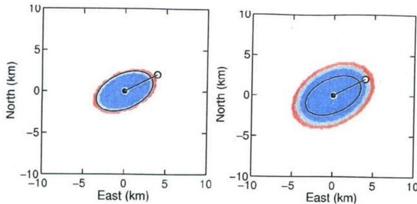
Figure 3. Epicenter confidence regions for a Pahute Mesa explosion with 6 Pn arrivals, computed with our two-step numerical algorithm. Left: Single-event confidence regions (path travel-time corrections assumed known). Right: Multiple-event confidence regions, treating a well-recorded Rainier Mesa event as a GT0 calibration event. Confidence regions are shown for 90%, 95%, and 98% confidence (blue, green, and red, respectively). In each frame the black circle marks the maximum-likelihood solution for the event location, and the white circle is its GT0 location (from Walter et al., 2003). The error distribution for picking errors was assumed to be Gaussian ( p = 2 ). The ellipse in each frame is the conventional 95% single-event confidence ellipse, computed analytically under the Gaussian/linear assumption.
