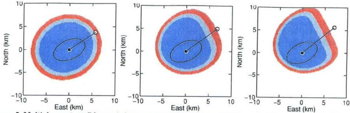
Figure 5. Multiple-event confidence regions computed with different GT5 constraints on the Rainier Mesa calibration event: generalized Gaussian orders p_0 = 2, 5 , and 20 (left, center, and right, respectively). The GT5 constraint is at 90% confidence in each case. The data errors are assumed to be Gaussian. The target event is the same as in previous figures.
