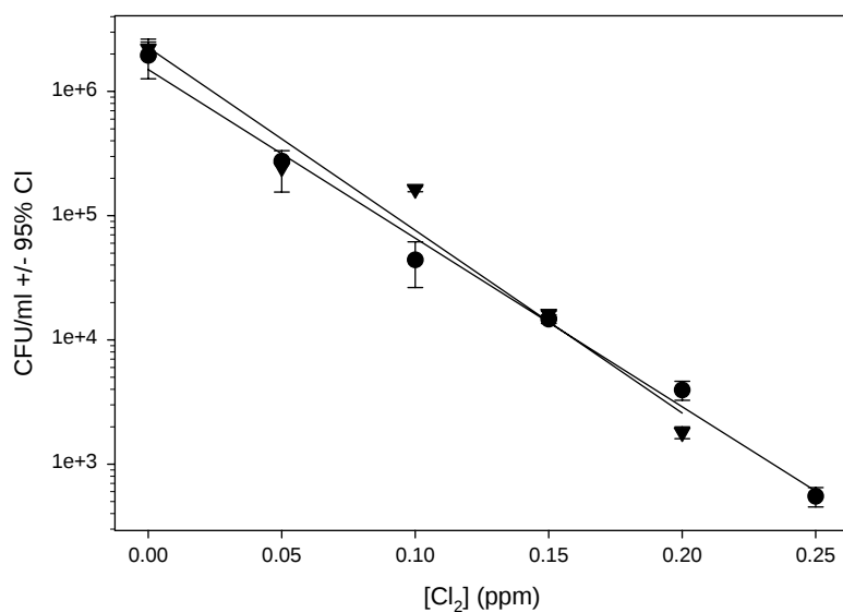
Figure 10. Survival of V. cholerae in synthetic seawater treated with ultrasound and dosed with total Cl 2 from 0-0.25 mg·l -1 . Ultrasound pre-treated (●, from Figure 9) and untreated (▼). All samples were quenched with sodium thiosulfate after 1 minute of Cl 2 exposure. The sample not treated by ultrasound and exposed to 0.25 mg·l -1 was less than 500 CFU/ml.
