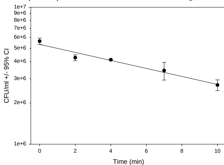
Figure 9. Survival of V. cholerae as a function of exposure time to low intensity (12 W·cm -2 ) ultrasound at low energy density (13 J·ml -1 ) in the beaker-scale system. The V. cholerae were subsequently exposed to chlorine (see Figure 10).
