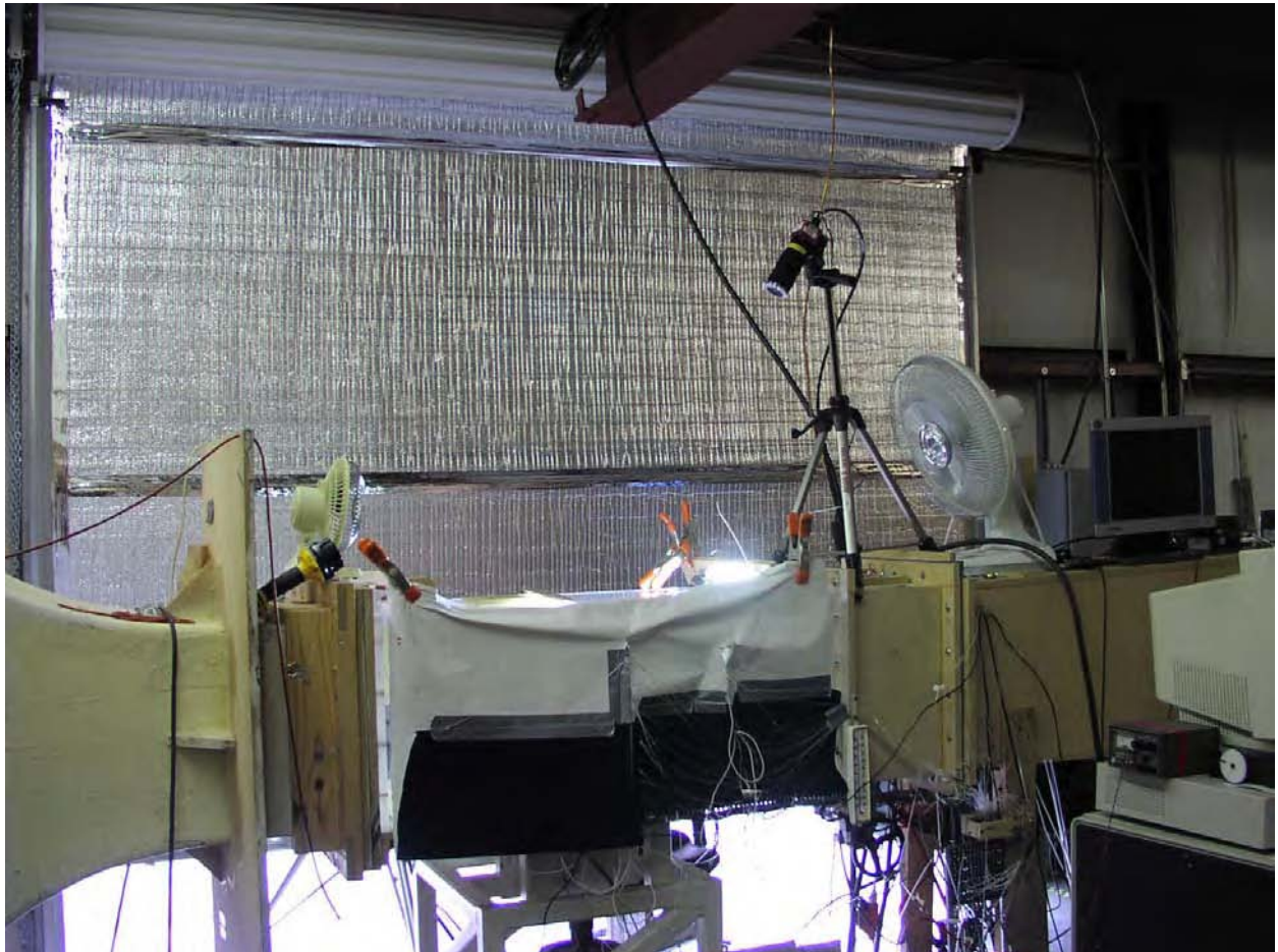
Figure 35. Displacement Camera Installation
