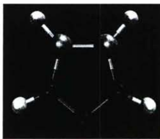
Figure 2b) 1,2,3-triazolium [123t]
