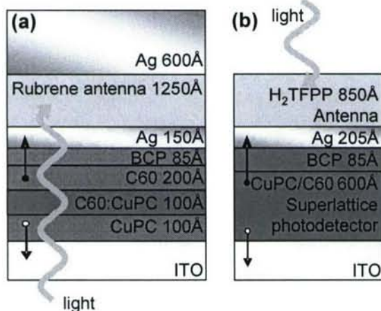
Fig. 4. (a) Devices with resonant antenna cavities have the structure: glass/ indium tin oxide (ITO) (1100 Å)/ copper phthalocyanine (CuPC) (100 Å)/ CuPC:fullerene (C60) (1:1) (100 Å)/ C60 (200 Å) / bathocuproine (BCP) (85 Å)/ Ag (150 Å)/ 30% Rubrene in CBP antenna (1250 Å) / Ag (600 Å). To quench or enhance the PL efficiency of the rubrene antenna we introduce either CuPC or DCJTb, respectively, at 2% weight ratio. Concentration quenching is minimized in the antenna by diluting rubrene with CBP. The devices are illuminated from the glass side. Organic materials were purified by vacuum thermal sublimation prior to use. All materials were deposited by thermal
