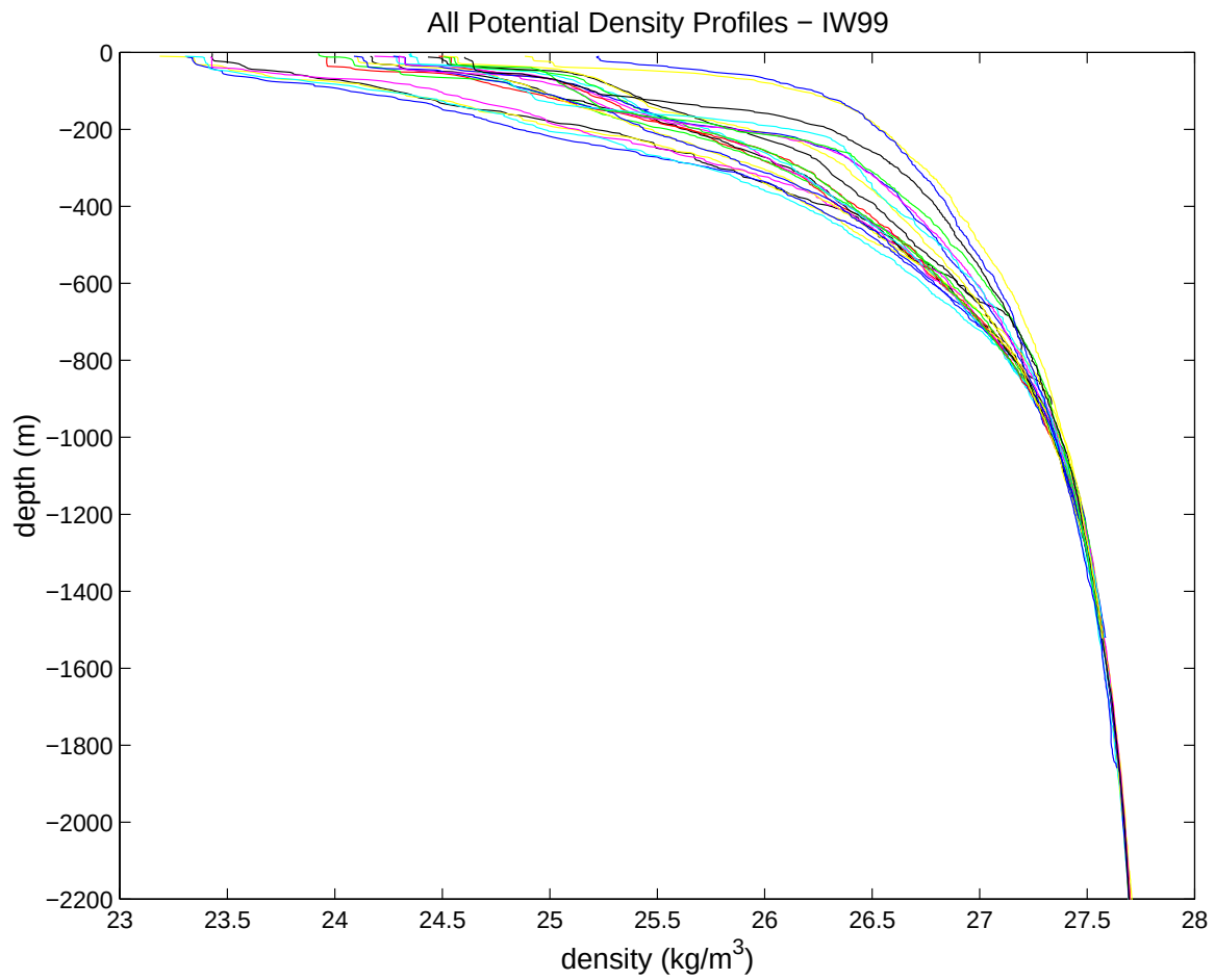
Figure 59. Potential density profiles, in \text{kg/m}^3 , from the IW99 cruise from the surface down to 2200 m.
