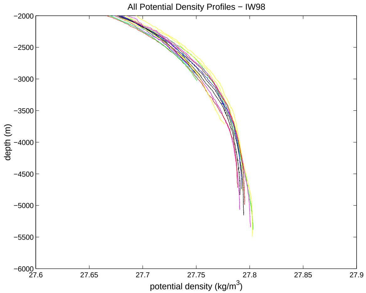
Figure 32. Potential density profiles, in kg/m 3 , from the IW98 cruise from 2000 m down to the ocean bottom.
