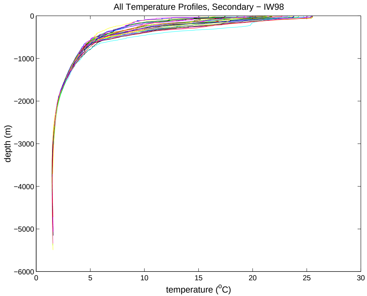
Figure 21. Temperature profiles from the secondary sensor on the IW98 cruise in ^{\circ}\text{C} .
