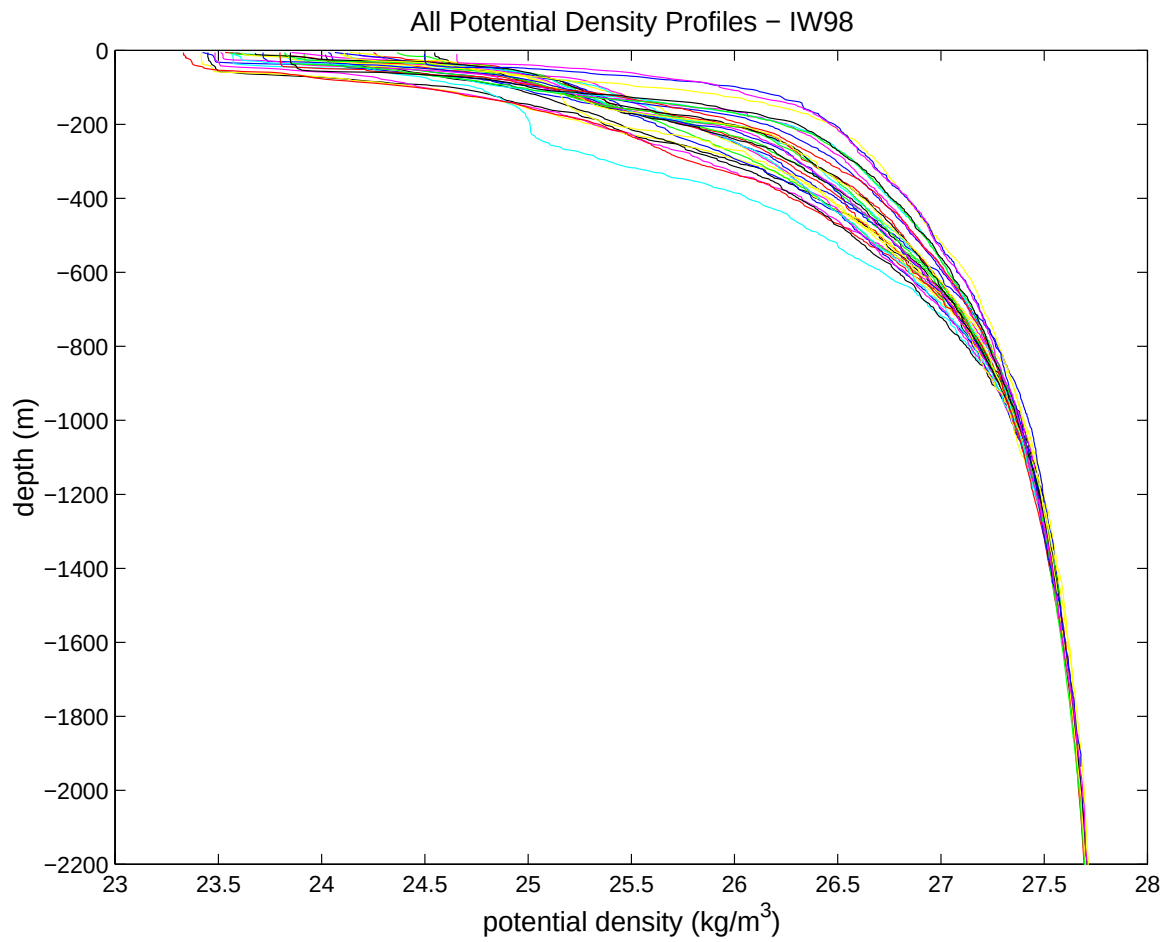
Figure 31. Potential density profiles, in kg/m 3 , from the IW98 cruise from the surface down to 2200 m.
