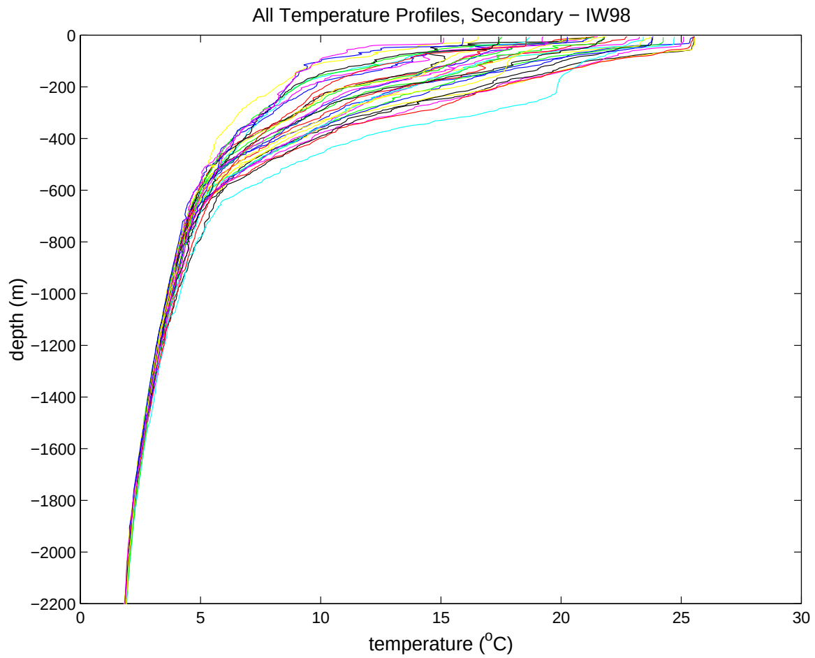
Figure 22. Temperature profiles from the secondary sensor on IW98, in °C, from the surface down to 2200 m.
