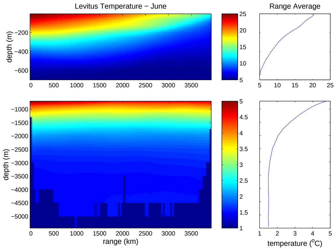
Figure 92. Same as in Figure 86, except for temperature in °C.
