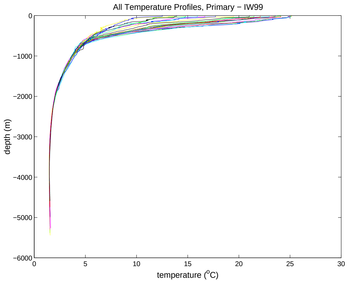
Figure 46. Temperature profiles from the primary sensor on the IW99 cruise in ^{\circ}\text{C} .
