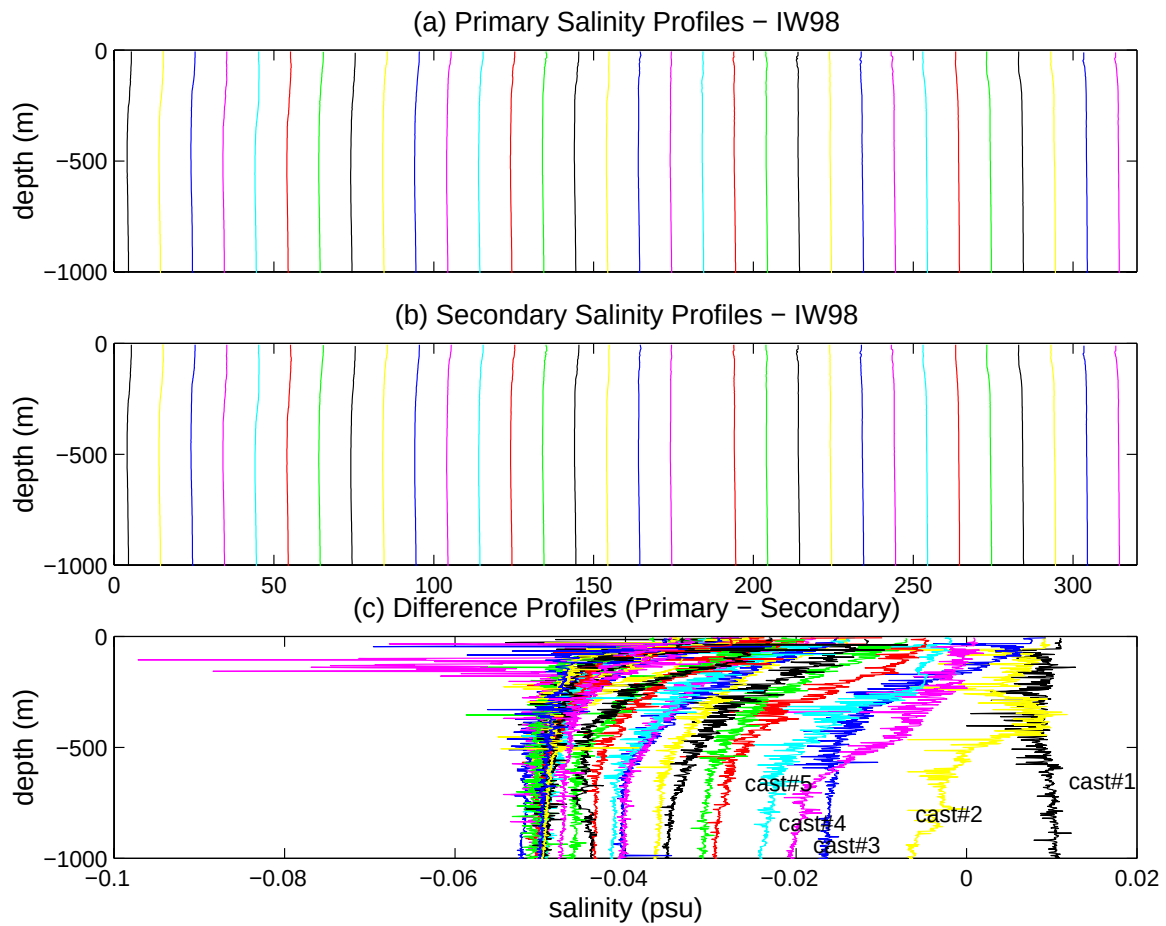
Figure 40. Same as Figure 39, except showing only the top 1000 m. The first five casts are labeled.
