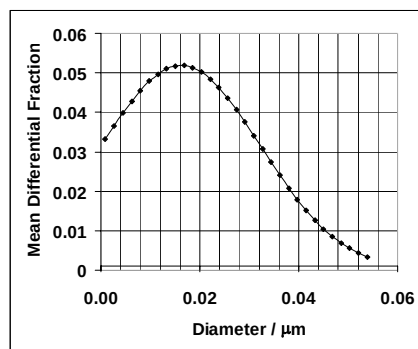
Figure 1: Average particle size distribution for the precursor YSZ powder.
