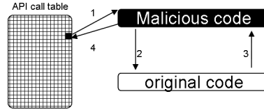
Figure 2.5: Hooking
