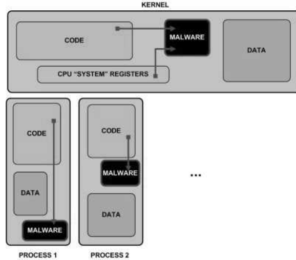
Figure 2.2: Type 1 Malware [18]
