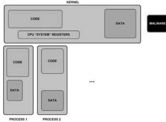
Figure 2.4: Type 3 Malware [18]
