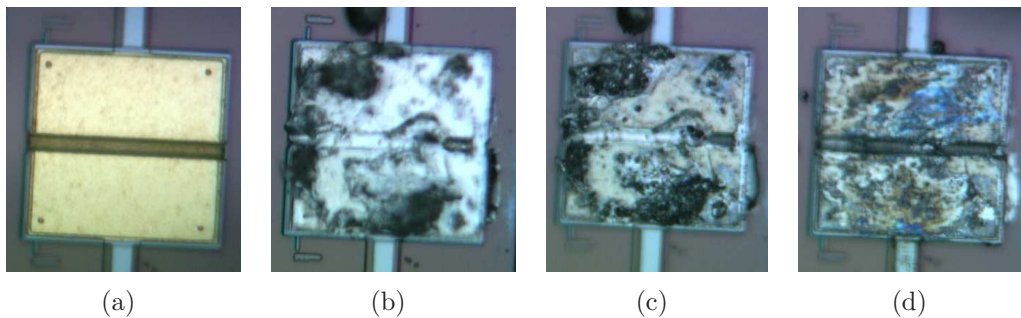
Figure 4.11: 270 °C solder powder test: (a) original contact pad prior to application of solder, (b) solder covers contact pad after initial application, (c) five minutes after solder application the solder pulls in and creates pools of solder leaving gold on contact exposed, (d) reapplied solder removing the previous solder with no new solder adhering to pad surface
