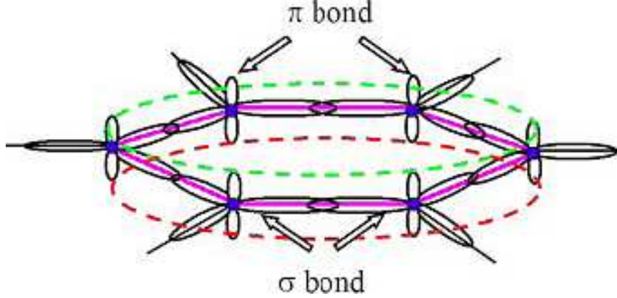
Figure 3.1: Vertical \pi bonds interconnect the graphene layers of carbon while the horizontal \sigma , covalent bonds, hold the graphene plane together [28].
