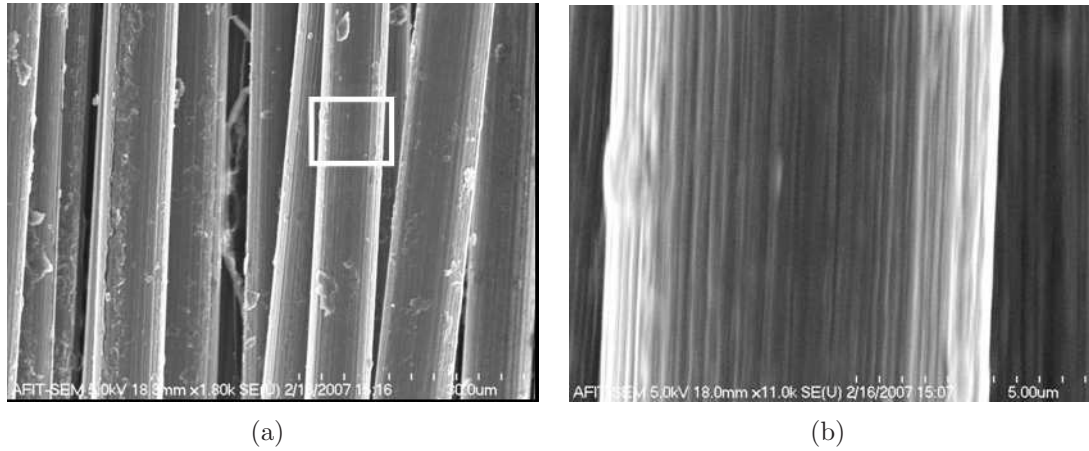
Figure 5.2: Base Thornel® P-100 fiber, F1, with heat treatment at 400 °C for 30 minutes to remove sizing, all subsequent fibers have this treatment. (a) Wide view of group of fibers, (b) image of individual fiber at 11k times view.
