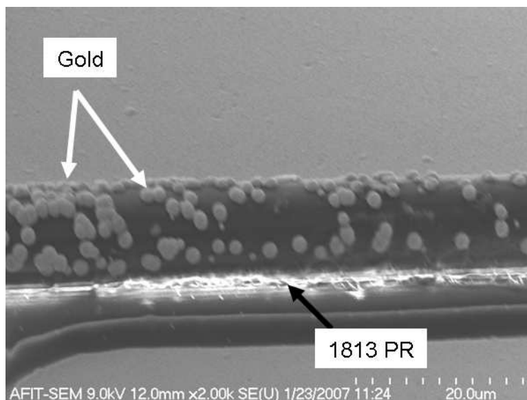
Figure 4.13: Gold electroplated fiber after approximately 1.5 hours of electroplating with 1813 PR trapped underneath
