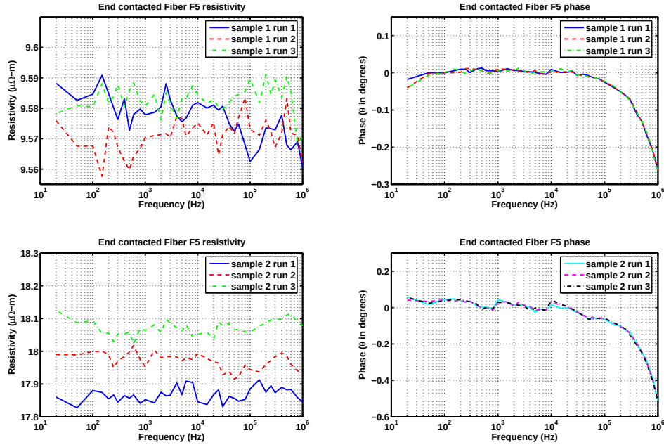
Figure 5.19: F5 samples 1 and 2, this data represents 2 fiber samples with the fiber ends covered with Epo-Tek® H-27D epoxy. The top two plots were from three runs for fiber F5 sample 1. The bottom two plots were from three runs for fiber F5 sample 2.
