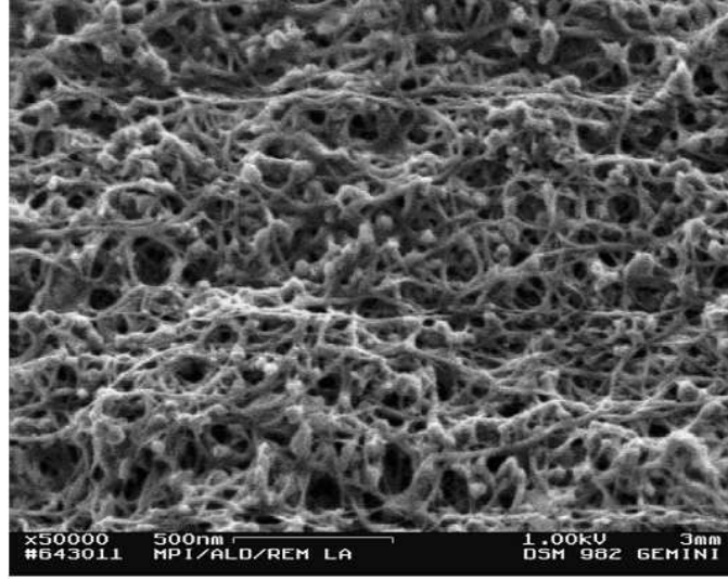
Figure 2.14: Surface of CNT sheet from scanning electron microscope [23].
