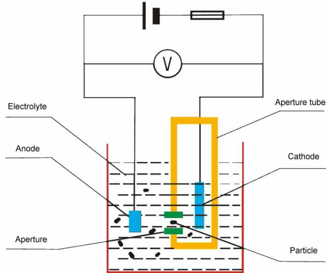
Figure 2.4 Diagram from pulvertechnology.com of a basic Coulter Counter. When voltage is applied across the electrodes, current flows from the anode to the cathode through a microscopic aperture. The particles in suspension are sensed by the current monitoring system because they increase the resistivity of the aperture as they pass through.
