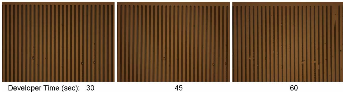
Figure 26. Line quality of 2 μm lines at a 10 μm period. The 30-second development shows slight roughness on the edges. The 45 second development shows better line quality, but the line width is slightly decreased due to the slow, unwanted development of the sidewalls. The 60-second development shows gaps where the LOR3A™ was undercut beneath the 1805.
