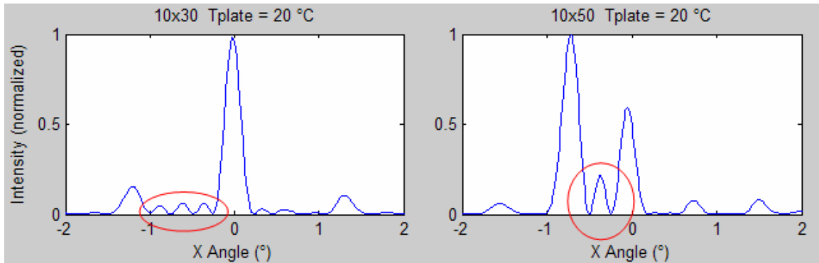
Figure 39. A side view of the 10x30 and 10x50 diffraction pattern across the y = 0^\circ line modeled at 20^\circ\text{C} . Three subsidiary maxima are shown between the zero and negative first orders for the 10x30 sample, and one for the 10x50. This correctly corresponds to the number of periods modeled for each (five and three).
