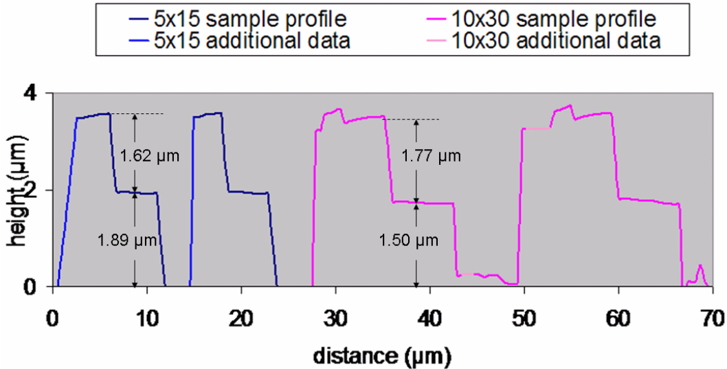
Figure 52. Step profile of 5x15 (blue) and 10x30 (magenta) samples fabricated using the alternative method. Because the Zygo® interferometer was not able to capture the entire profile at this small scale, the expected profile is added (lighter colors).
