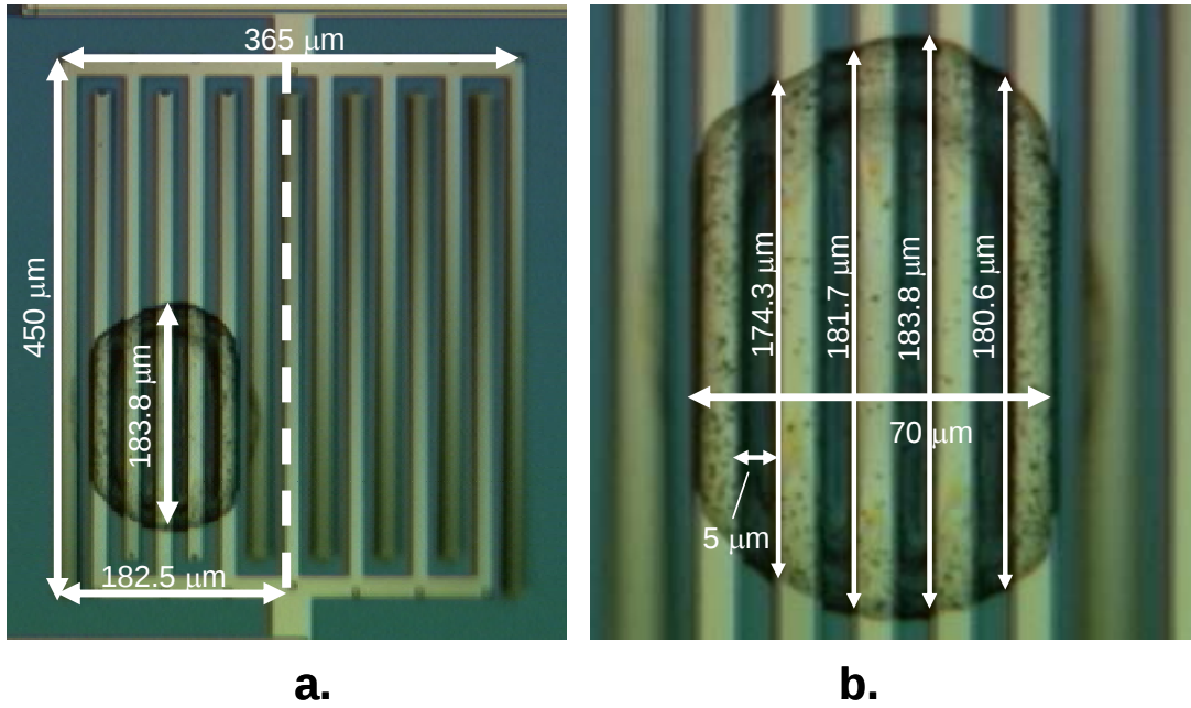
Figure 46: Two images taken by a microscope camera illustrating approximate dimensions of the inkjet deposited droplet (5 layers). This allows for calculating for both the surface area/cross-sectional area of the effective sensing region. a) Photo of the effective sensing area of the PIP with respect to the dimensions of the pixel. b) Magnified image of part a) that was measured using the software of the microscope camera.
