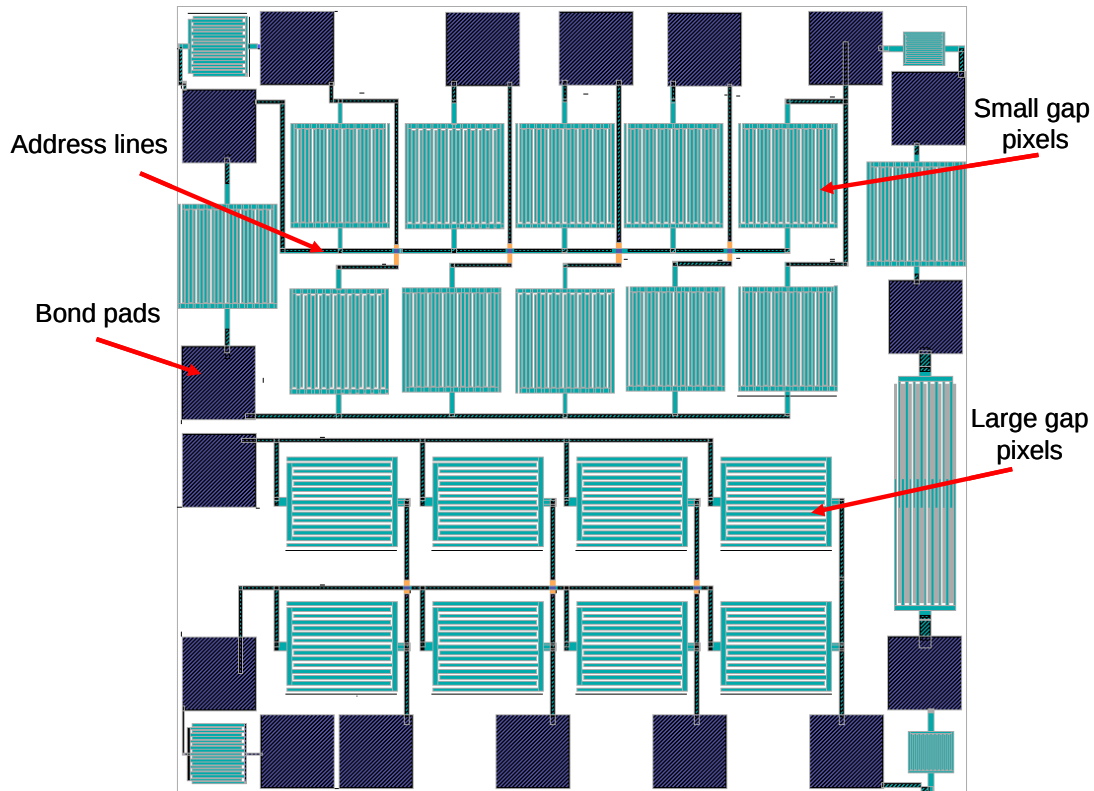
Figure 69: PolyMUMPs run 73.
