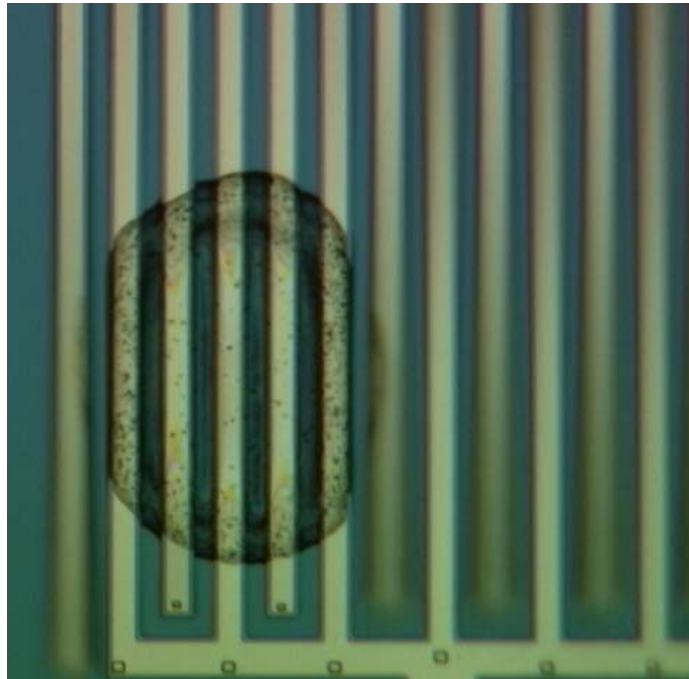
Figure 45: A microscope image illustrating how multiple layers cause the inderdigitized fingers to adhere to the underlying substrate, annulling thermal isolation. The image is out of focus where there is thermal isolation and in focus where the fingers are stuck to the substrate by the PIP material.
