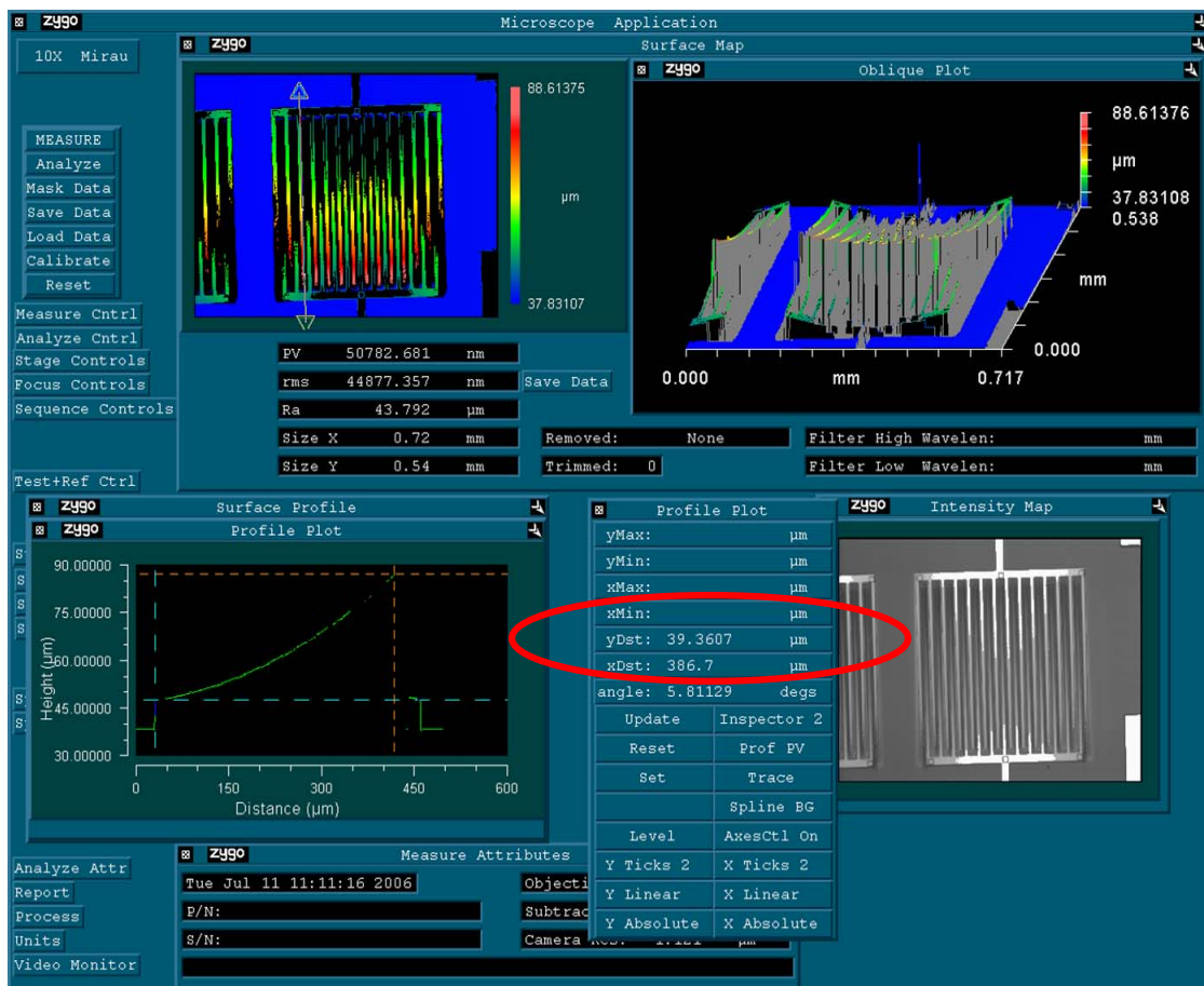
Figure 32: Image from Zygo's IFM that depicts deflection characteristics of pixel design. The max deflection is seen in the "yDst" parameter shows \sim 39.36 \mu\text{m} .
