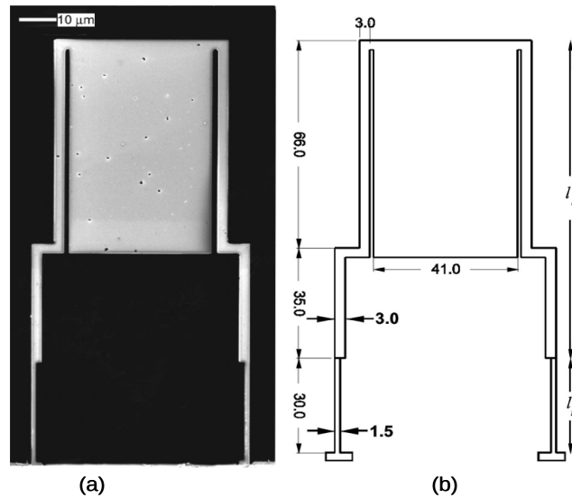
Figure 8: Microcantilever IR detector design. a) SEM image. b) Detector's dimensions in μm [9].
