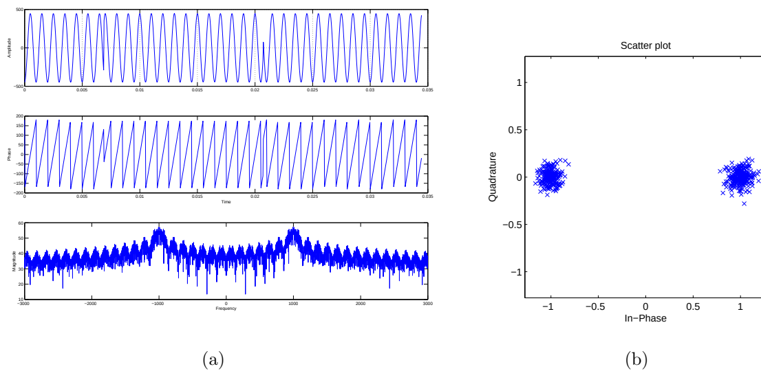
Figure 4.2: BPSK modulation (a) amplitude, phase, and spectrum representations. (b) scatter plot.
