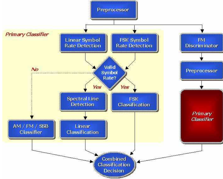
Figure 2.8: Flow Chart of the CuHBC algorithm.
