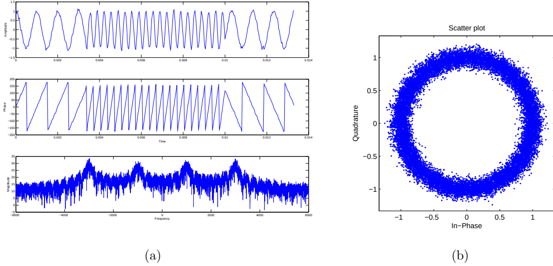
Figure 4.6: FSK2 modulation (a) amplitude, phase, and spectrum representations. (b) scatter plot.
