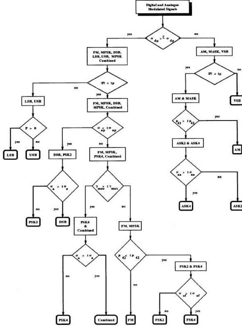
Figure 2.6: Flow Chart of Azzouz and Nandy algorithm.
