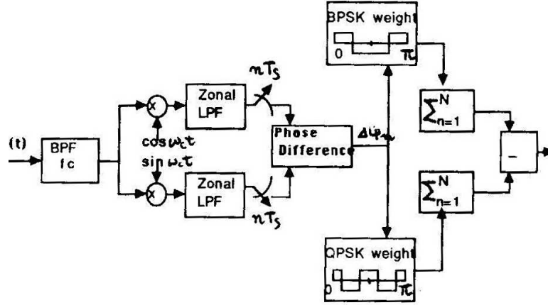
Fig.1 A phase-based BPSK/QPSK classifier structure
