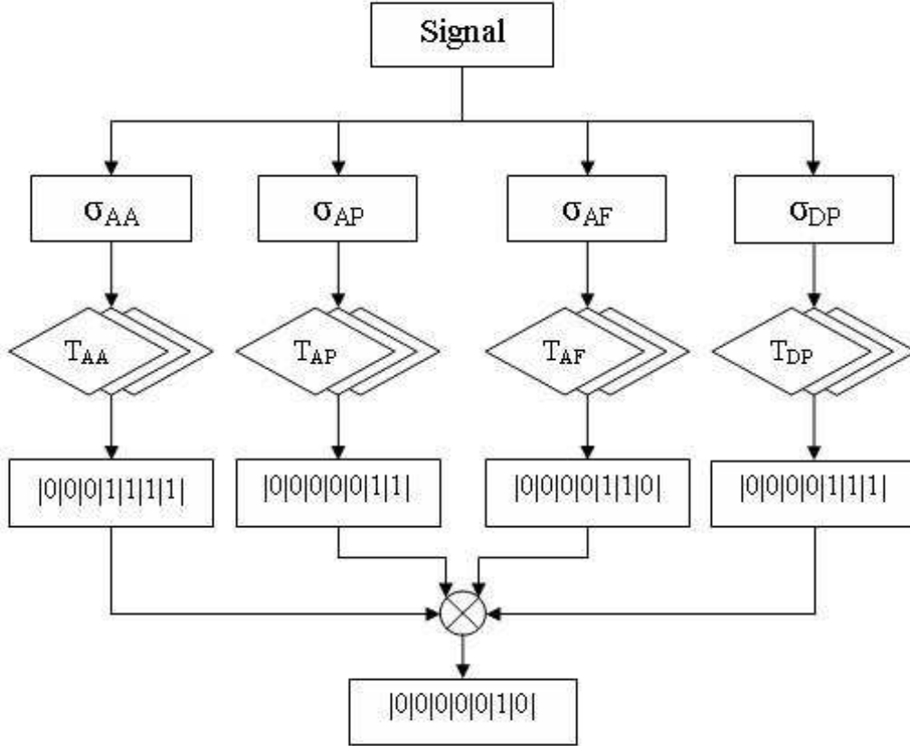
Figure 4.24: Diagram of the SNR estimation method. Each of the four features is input to a distinct branching tree ( T ) which then produces a (1x7) vector of ones and zeros corresponding to the seven SNR regions. The ones indicate that the given feature value is within the region, the zeros indicate the opposite. Multiplying the four output vectors of the four branching trees produces the desired overlap. The Matlab ® code for each of the four branching trees is provided in Appendix 2.
