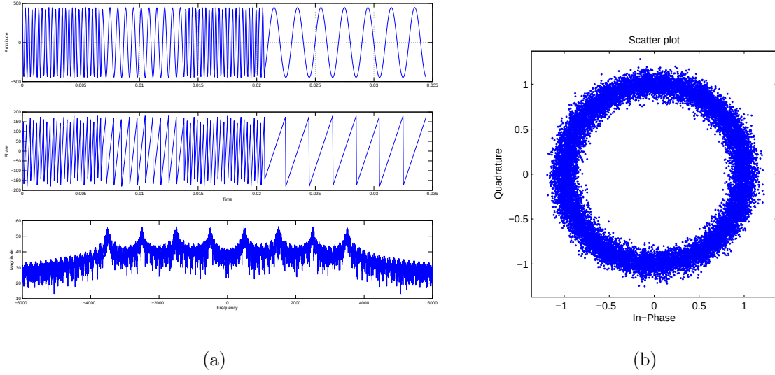
Figure 4.7: FSK4 modulation (a) amplitude, phase, and spectrum representations. (b) scatter plot.
