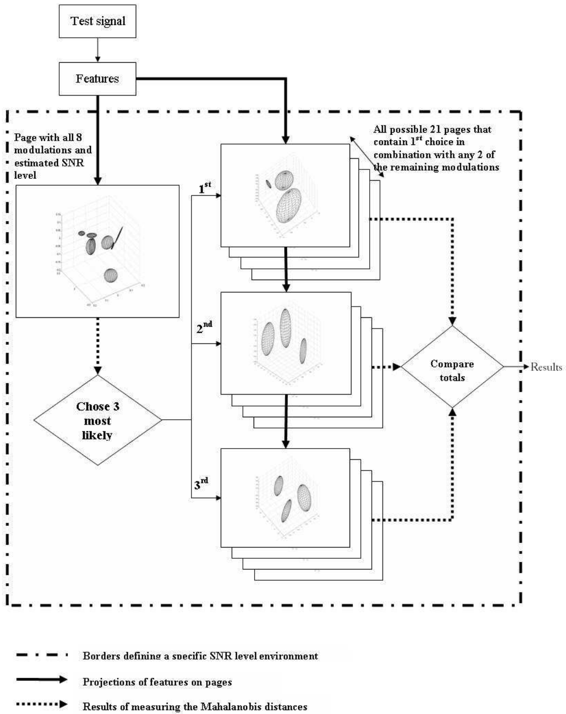
Figure 4.18: Flow diagram of classification of a test signal as performed in a fixed SNR level environment.
