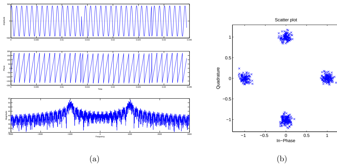
Figure 4.3: QPSK modulation (a) amplitude, phase, and spectrum representations. (b) scatter plot.
