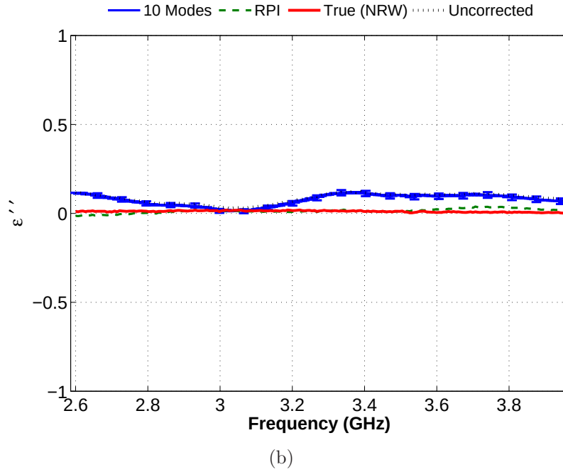
Figure 5.4: Permittivity of FGM-125 in a PFW with 27 mil top air gap. A 10 mode solution overcorrects the (a) real part, and yields an exact match between 3 and 3.1 GHz for the (b) imaginary part. The inclusion of RPI is within the error bounds in (a), but gives superior performance in (b). Error bars indicate \pm 2 mil uncertainty in height and thickness.
