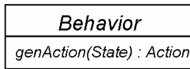
Figure 4.2: Defining an abstract class allows behavior logic to be encapsulated as independent and interchangeable objects that conform to a standard interface.
