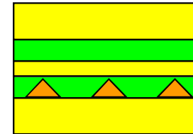
Double QW with buried QDs
