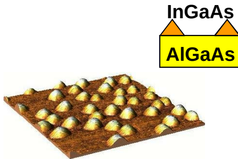
Self-Assembled QDs
