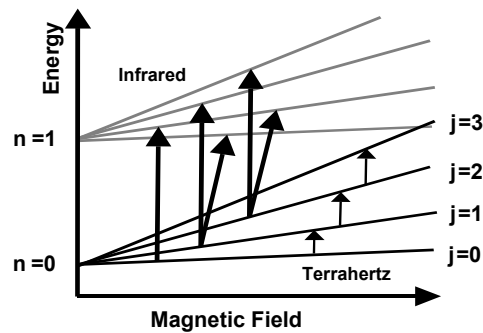
Figure 6: Calculations for a magnetic field parallel to the quantum well growth direction. The “n” states are quantum well electronic states; the “j” states are magnetic Landau states.
