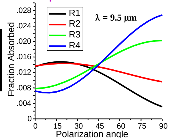
Response To Linear Polarization
