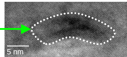
TEM enlargement of quantum dot
