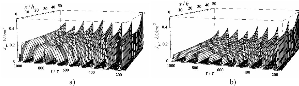
Fig.3. Drift and recombination of holes inside i -region of GaAs SPEM:
