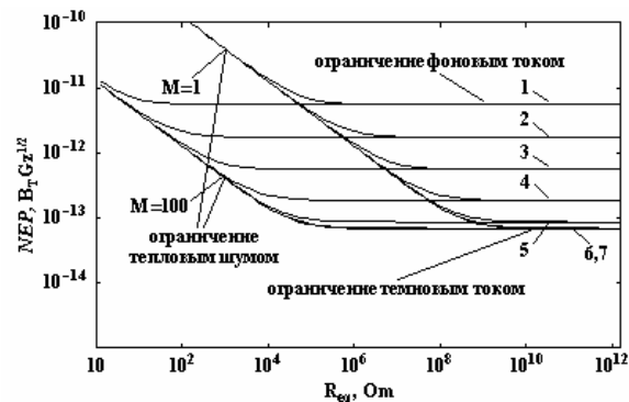
Fig.7. NEP dependencies on the load resistance for various amplification coefficients M ( F(M)=6 ), background current I_B (curve 1- I_B=10^{-6} ; 2- I_B=10^{-7} ; 3- I_B=10^{-8} ; 4- I_B=10^{-9} ; 5- I_B=10^{-10} ; 6- I_B=10^{-11} ; 7- I_B=10^{-12} A) and constant dark current I_D=1.5 \cdot 10^{-10} A.
