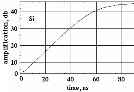
Fig.2. Dependence of the amplification coefficient inside SPEM as function of amplifying time.
