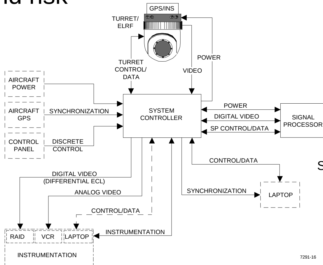
System Controller
