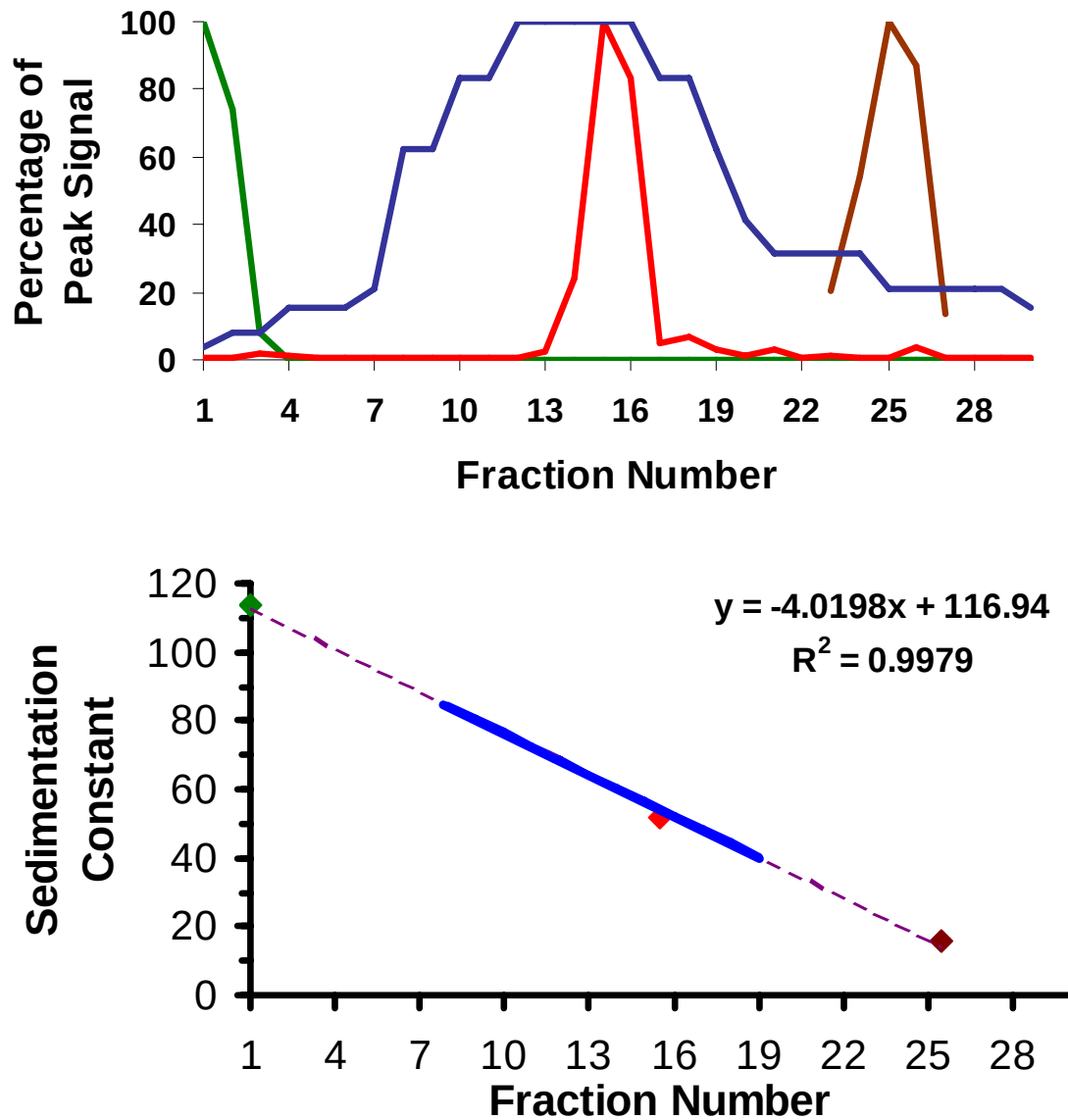
Figure 2. \text{PrP}^{\text{res}} was predominantly found in fractions 8-19, with a broad peak between fractions 12-16, corresponding to 50 to 70 Svedbergs (S). The marker particles with known constants were found in the following fractions: PhiX174, 114 S, fractions 1 and 2; PCV1, 52 S, fractions 15 and 16; Apoferritin, 18 S, fraction 26. In the top plot, each marker is plotted as a percentage of its own peak signal so that they are all normalized to a peak height of 100%. The bottom figure shows a standard curve generated by plotting the marker particles' positions, which allowed us to interpolate the sedimentation constant range of \text{PrP}^{\text{res}} . When infectivity data becomes available, it will be added to these plots.
