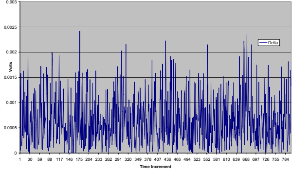
Pitch-Catch (5 to 4): 155kHz (Damage #3 Average - 30 Jan Damage #4) Delta
