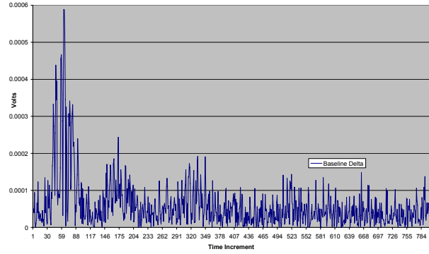
Pulse-Echo (0072): 95kHz (No Damage Average - 10 Nov Block 1) Delta
