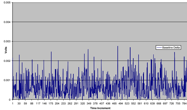
Pitch-Catch (5 to 4): 95kHz (Damage #12 Average - 11 Feb Damage #13) Delta
