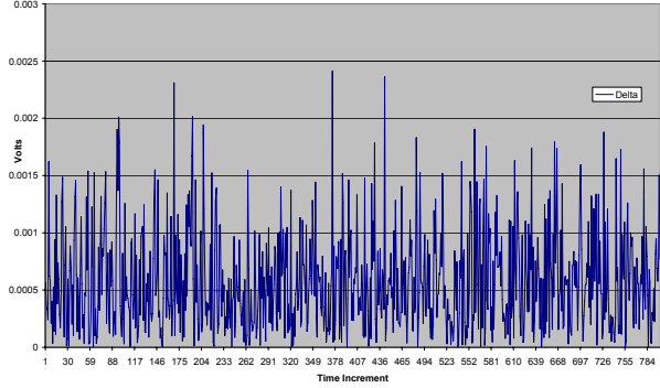
Pitch-Catch (5 to 4): 155kHz (Damage #7 Average - 02 Feb Damage #8) Delta
