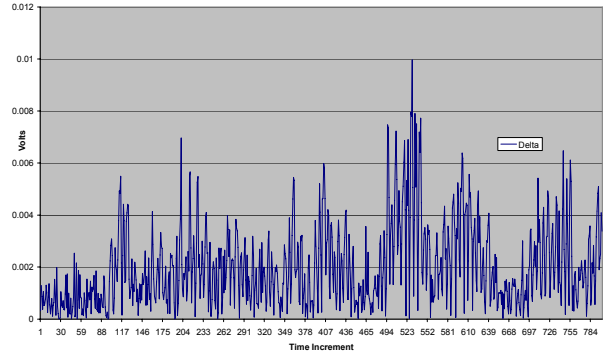
Pitch-Catch (5 to 4): 95kHz (No Damage Average - 16 Jan Block 7 Offset) Delta
