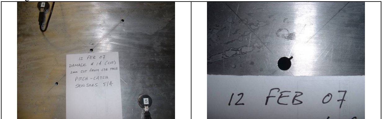
Pitch-Catch (Sensor 5 to 4): 12 Feb 07, Damage 14 – 2mm Cut from Center Hole Damage 13 Baseline
