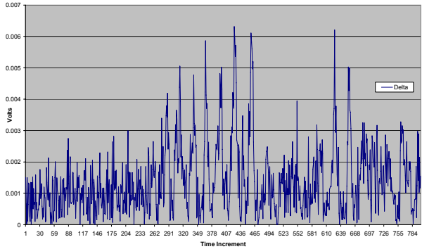
Pitch-Catch (5 to 4): 35kHz (Damage #4 Average - 30 Jan Damage #5) Delta
