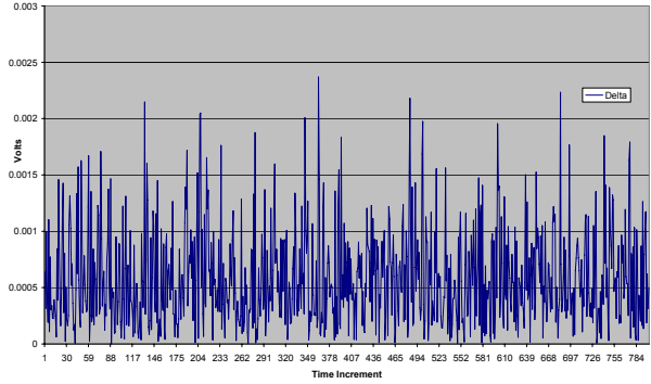
Pitch-Catch (5 to 4): 155kHz (Damage #7 Average - 03 Feb Damage #8) Delta
