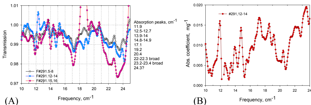
Figure 2: (A) A comparison of three experiment results on BG cell aerosols, (B) Estimated absorption coefficient of BG cell aerosol, \alpha/c , with a concentration less than 5 \cdot 10^{-3} mg/ml.
