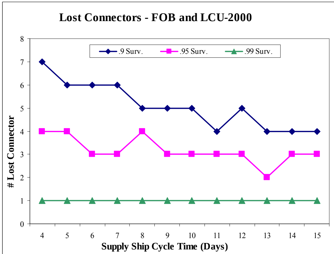
Figure 137. Lost Connectors using FOB and LCU-2000 configuration as a function of supply ship cycle time.
