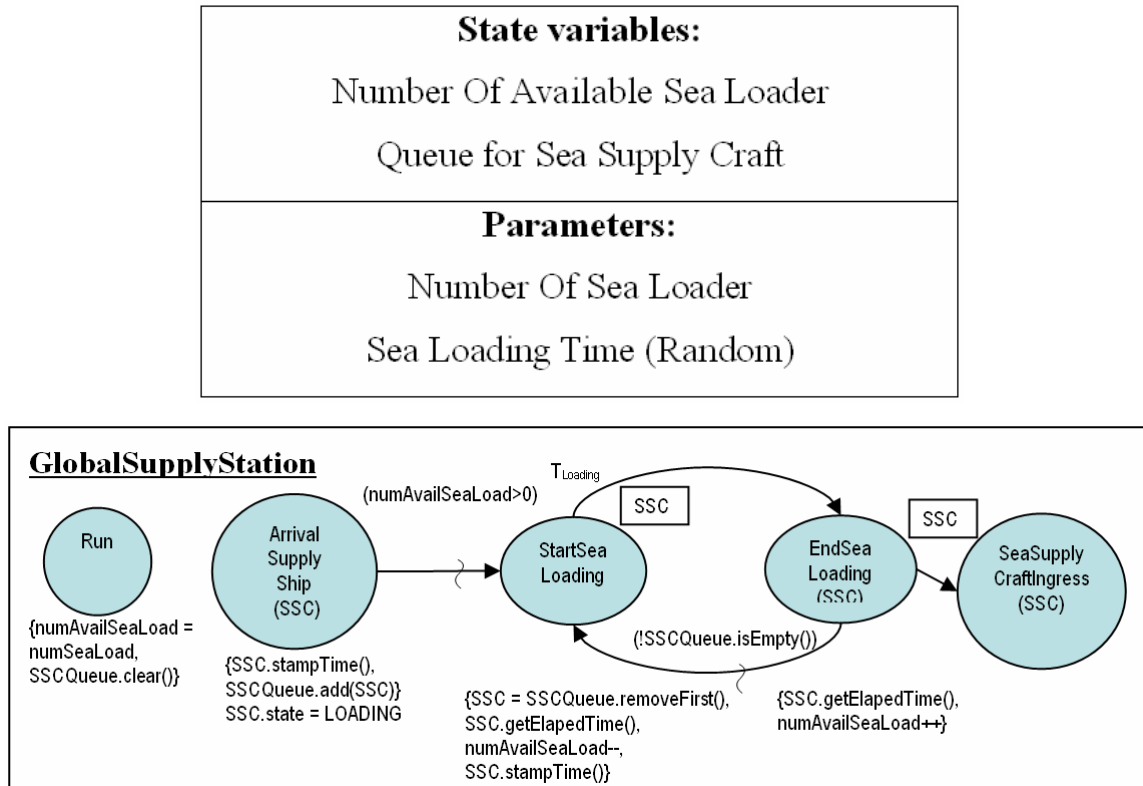
Figure 97. Event Graph for SupplyStation Object
