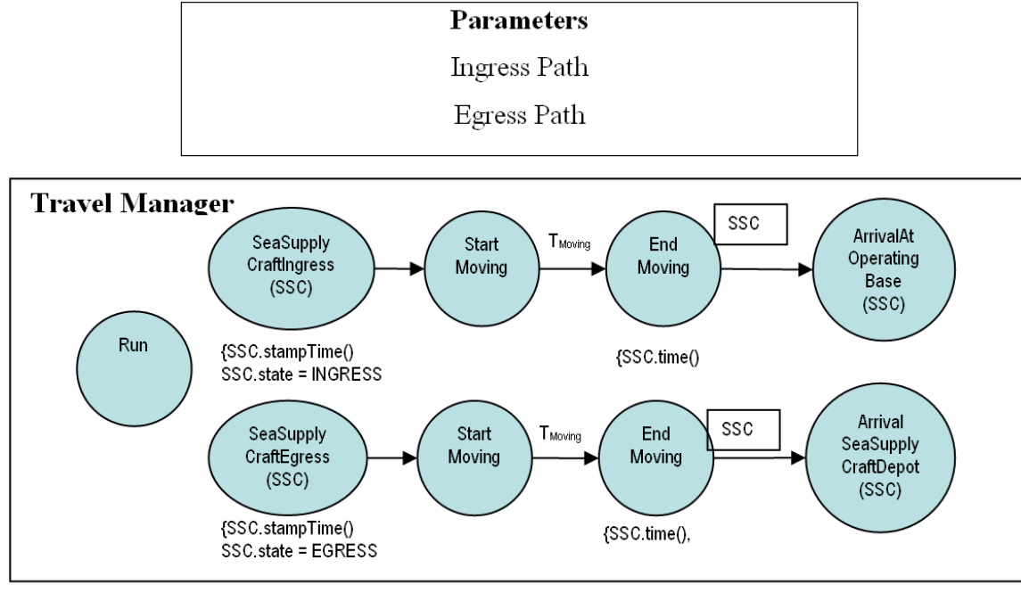
Figure 98. Event Graph for TravelManager Object
