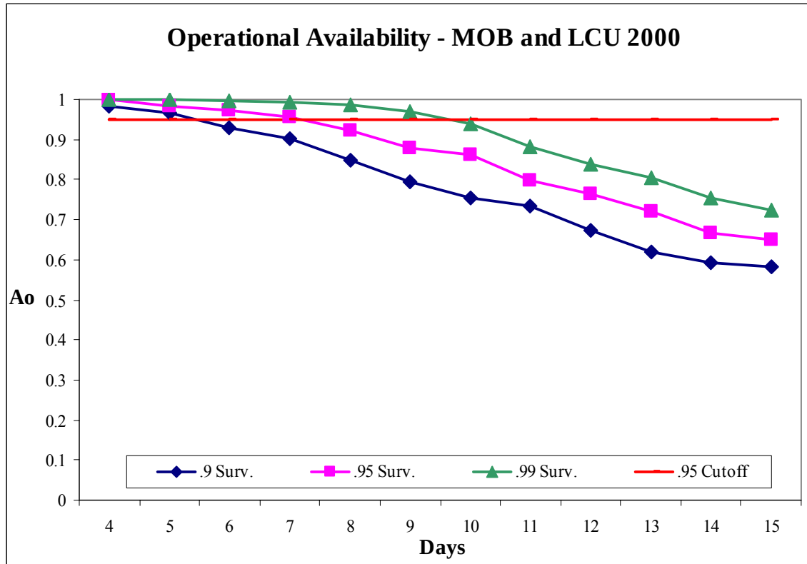
Figure 131. A_o fuel SURC for MOB and LCU-2000
