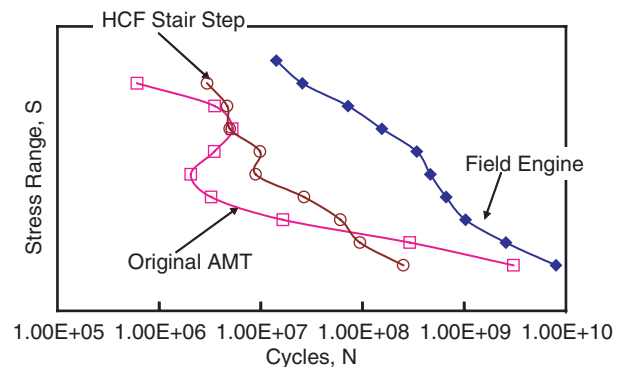
Figure 11. Comparison of Field Engine, AMT, and HCF Stair-Step Load Spectra
