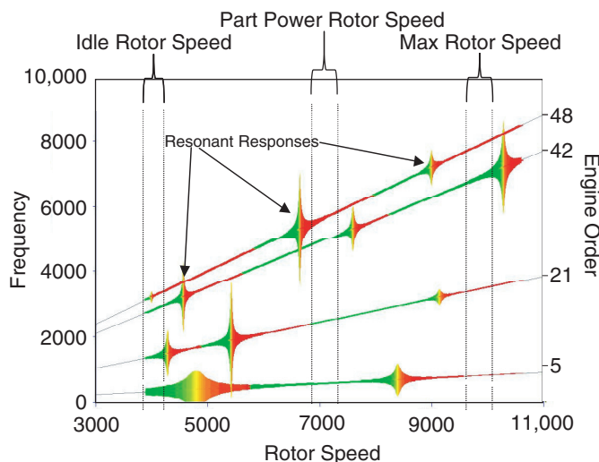
Figure 4. Campbell Diagram with AMT Speed Ranges
