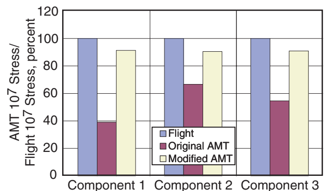
Figure 15. Comparison of 10^7 Stress Range for AMT and Flight
