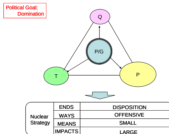
Figure 3. Cuban-crisis NS Model
