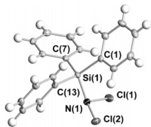
Figure 1. Structure of the \text{Ph}_3\text{SiNCl}_2 molecule. Thermal ellipsoids are shown at the 50% probability level.
