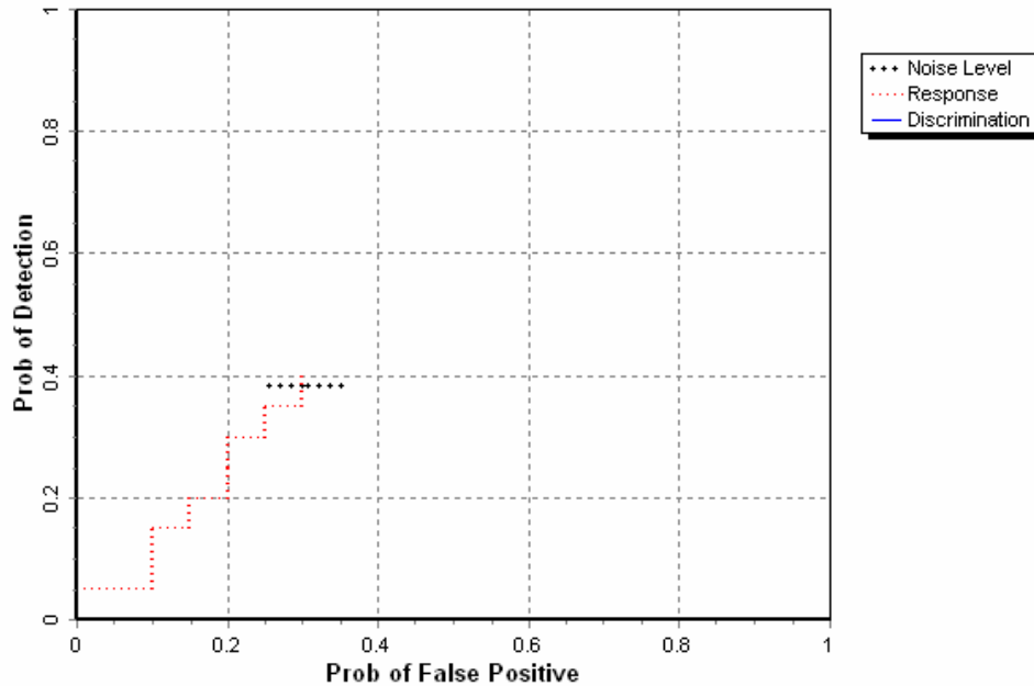
Figure 2. FEREX fluxgate gradient MAG/sling blind grid probability of detection for response and discrimination stages versus their respective probability of false positive over all ordnance categories combined.
