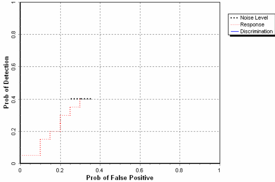
Figure 4. FEREX fluxgate gradient MAG/sling blind grid probability of detection for response and discrimination stages versus their respective probability of false positive for all ordnance larger than 20 mm.
