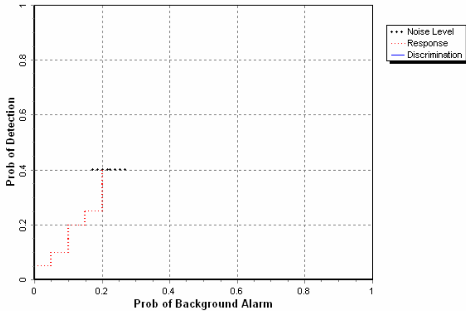
Figure 5. FEREX fluxgate gradient MAG/sling blind grid probability of detection for response and discrimination stages versus their respective probabilities of background alarm for all ordnance larger than 20 mm.
