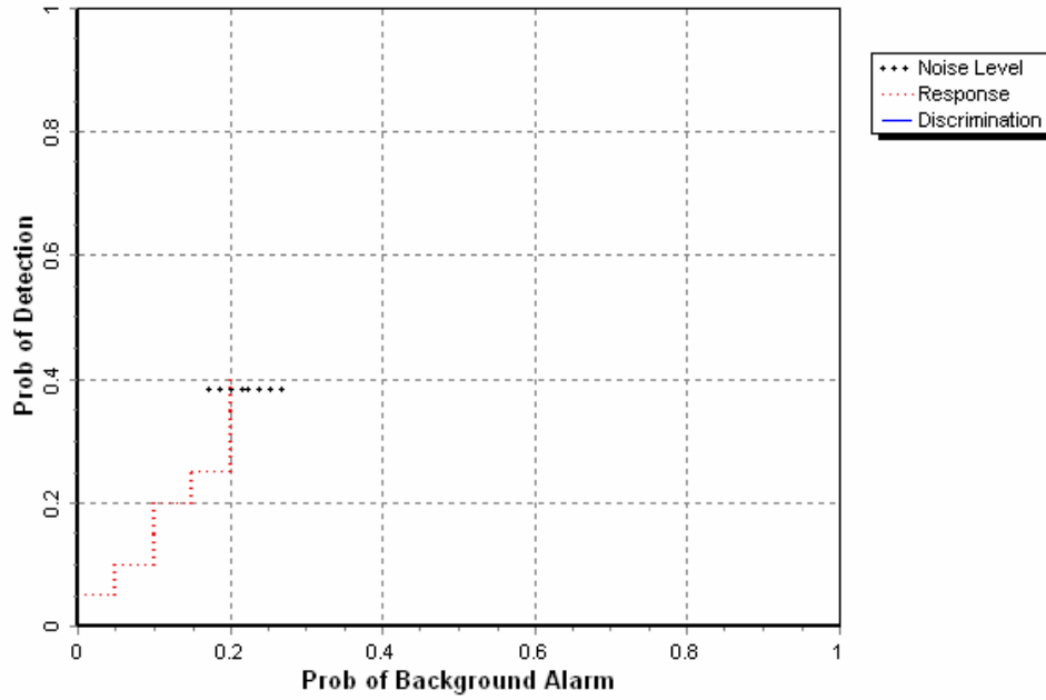
Figure 3. FEREX fluxgate gradient MAG/sling blind grid probability of detection for response and discrimination stages versus their respective probability of background alarm over all ordnance categories combined.
