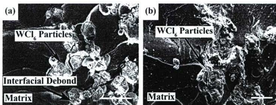
Figure 1.5. SEM images of epoxy fracture surfaces for samples containing as-received WCl_6 (12 wt%). a. Significant interfacial debonding is revealed when no coupling agent is used. b. The addition of 1 wt% silane coupling agent (3-glycidoxypropyltrimethoxysilane) dramatically reduces the amount of interfacial debonding. [scale bars = 50 \mu m]
