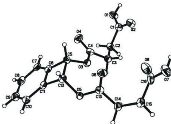
Figure 2.4. ORTEP thermal ellipsoid diagram at the 50% probability for cis -benzocyclobutene linker 2 .
