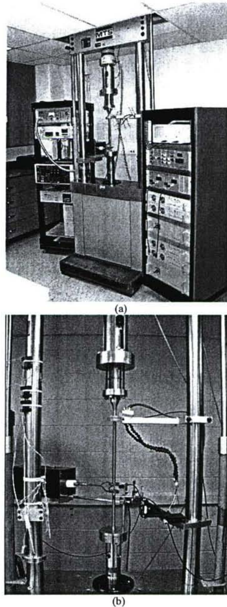
Figure 1: The ultrasonic fatigue testing system capable of testing with superimposed mean stresses at elevated temperature (a) the entire system with the controls and (b) the ultrasonic fatigue load train.
