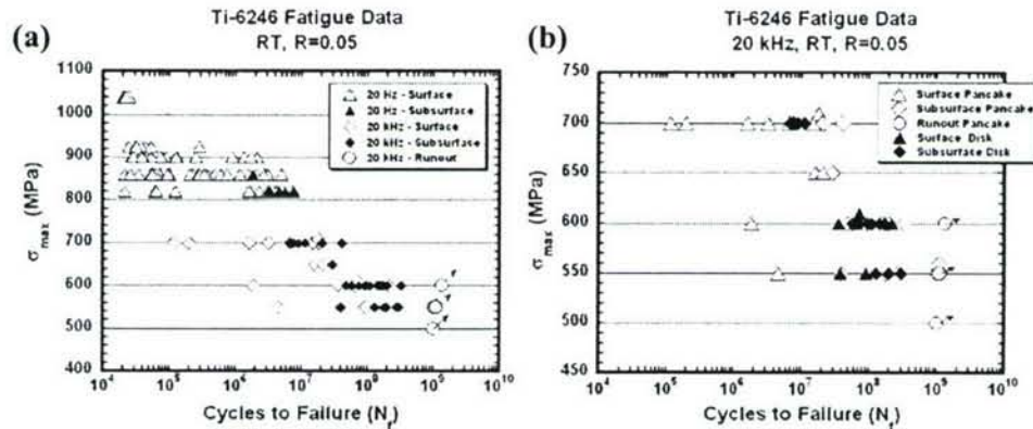
Figure 2. (a) The lifetime data is shown for both heats of material to compare the results from conventional and ultrasonic frequencies. (b) Ultrasonic frequency fatigue data for both forged pancake and retired disk specimens.
