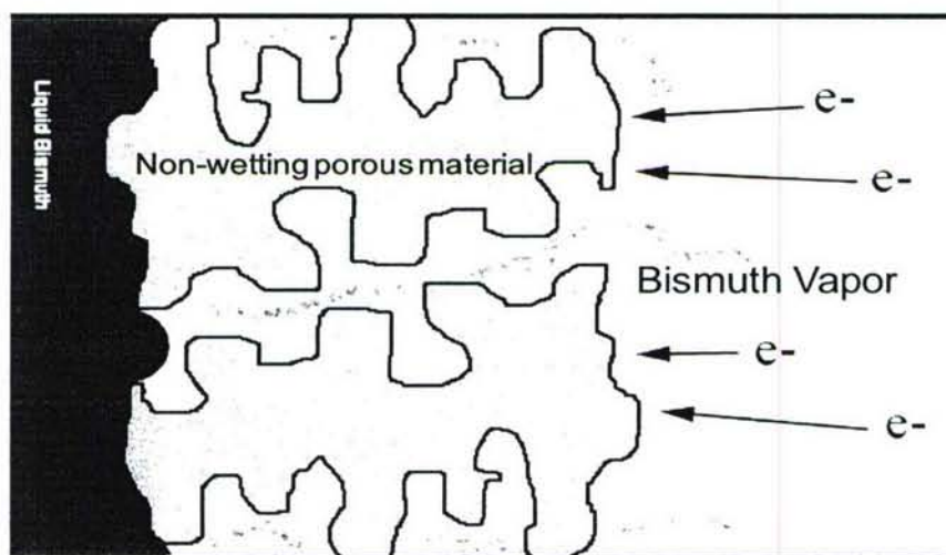
Figure 4-5. Model of liquid bismuth-porous plate interface with electron heating. Surface tension prevents the liquid from flowing through the pore yet gives a free surface for evaporation.
