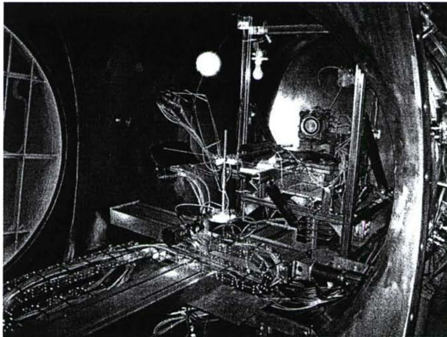
Figure 3-2. Thruster mounted on thrust stand in Xe test facility at the Isp Lab.
