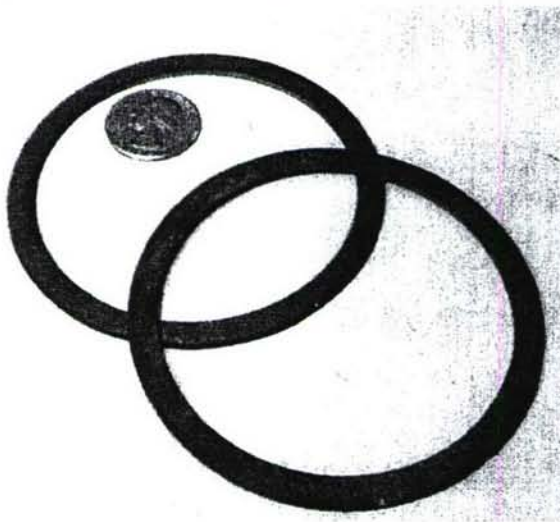
Figure 4-18 – Completed porous molybdenum vaporizer faces ready for electron beam welding.
