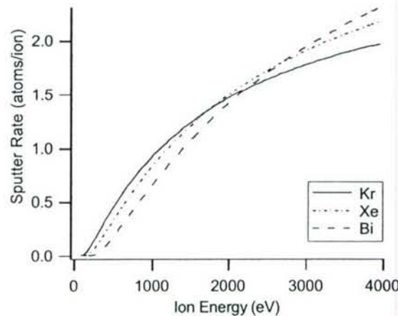
Figure 1-4, Sputter Yield of carbon under bismuth, xenon and krypton ion collisions.
