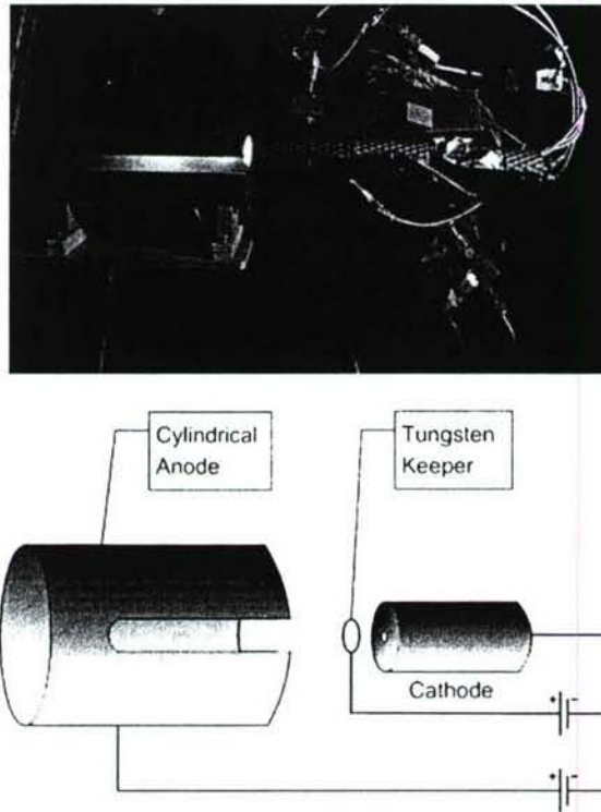
Figure 5-2. Operating bismuth cathode (top) and electrical schematic (bottom).
