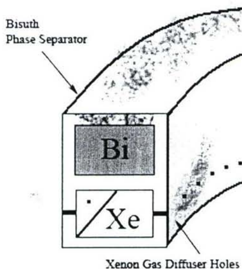
Figure 4-1. Dual-propellant anode cross section. Porous phase discriminator was constructed from stainless-steel.
