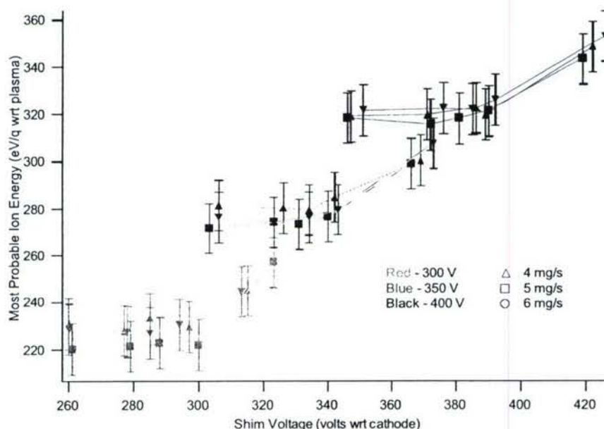
Figure 3-11: Most Probable Ion Energy as a function of all three experimental factors. Higher shim voltage indicates a higher proportion of discharge current on the shims.
