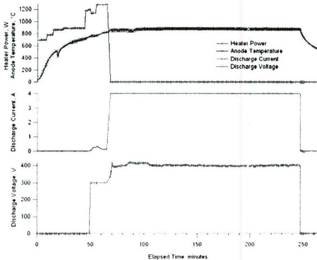
Figure 4-9 – Plot of a typical extended duration testing. After the initial warm up and transient period, steady state operation ensues.
