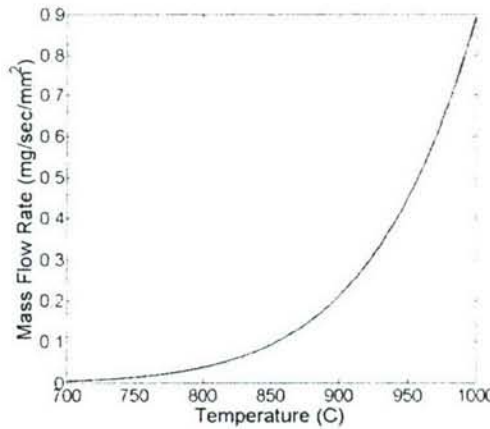
Figure 5-6. Bismuth evaporation rate per surface area as a function of temperature.
