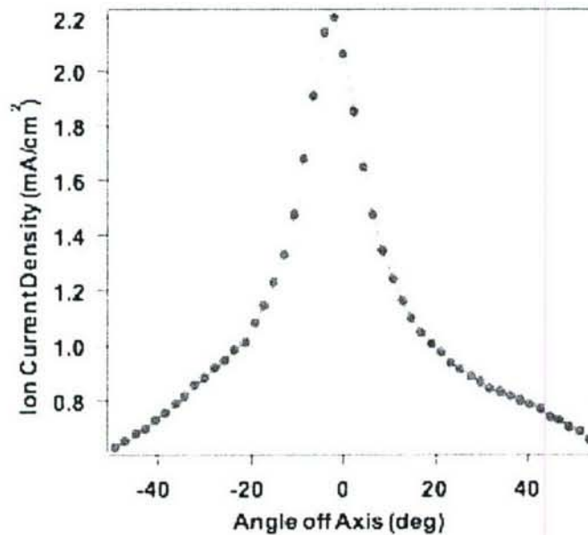
Figure 4-12 – Faraday probe sweep of the exhaust plume taken at 250 mm showing a focused beam.
