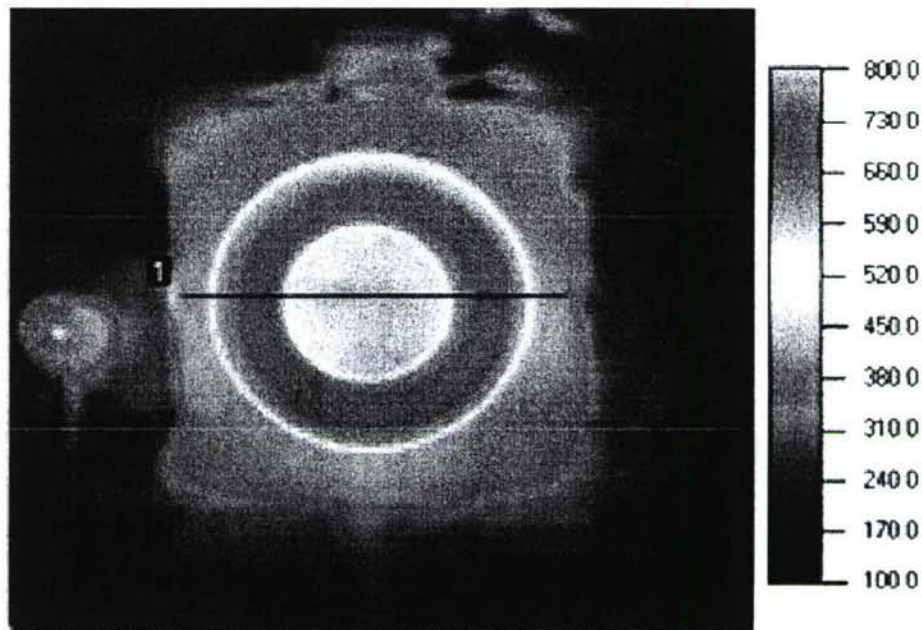
Figure 4-13 – Thermal image of the thruster taken immediately after an extended duration test. Vaporizer face temperature is uniform and the magnetic circuit is below the Curie point.
