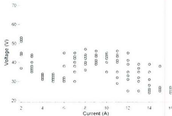
Figure 5-4. Anode voltage taken at currents varying from 2 to 16 Amps at a mass flow rate of 0.71 mg/s using bismuth.
