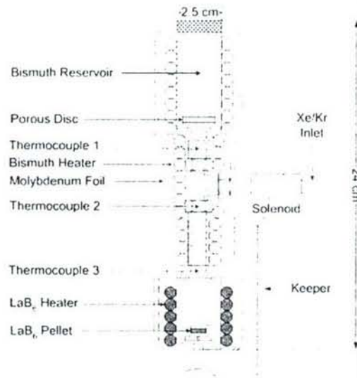
Figure 5-1. Bismuth cathode schematic and thermocouple placement.
