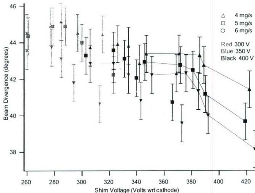
Figure 3-9: Beam divergence as a function of all three experimental factors.
