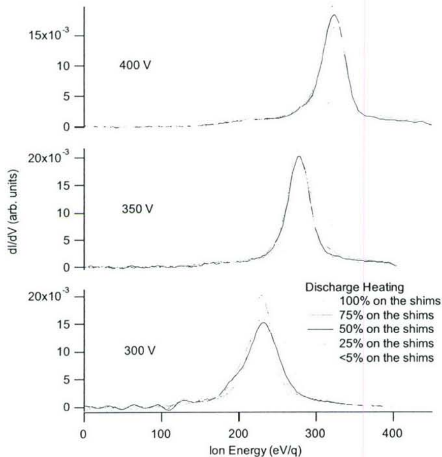
Figure 3-10: Derivatives of RPA current with at 4 mg/s of xenon, at all combinations of anode voltages and shim levels.
