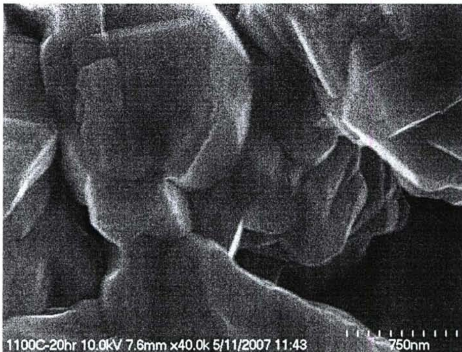
Figure 4-17 - FESEM micrograph of a representative sintered molybdenum disc at 40,000x magnification. The inter-particle grain boundaries are almost indistinguishable from the grains grown on the individual particles. This sample was sintered for 20 hours at 1100°C under high vacuum.
