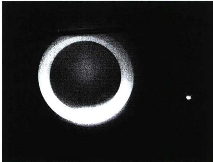
Figure 4-14 – Vaporizer during the early stages of bismuth intrusion into the discharge chamber.
