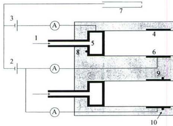
Figure 2-4. Electrical schematic of thruster test apparatus. Numbered annotations are 1: xenon propellant flow (for test with Xe instead of Bi), 2: shim power supply, 3: main anode power supply, 4: outer shim electrode, 5: main anode and gas distributor, 6: inner shim electrode, 7: cathode, 8: anode thermocouple, 9: inner shim thermocouple, and 10: outer shim thermocouple.
