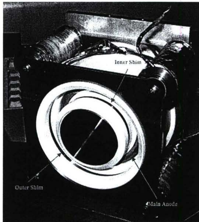
Figure 2-7. Photograph of segmented-anode Hall thruster based on the Aerojet BPT-2000.
