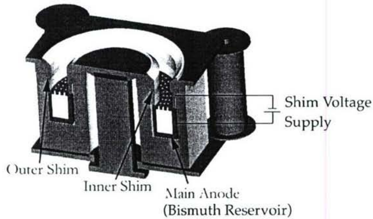
Figure 2-3. Cross section of segmented-anode thruster for direct evaporation of bismuth. The shim electrodes can be used to intercept a fraction of the discharge current and, hence, control the heat deposition to the main anode/bismuth reservoir.
