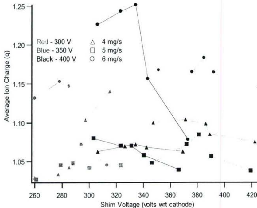
Figure 3-13: Average ion charge as a function of all three experimental factors. High shim voltage for indicates a higher fraction of discharge current heating on the shims.
