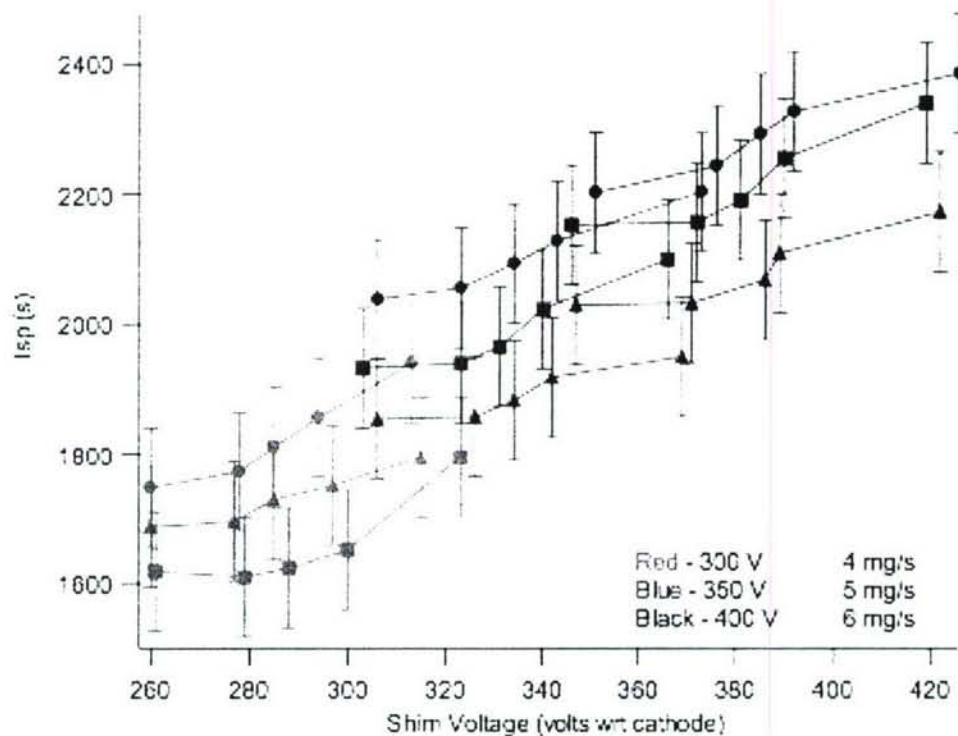
Figure 3-6: Specific Impulse as a function of shim voltage for all thruster operating conditions tested. Higher shim voltage for a given anode voltage indicates higher discharge electron heating on the shims.
