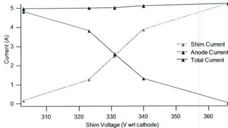
Figure 3-4: Characteristic shift in current on the shims and main anode as shim voltage was varied. Thruster was operating at 350 V on the anode and 5 mg/s of mass flow.
