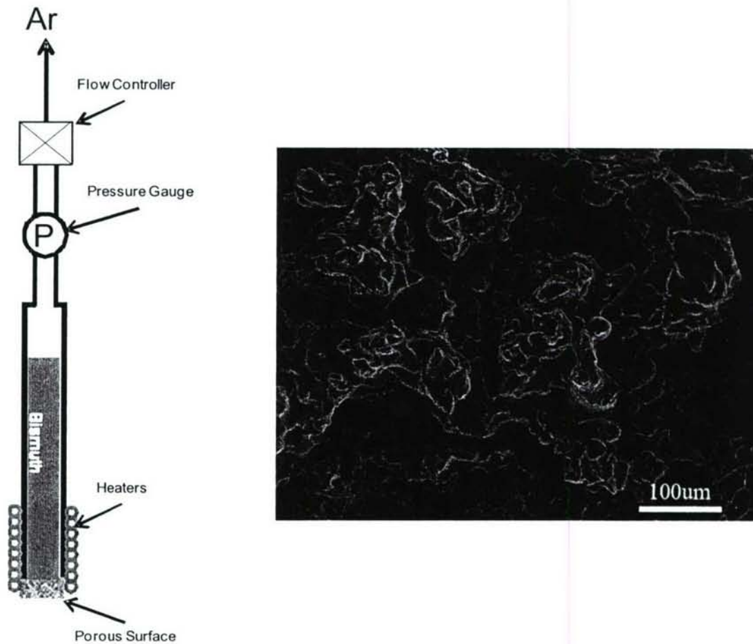
Figure 4-6. Extrusion test set-up (left). Electron micrograph of a 10-mm commercially sintered stainless-steel plate showing the statistical variation of pore size (right).
