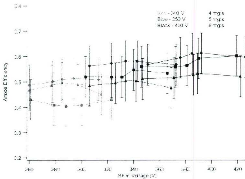
Figure 3-7: Thruster Efficiency as a function of all three experimental factors. Higher shim voltage for a given anode voltage indicates higher discharge heating on the shims.
