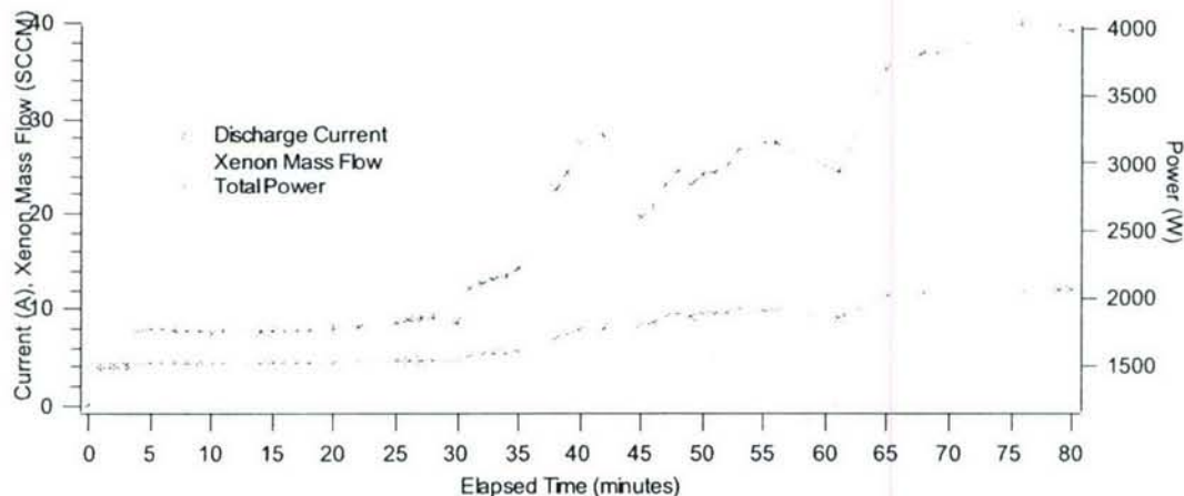
Figure 4-2. Current, power, and Xe flow rate during a “jump start” from Xe to Bi operation.
