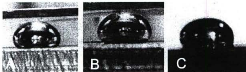
Figure 4-4. Bismuth wetting tests on stainless steel (A), molybdenum (B) and tungsten (C) substrates. In all cases the contact angle exceeds 90^\circ therefore bismuth is non-wetting on these materials.
