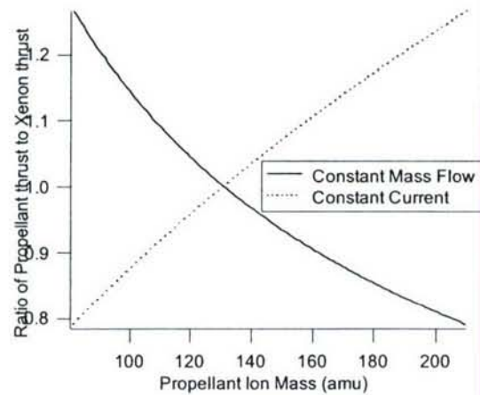
Figure 1-1. Change in thrust as a function of propellant ion mass, assuming constant acceleration voltage.
