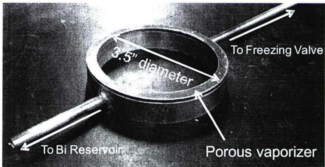
Figure 4-7. Photo of an anode laying vaporizer-side up.
