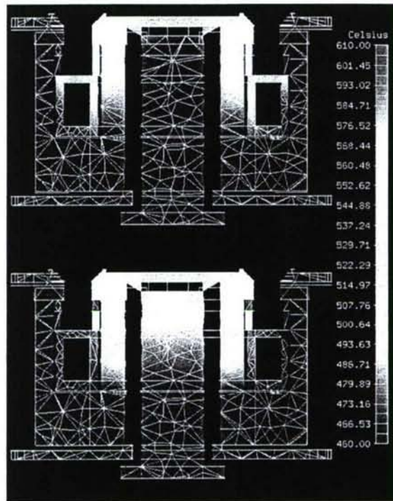
Figure 2-6. Thermal simulation of segmented anode thruster. In the top figure, 100% of the discharge current is attached to the main anode. In the bottom, all of the current is intercepted by the inner shim electrode.
