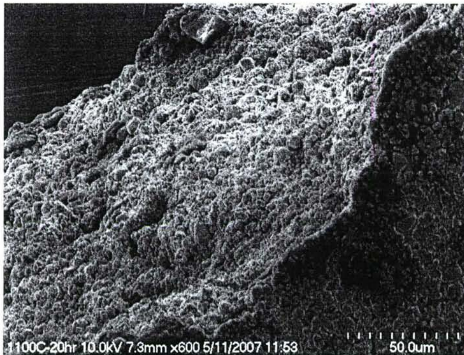
Figure 4-15 – FESEM micrograph at 600x showing some of the bulk features of the sintered molybdenum. This sample was sintered for 20 hours at 1100°C under high vacuum.
