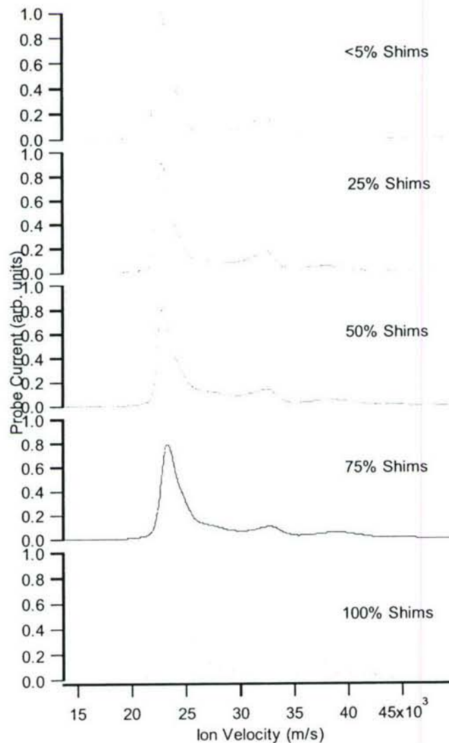
Figure 3-12: typical set of ExB probe traces taken as the level of shim current was varied. Data are for 400 V on the anode and 4 mg/s of xenon.
