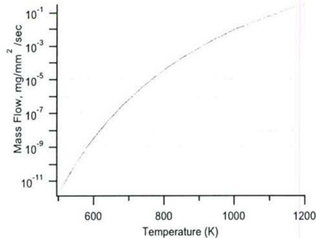
Figure 2-5. Calculated Bi evaporation rate as a function of temperature.
