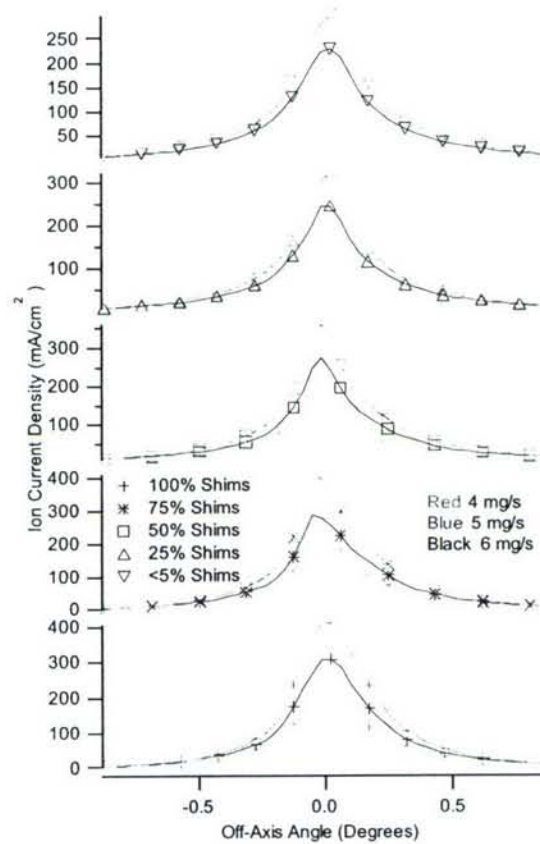
Figure 3-8: Beam Profiles with 350 V on the anode at all mass flows and levels of discharge current heating.
