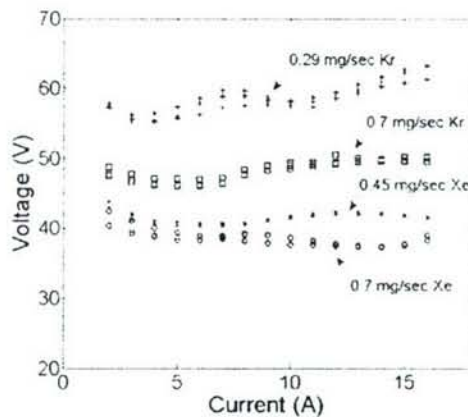
Figure 5-5. Anode voltage taken at currents varying from 2 to 16 amps using krypton and xenon propellants.
