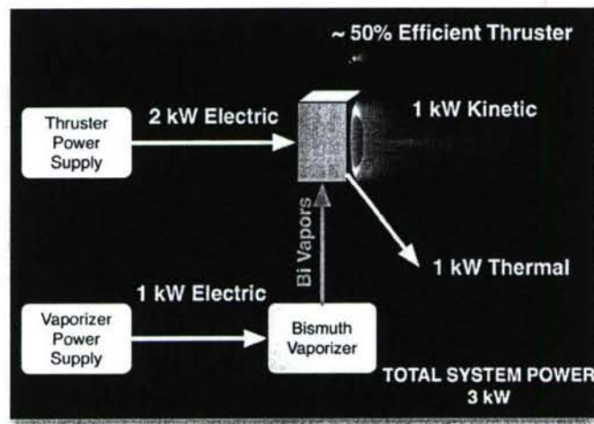
Figure 2-1. System power for an externally heated bismuth supply system.
