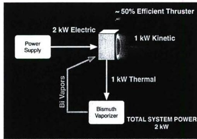
Figure 2-2. MTU-patented energy harvesting scheme to use plasma discharge waste heat from electron attachment to the anode for bismuth evaporation.
