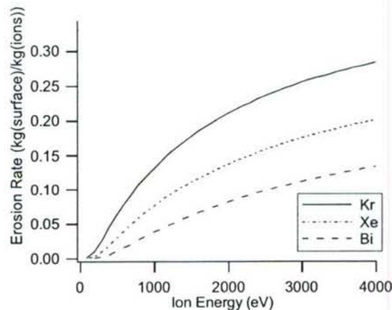
Figure 1-5. Erosion Rate of Carbon per kilogram of bismuth, xenon, and krypton ions.
