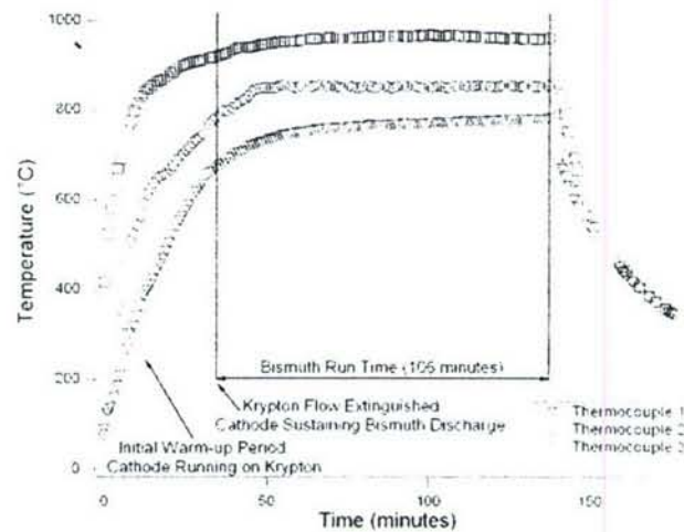
Figure 5-3. Temperature data taken near the bismuth reservoir, the cathode center, and the end orifice by thermocouples 1, 2, and 3, respectively, throughout the duration of the bismuth cathode test.
