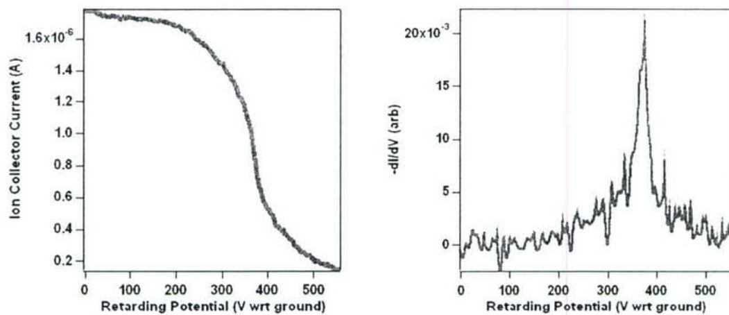
Figure 4-11 – RPA data taken at 500 mm down stream of the thruster exit plane on centerline. The expected energy of the exhausted ions is approximately 360 volts.
