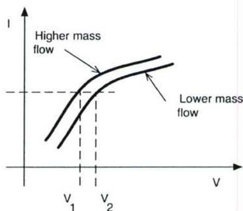
Figure 4-10 – I-V characteristics for typical HET at different mass flow rates illustrating how discharge voltage compensates for varying mass flows.
