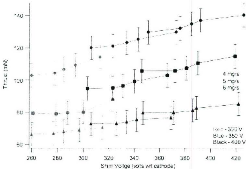
Figure 3-5: Thrust measured as a function of all three experimental factors. Higher shim voltages for a given mass flow and anode voltage combination correspond to higher discharge heating acceptance by the shims.
