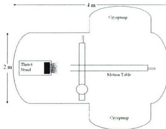
Figure 3-1. Top view of Xe test facility.
