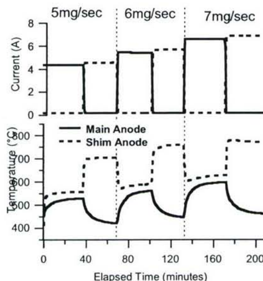
Figure 3-3. Thermal response of the segmented-anode Hall thruster with 400 V on the main anode. Temperature uncertainty is approximately 1%.
