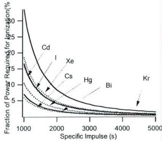
Figure 1-2. Fraction of thruster power required for ionization vs. I_{sp} for all propellants examined.
