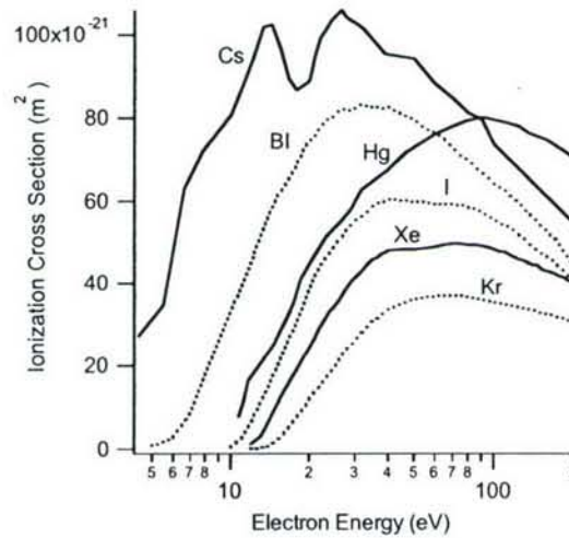
Figure 1-3. Electron-Impact Ionization Cross Sections for bismuth 26 , cesium 27 , iodine 28 , krypton 30 , mercury 31 , and xenon 30 between threshold and 200 eV.
