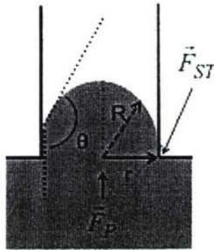
Figure 4-3. Balance of forces in response to a non-wetting fluid interacting with a capillary.
