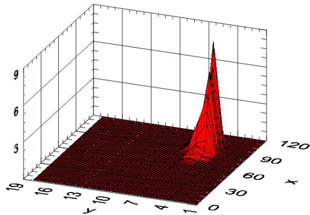
Figure 8. Normalized Cumulative Damage Plot for SG2 versus Frequency 1/3 Octave Band Number (Y) versus X
