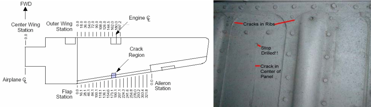
Figure 1. Crack Location on C-130 Secondary Structure
