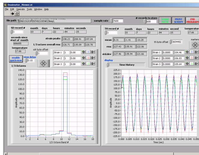
Figure 2. Typical Sine Wave Data –SN01-10 Oct 02
