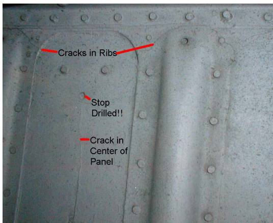
Figure 1. Cracks on Secondary Aircraft
