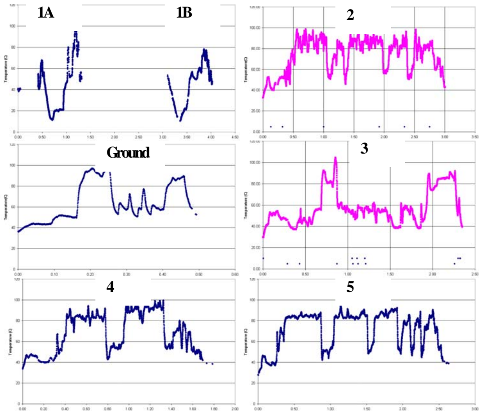
Figure 5. Temperature ( ^{\circ}\text{C} ) versus Time (Hours) for Each Flight
