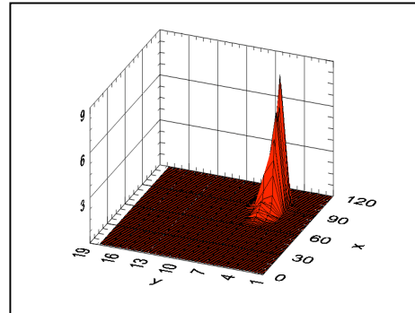
Figure 8. Normalized cumulative damage plot for SG2 versus frequency 1/3 octave band number (Y) versus temperature °C (X).
