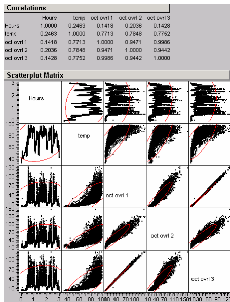
Figure 7. Flight 2 Correlations Between Temperature and Strains
