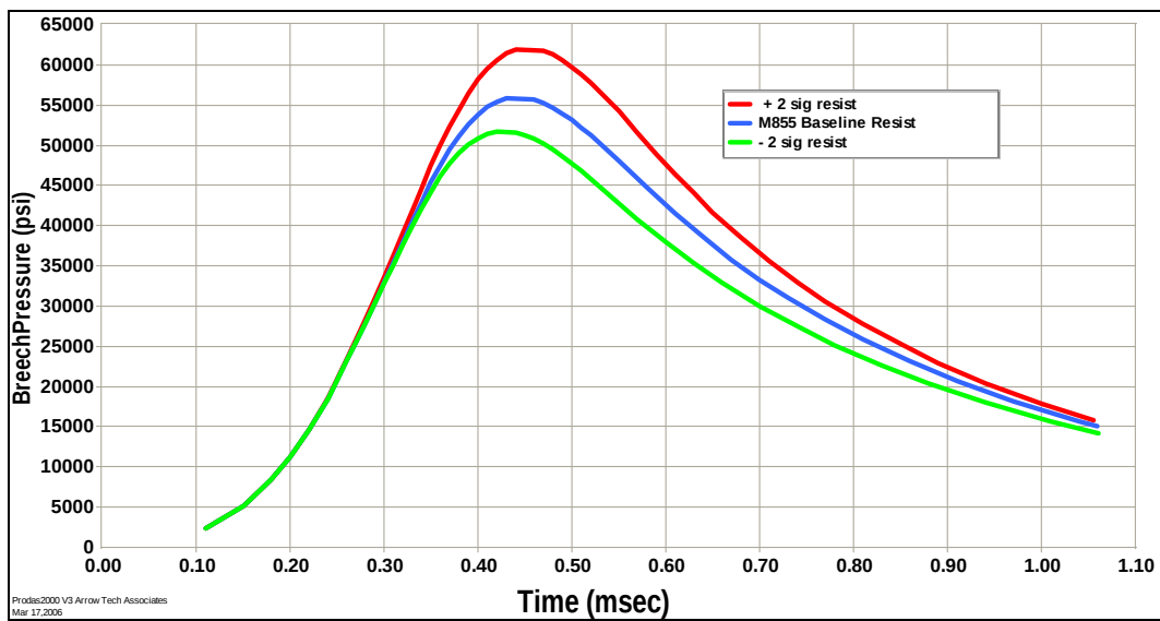
Figure 16. Predicted pressure vs. time for M855 bullets with varying resistance pressures.
