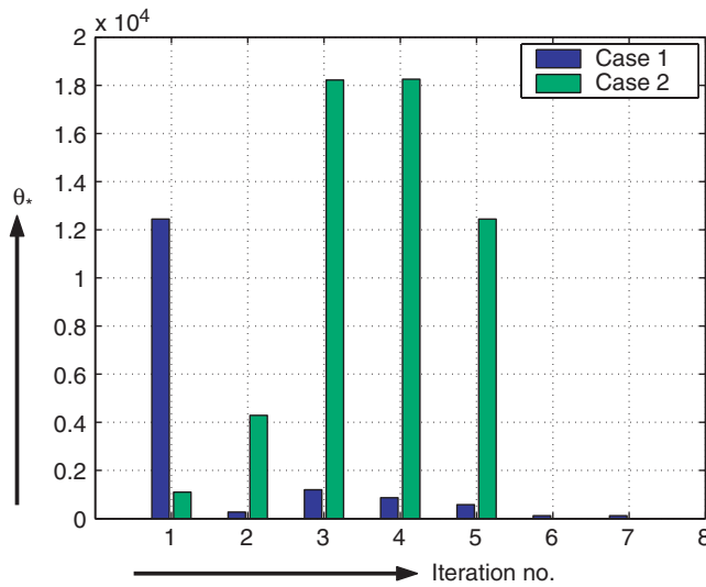
Figure 7. Computed \theta_i for each iteration.
