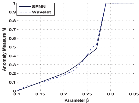
Fig. 11. Anomaly detection on the electronic system apparatus.
